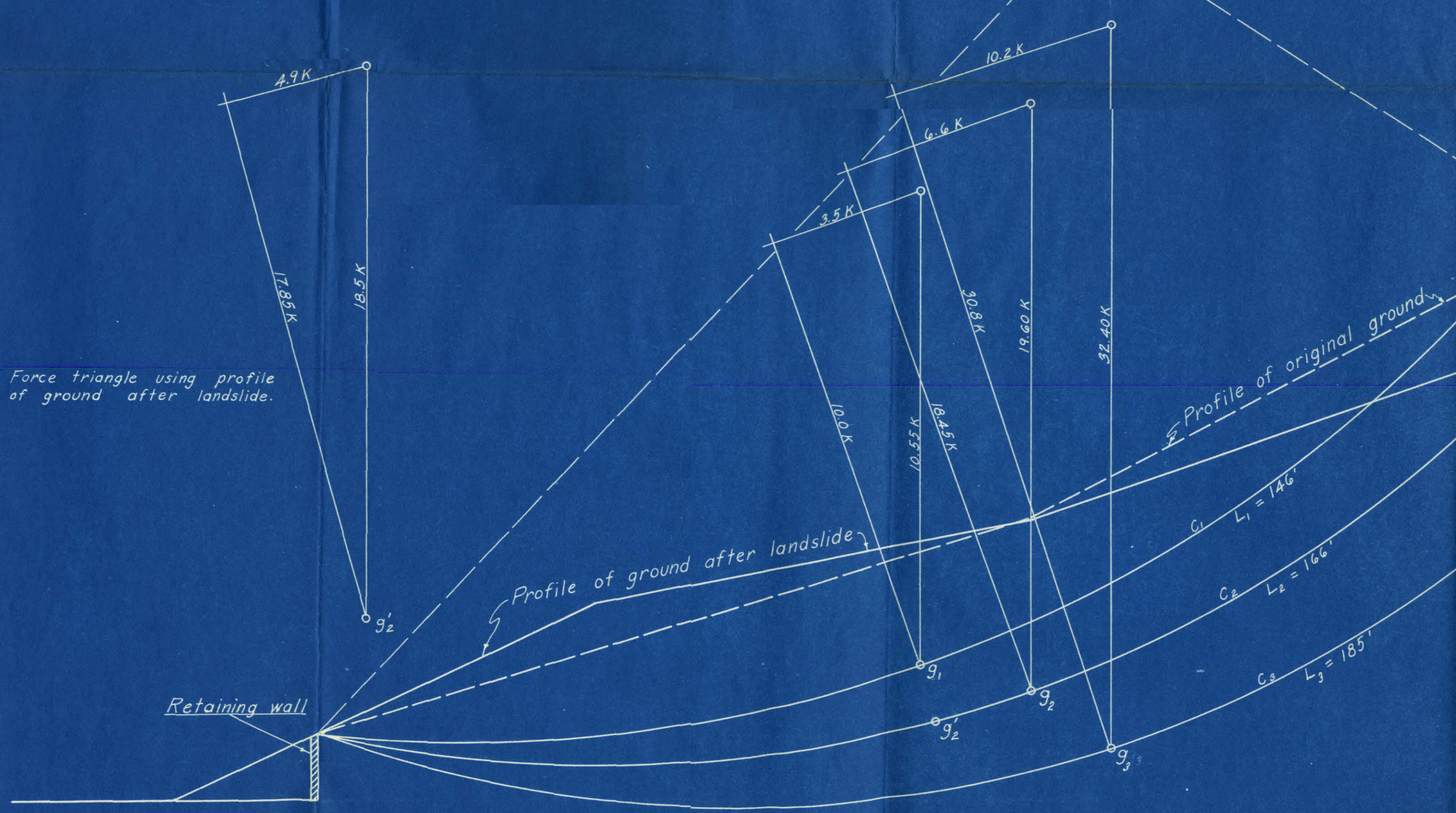
Figure 25. Graphical Determination of Coefficients of Cohesion and Friction for Cross-Section Through Landslide "A" Along Turk Street Lone Mountain - San Francisco Scales { Linear : 1 inch = 10 feet Force : 1 inch = 2K, 3K, 4K Drawn and Calculated by William M. Cogen June 1936
