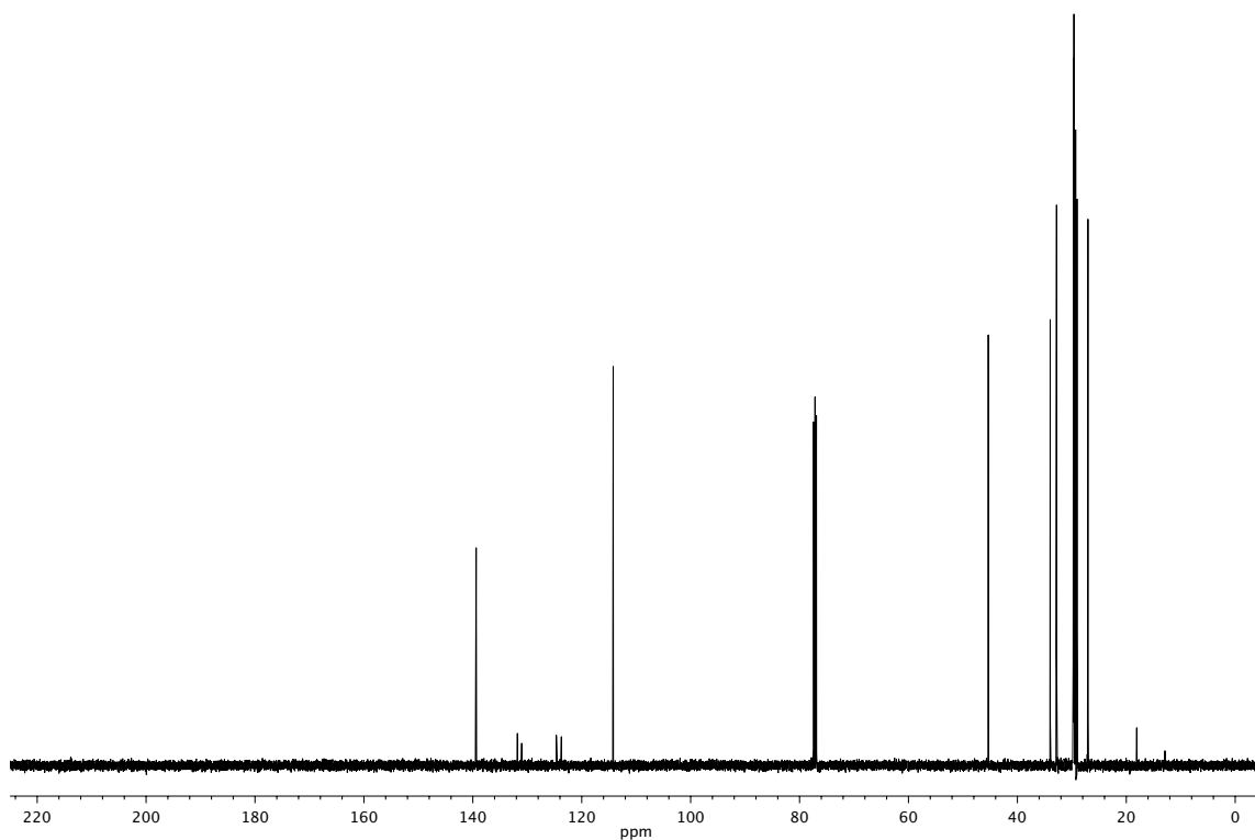
Figure A5.16 13 C NMR (126 MHz, CDCl 3 ) of compound 129h .
