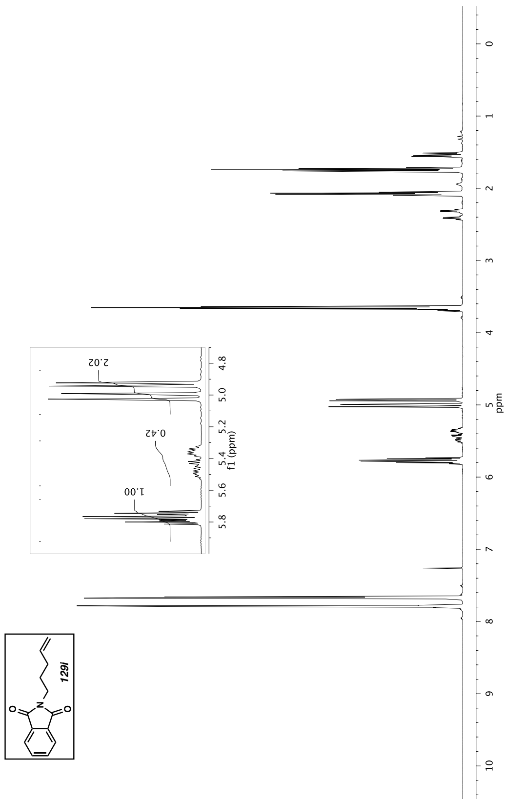
Figure A5.17 ^1\text{H} NMR (500 MHz, \text{CDCl}_3 ) of compound 129i .
