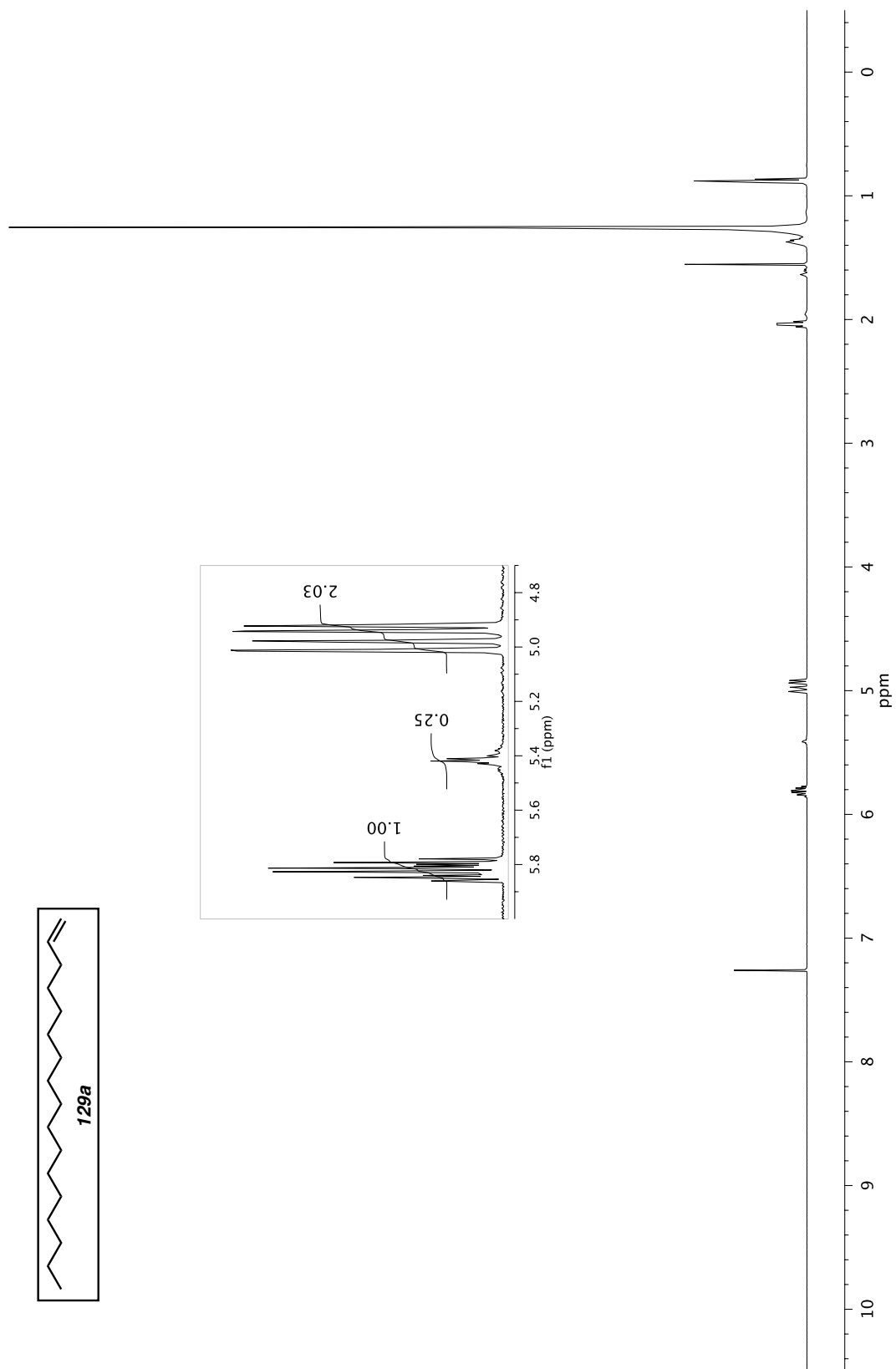
Figure A5.7 ^1\text{H} NMR (500 MHz, \text{CDCl}_3 ) of compound 129a .
