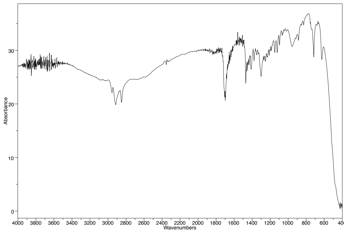
Figure A5.5 Infrared spectrum (Thin Film, NaCl) of compound 128o .
