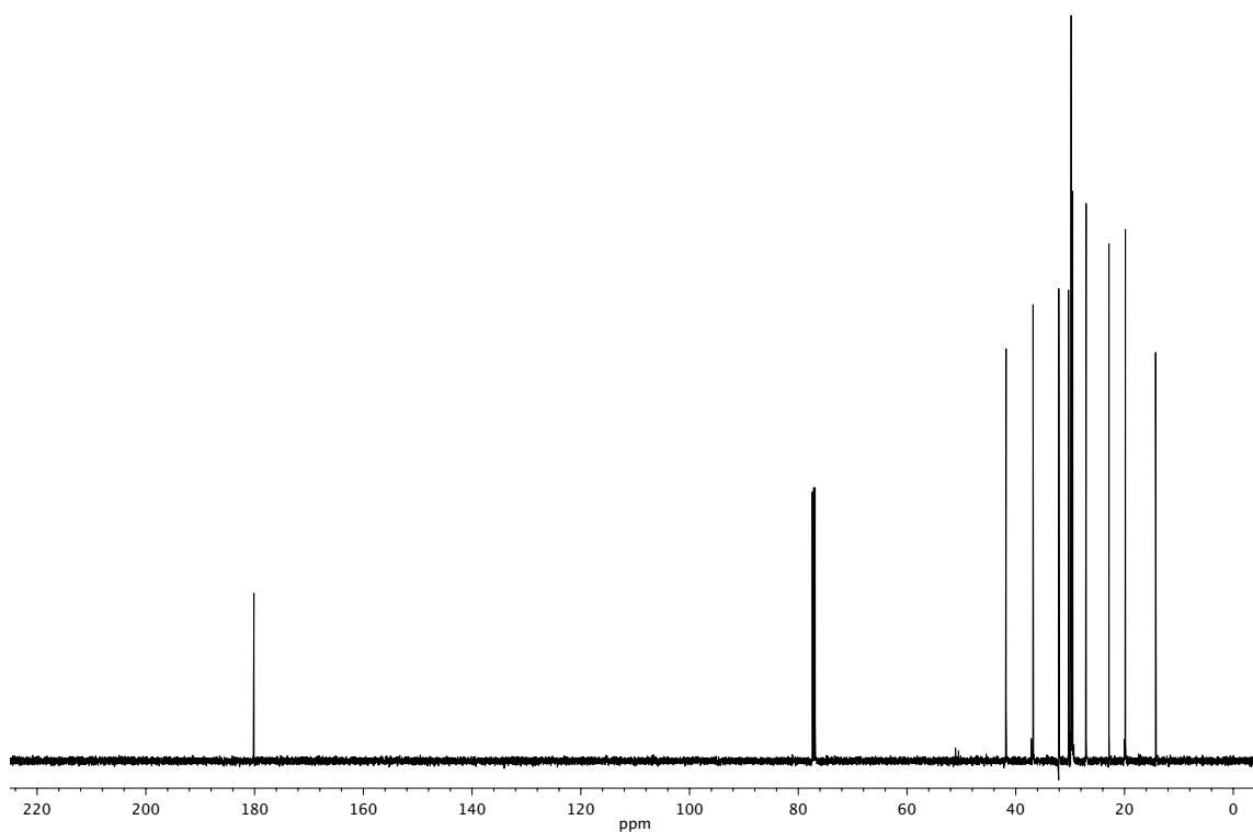
Figure A5.6 13 C NMR (126 MHz, CDCl 3 ) of compound 128o .
