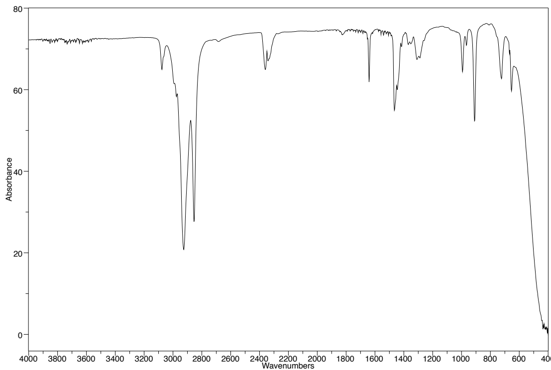
Figure A5.15 Infrared spectrum (Thin Film, NaCl) of compound 129h .
