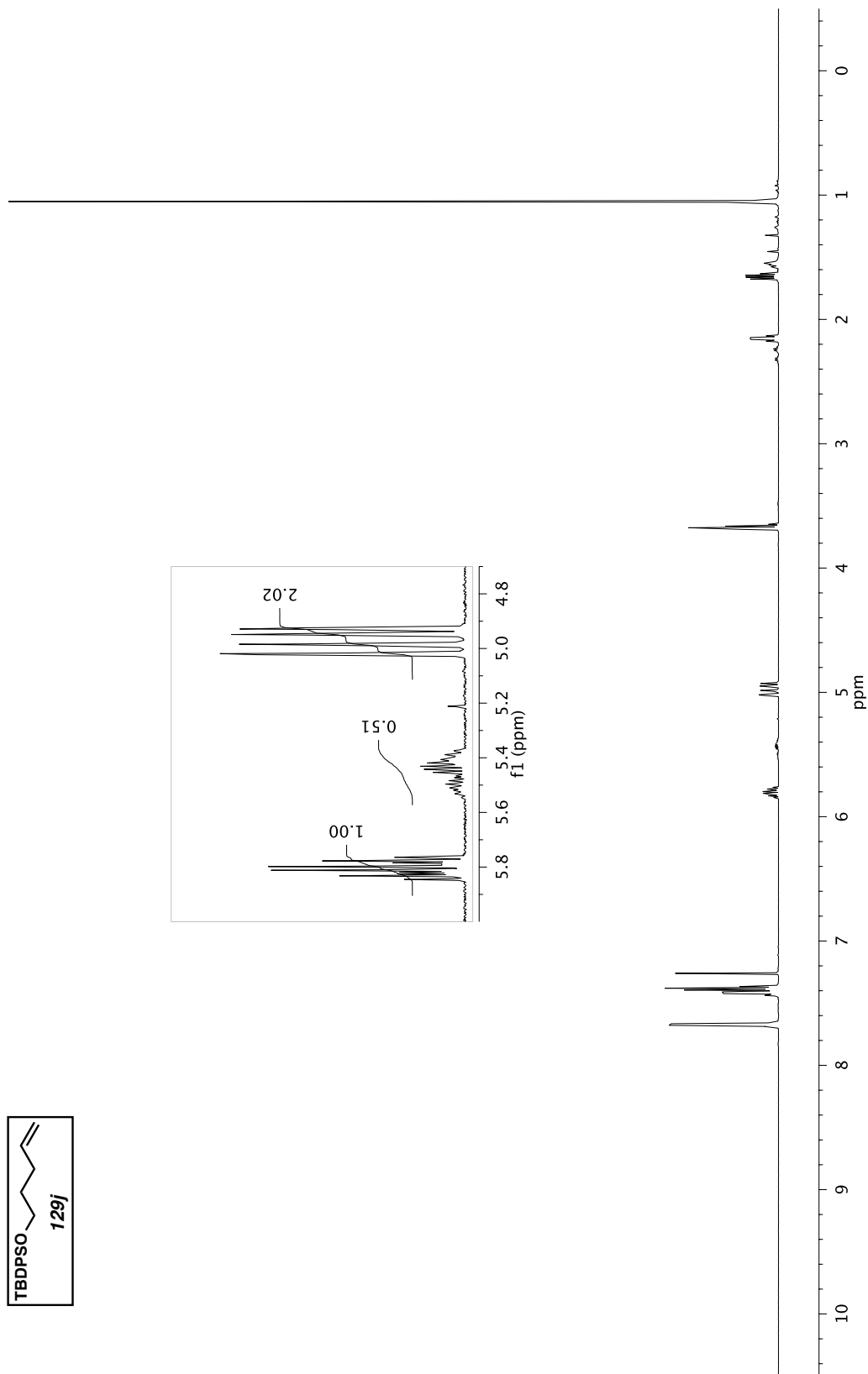
Figure A5.18 ^1\text{H} NMR (500 MHz, \text{CDCl}_3 ) of compound 129j.
