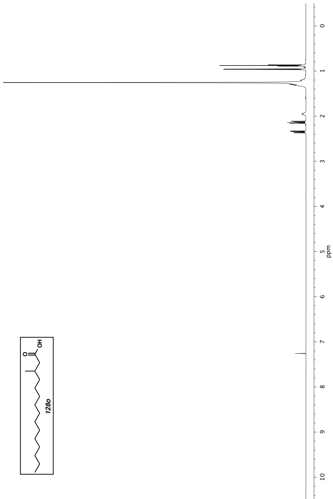
Figure A5.4 ^1\text{H} NMR (500 MHz, \text{CDCl}_3 ) of compound 1280.
