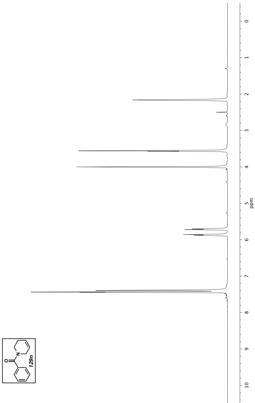
Figure A5.22 ^1\text{H} NMR (500 MHz, \text{DMSO-d}_6 , 130\text{ }^\circ\text{C} ) of compound 129n .
