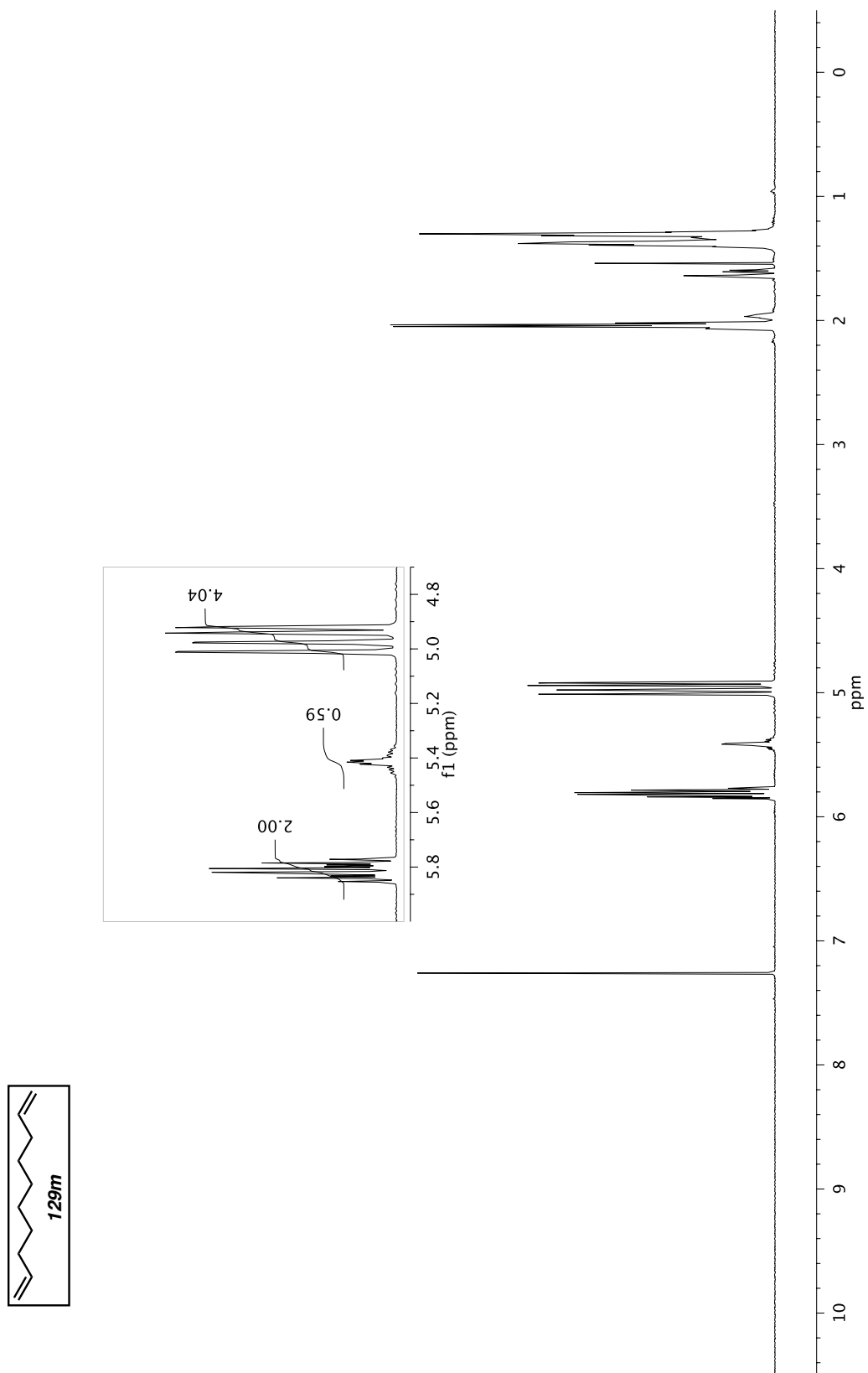
Figure A5.21 ^1\text{H} NMR (500 MHz, \text{CDCl}_3 ) of compound 129m .
