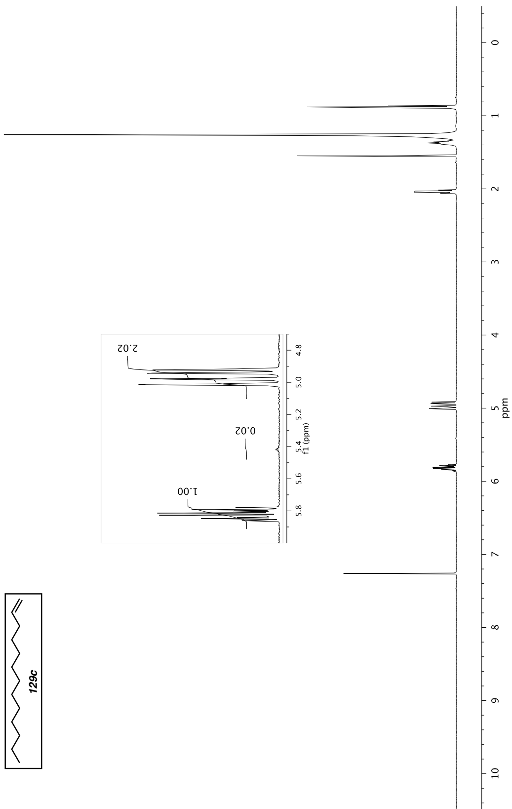
Figure A5.9 ^1\text{H} NMR (500 MHz, \text{CDCl}_3 ) of compound 129c .
