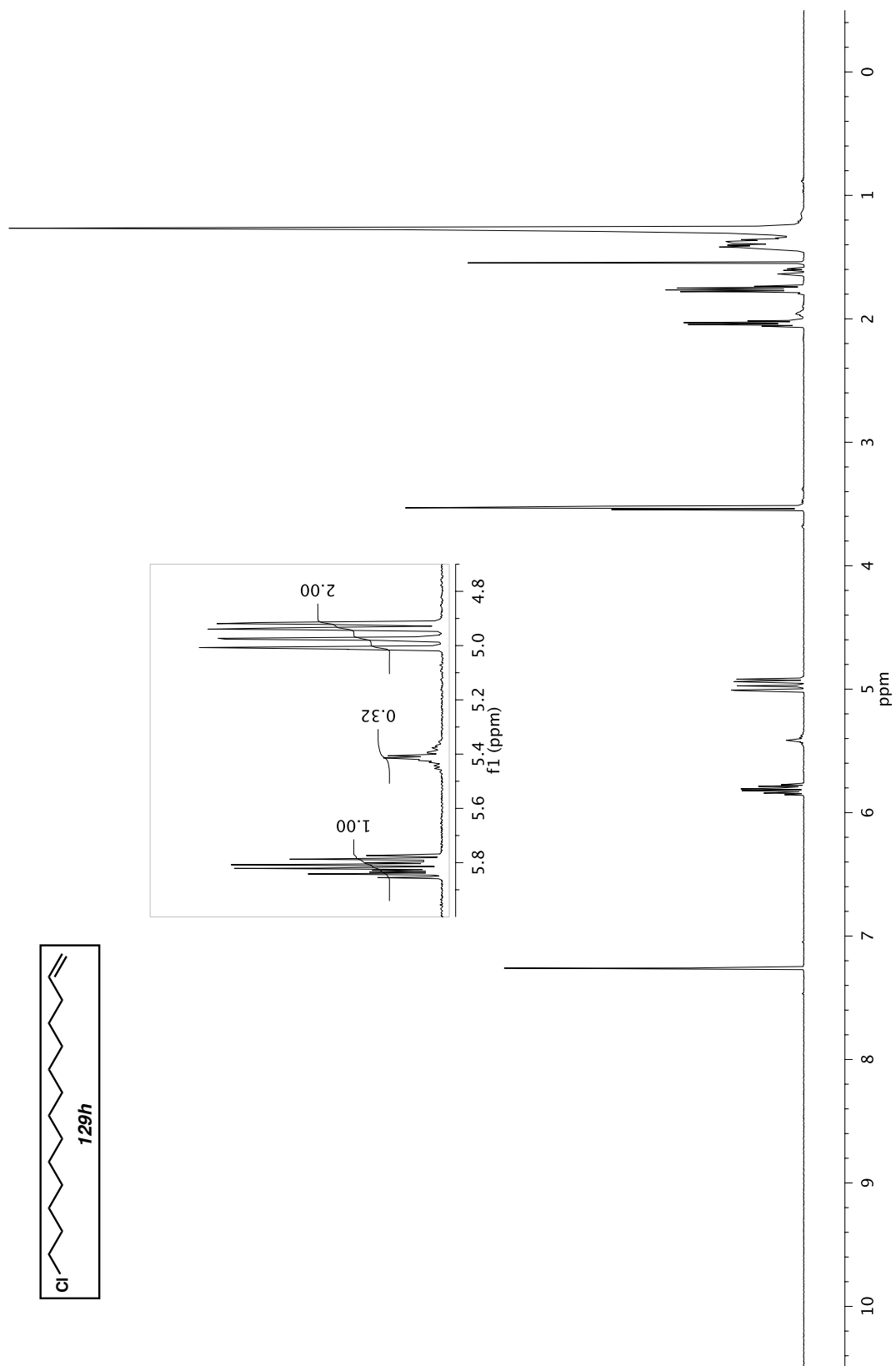
Figure A5.14 ^1\text{H} NMR (500 MHz, \text{CDCl}_3 ) of compound 129h .
