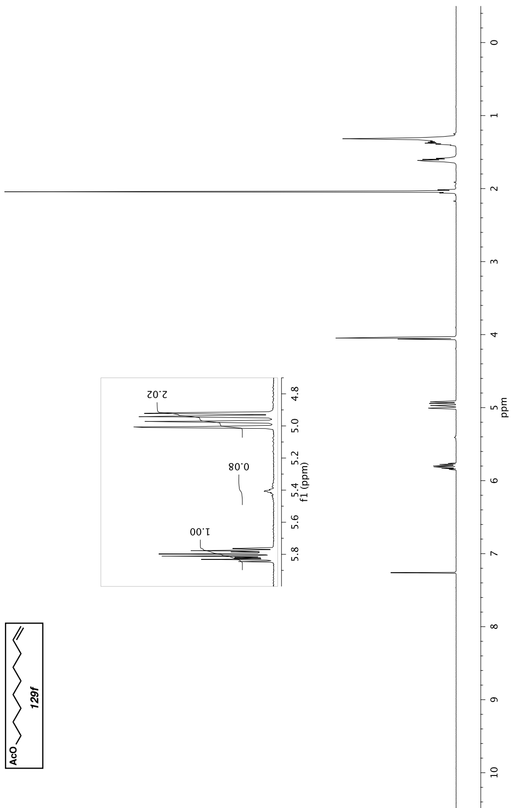
Figure A5.12 ^1\text{H} NMR (500 MHz, \text{CDCl}_3 ) of compound 129f .
