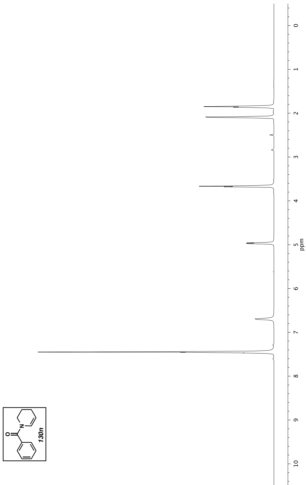
Figure A5.23 ^1\text{H} NMR (500 MHz, \text{DMSO-d}_6 , 130\text{ }^\circ\text{C} ) of compound 130n .
