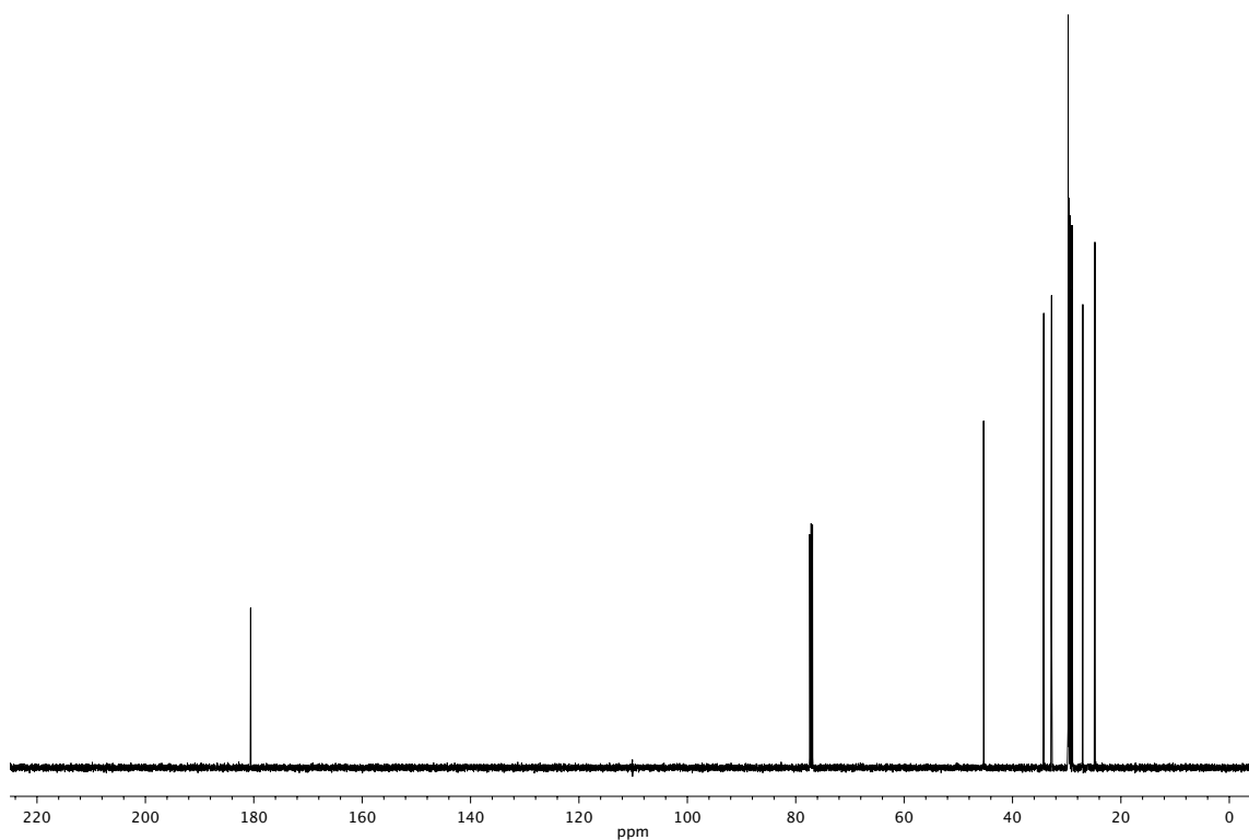
Figure A5.3 13 C NMR (126 MHz, CDCl 3 ) of compound 128h .
