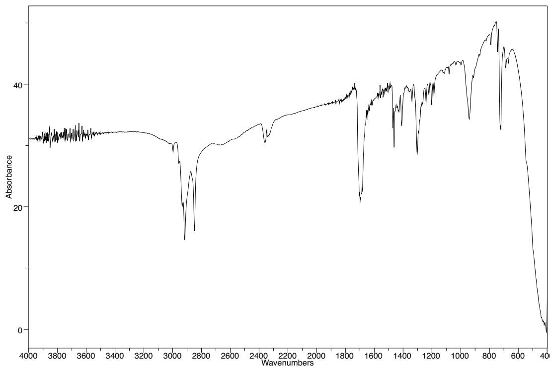
Figure A5.2 Infrared spectrum (Thin Film, NaCl) of compound 128h .
