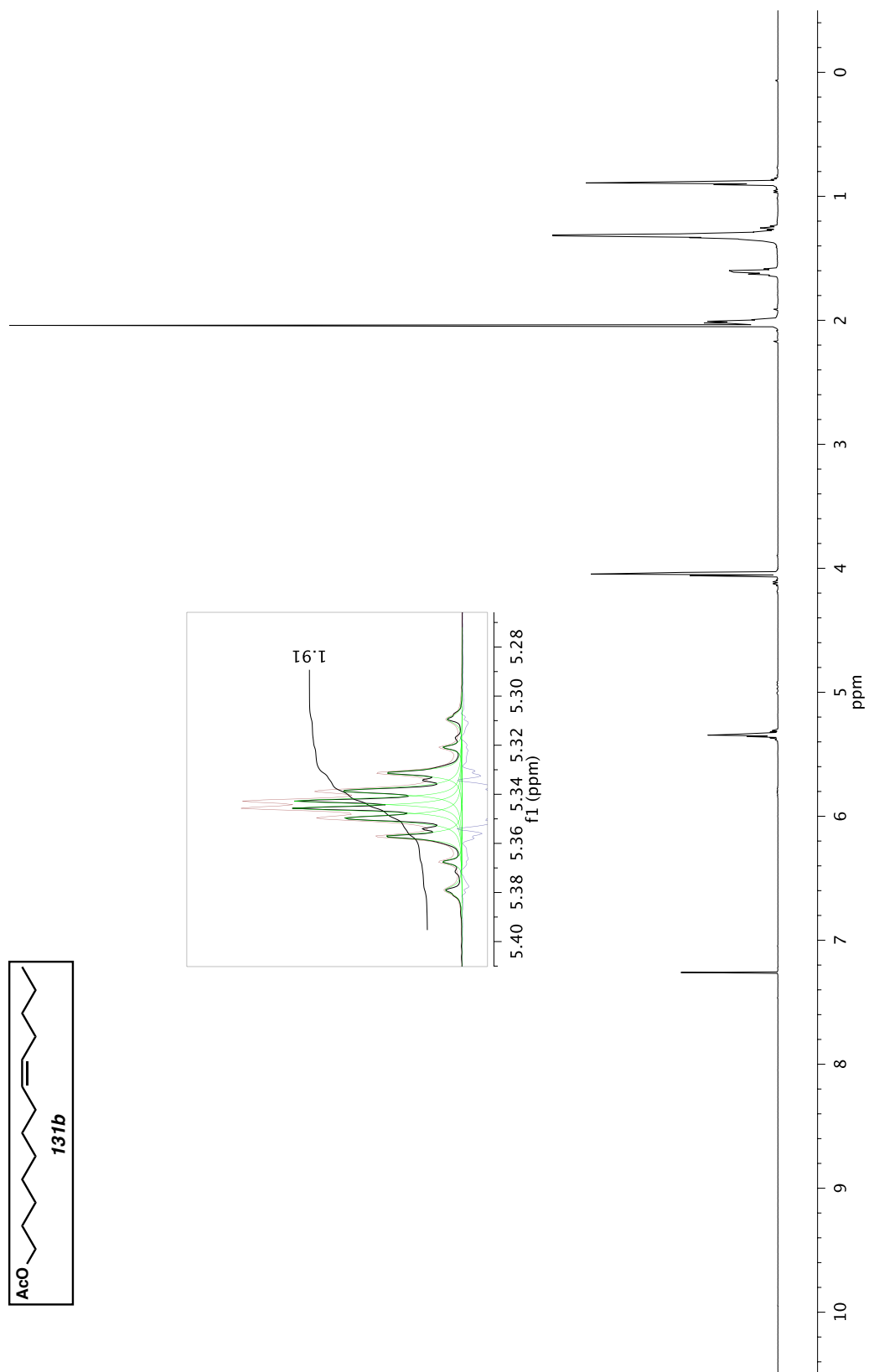
Figure A5.27 ^1\text{H} NMR (500 MHz, \text{CDCl}_3 ) of compound 131b .
