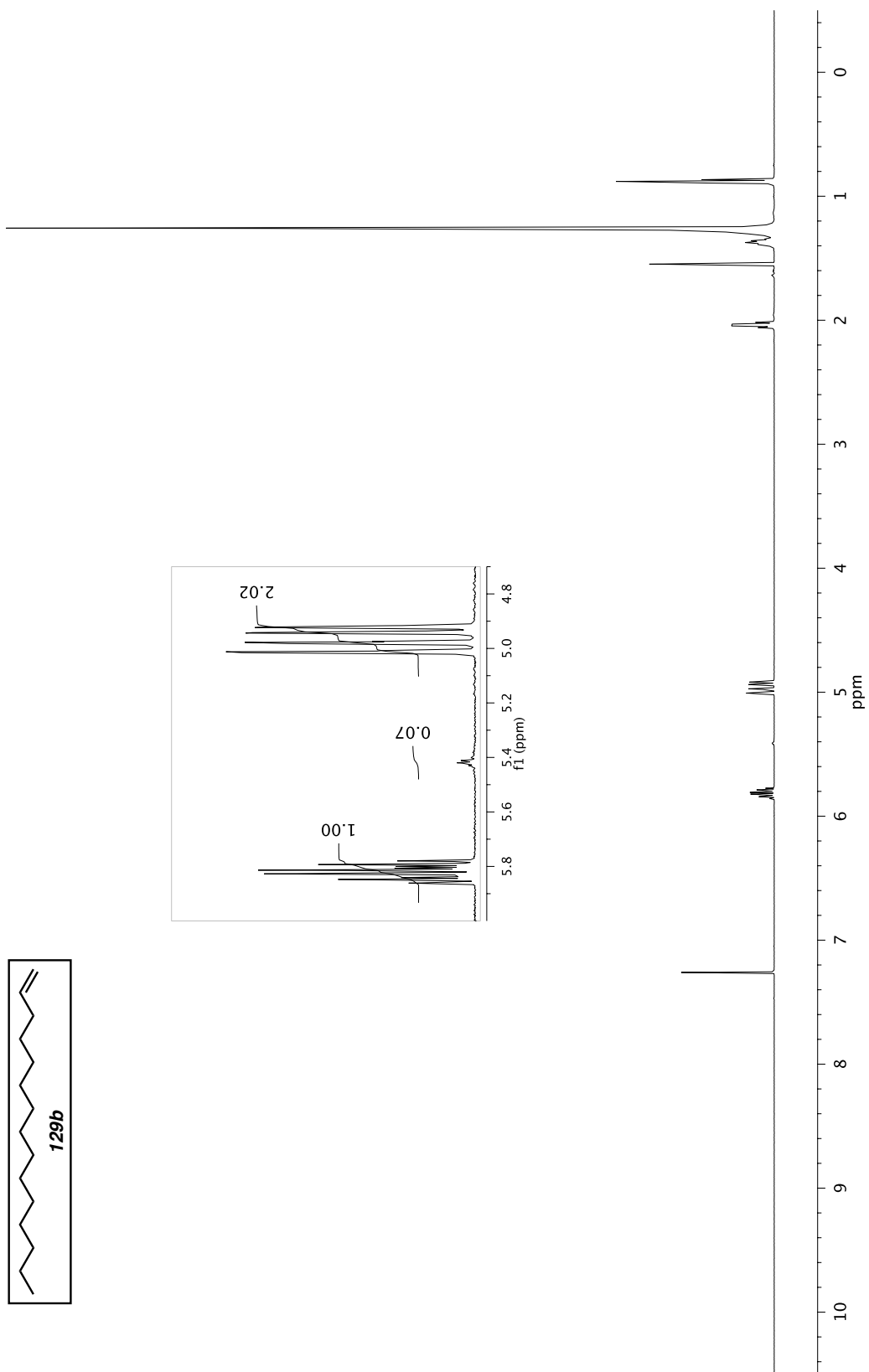
Figure A5.8 ^1\text{H} NMR (500 MHz, \text{CDCl}_3 ) of compound 129b .
