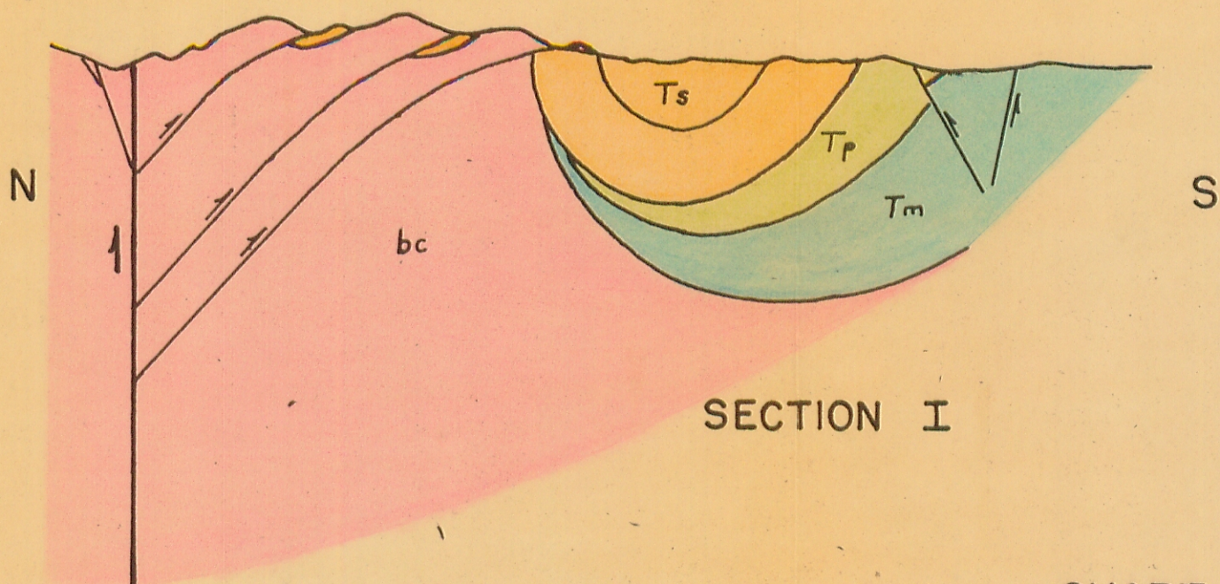
CHART II SEQUENCE OF STEPS IN THE DETERMINATION OF THE PRE-FAULTING GEOLOGIC STRUCTURE
