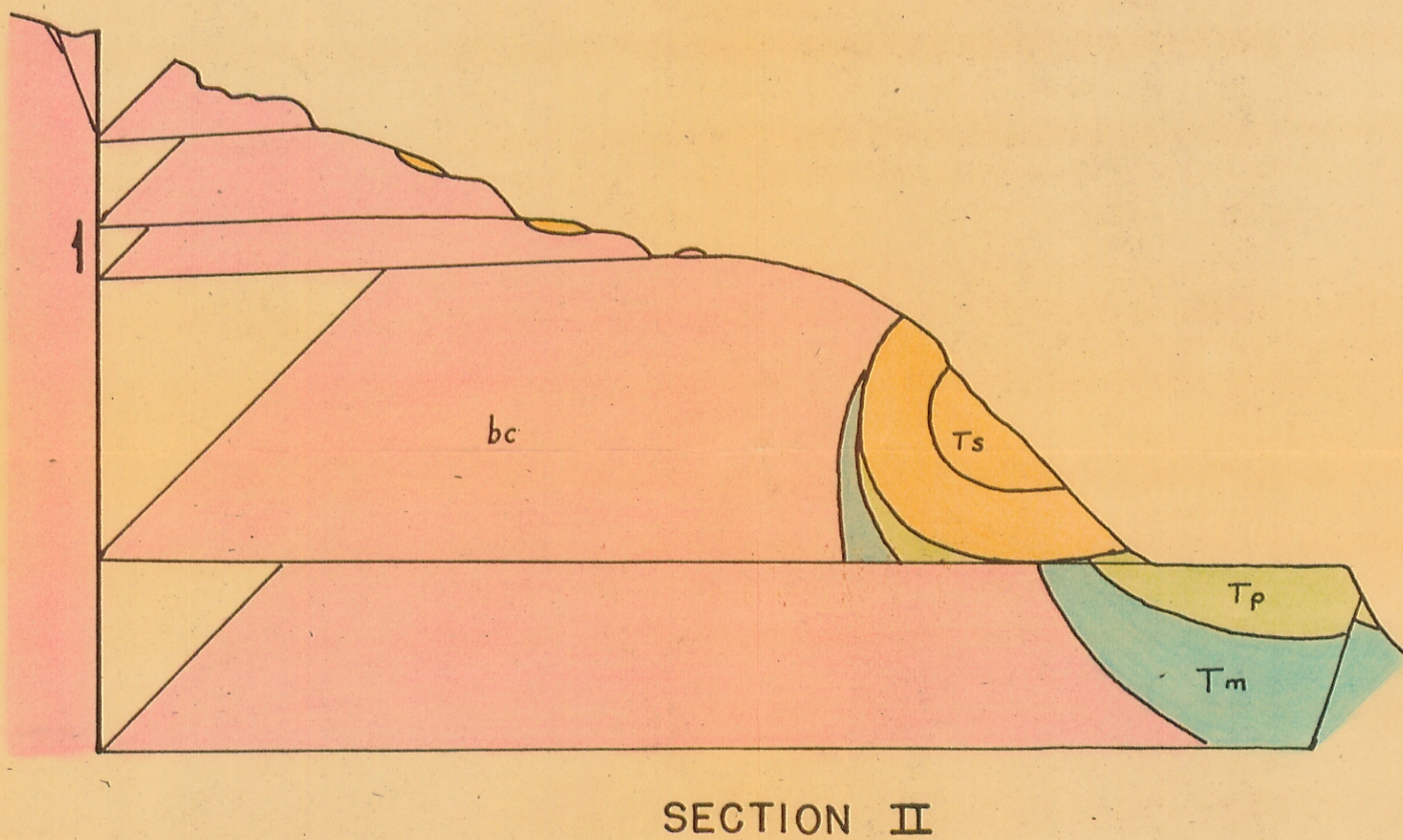
CHART II SEQUENCE OF STEPS IN THE DETERMINATION OF THE PRE-FAULTING GEOLOGIC STRUCTURE
