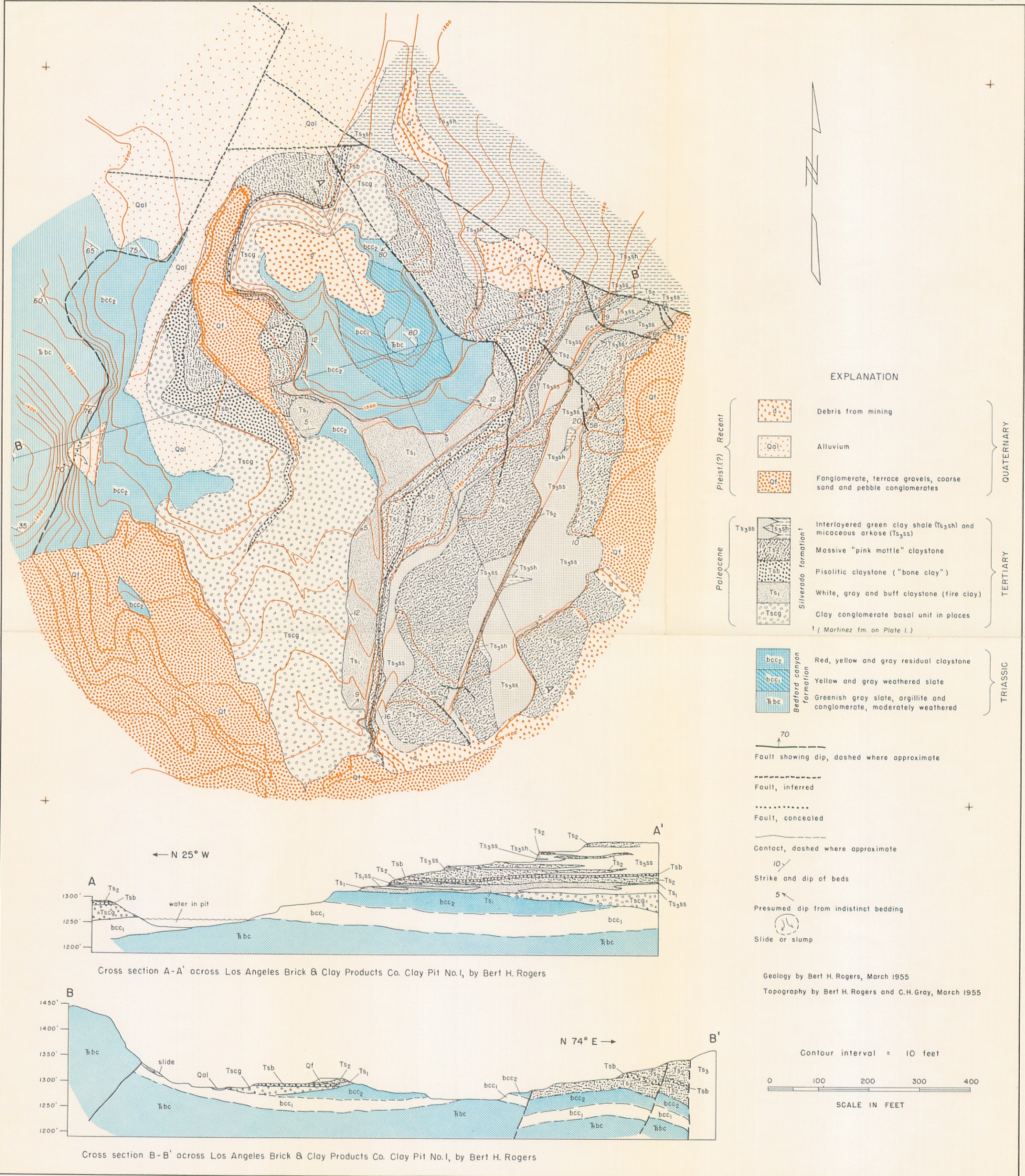
GEOLOGIC MAP AND SECTIONS OF LOS ANGELES BRICK AND CLAY PRODUCTS COMPANY NO. 1 CLAY PIT, ALBERHILL, RIVERSIDE CO., CALIF.
