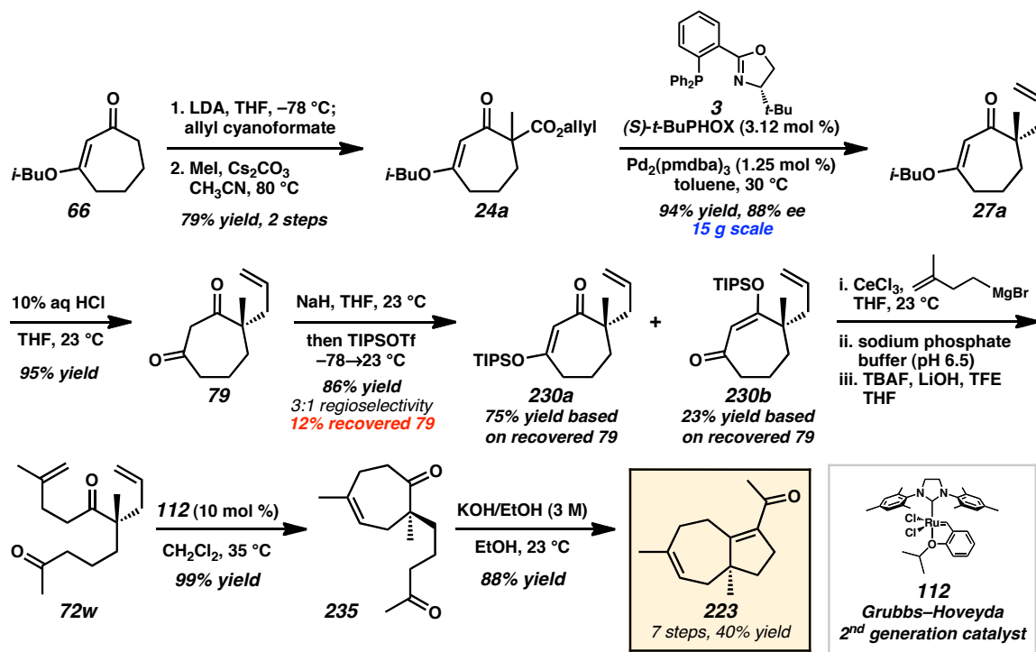
Scheme A4.1. Route to key intermediate enone 223 .
