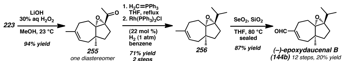
Scheme A4.2. Synthesis of (-)-epoxydaucenal B ( 144b ).
