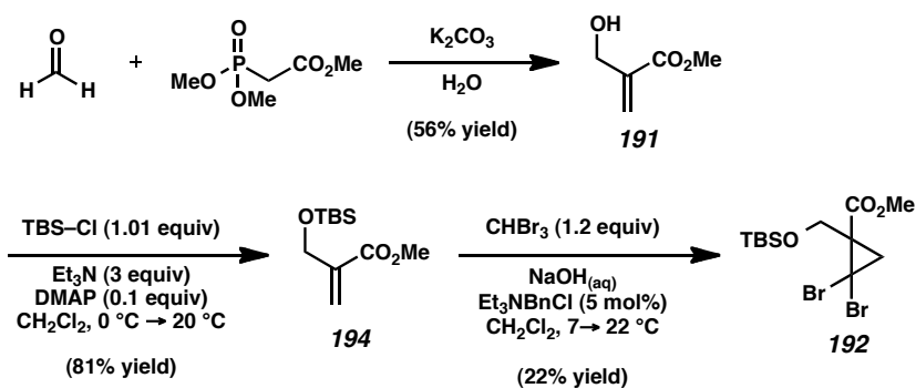
Scheme A5.2 Synthesis of dibromocyclopropane 192
