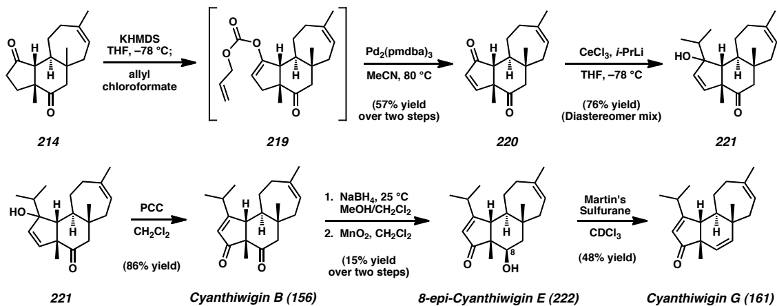
Scheme A1.3 Synthesis of cyanthiwigins B ( 156 ) and G ( 161 )
