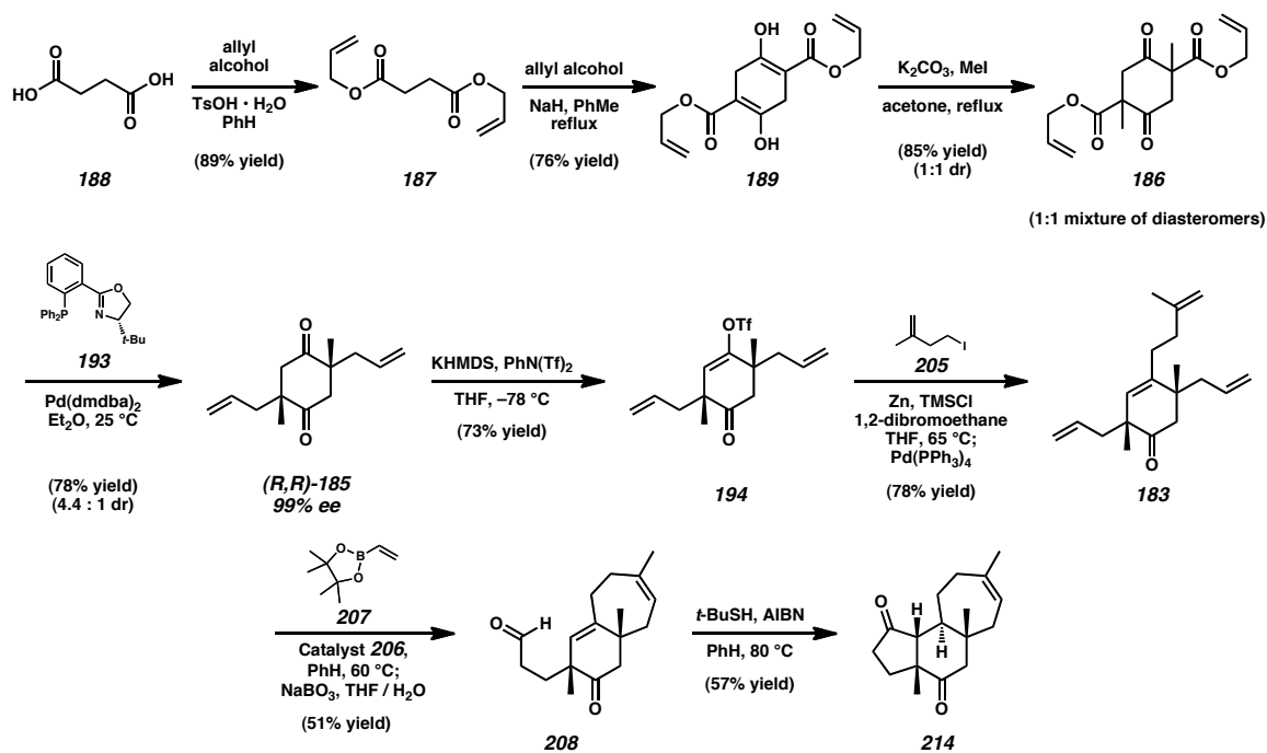
Scheme A1.1 Synthesis of tricyclic diketone 214
