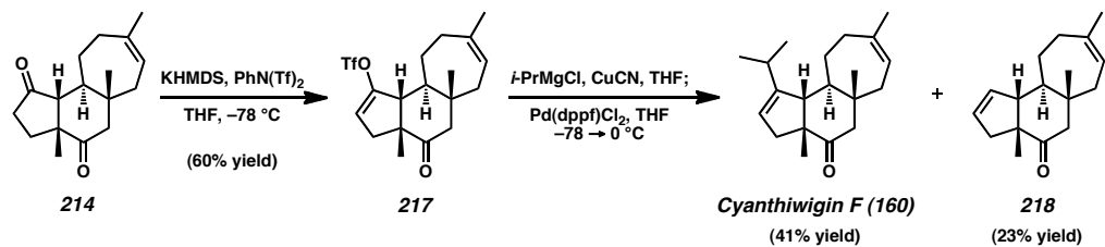
Scheme A1.2 Synthesis of cyanthiwigin F ( 160 )
