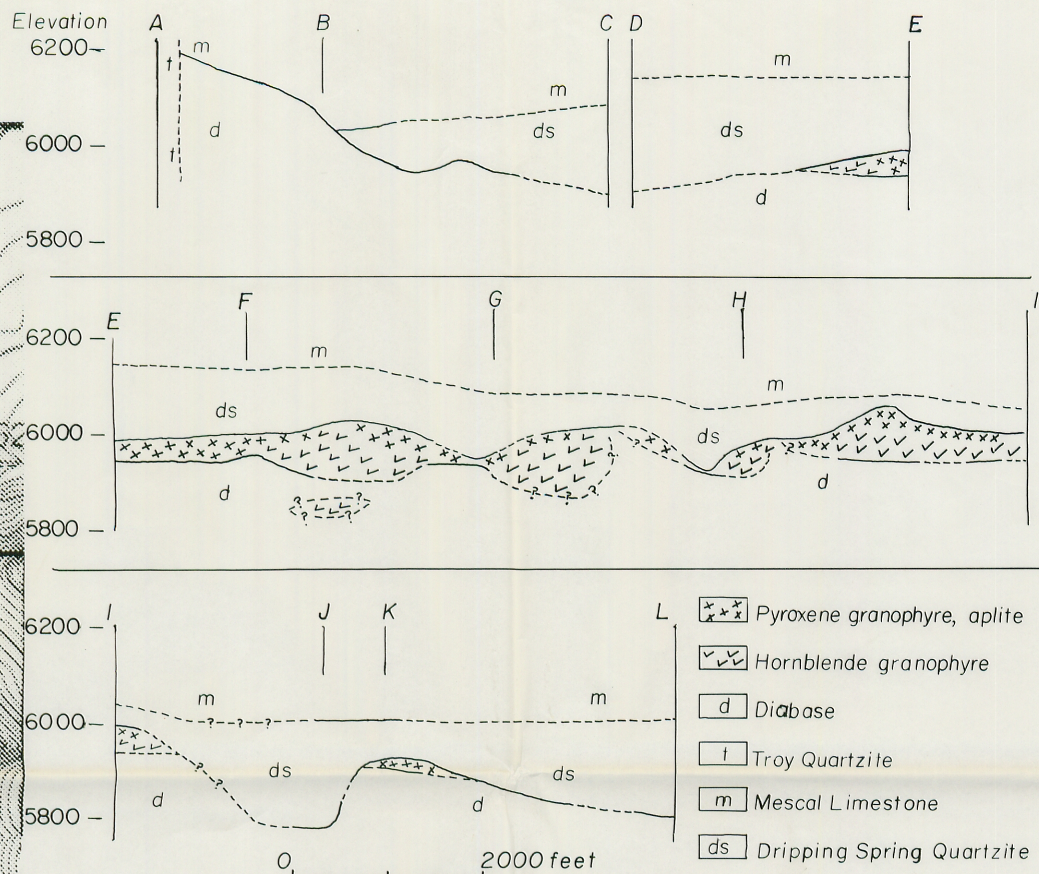
These sections show the relationships exposed on the ridge slopes projected onto vertical planes. The section lines are shown on the map.
