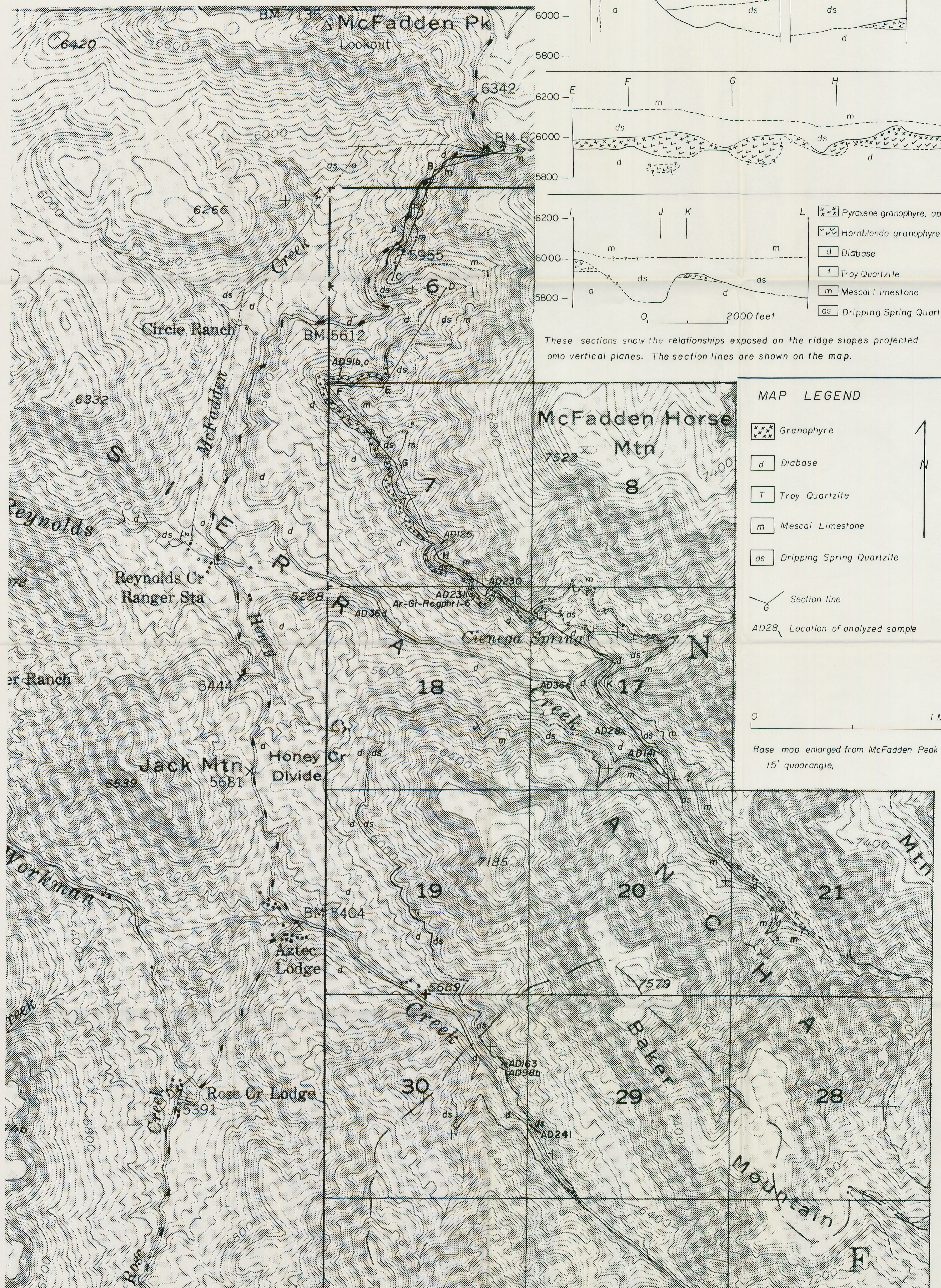
PLATE 4. Reynolds and Workman Creek areas
