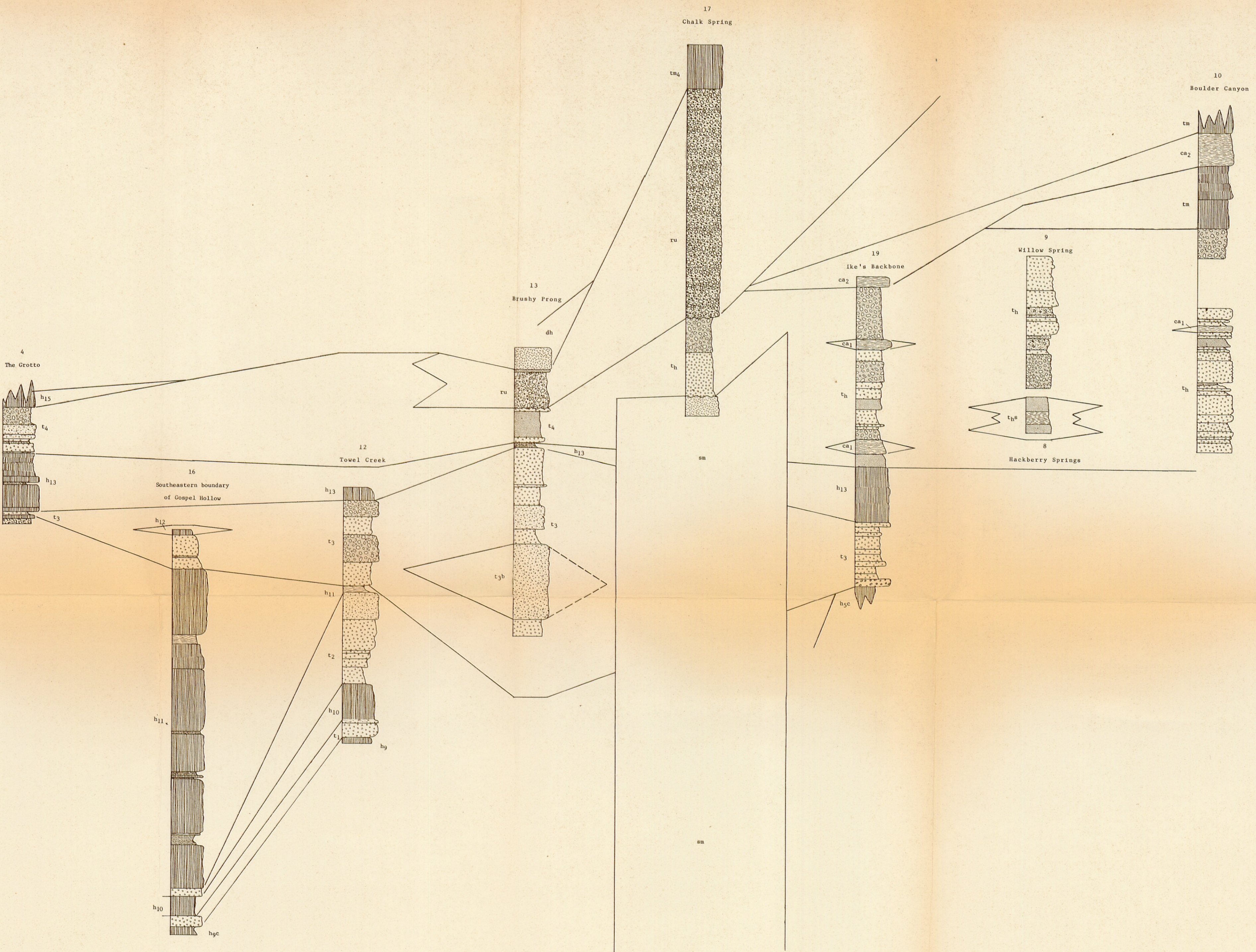
SECTION 4 CORRELATION OF THE DACITIC ROCKS
