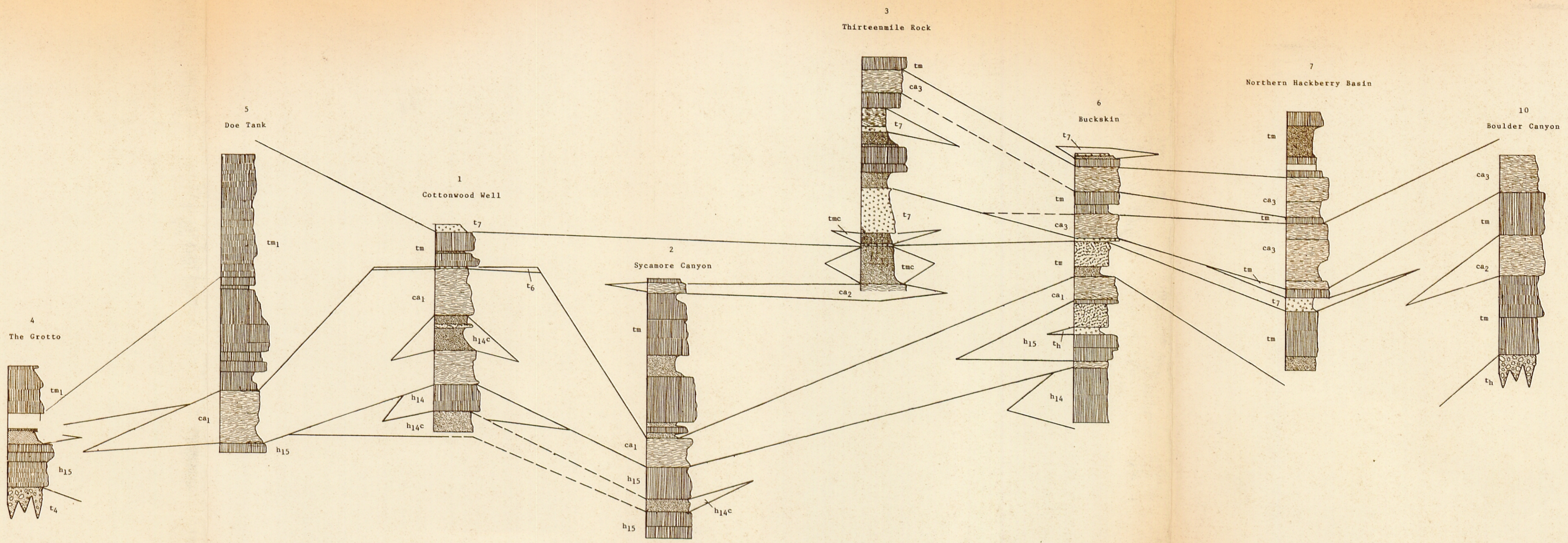
SECTION 3 CORRELATION OF THE THIRTEENMILE ROCK BASALT AND THE CIMARRON HILLS ANDESITE
