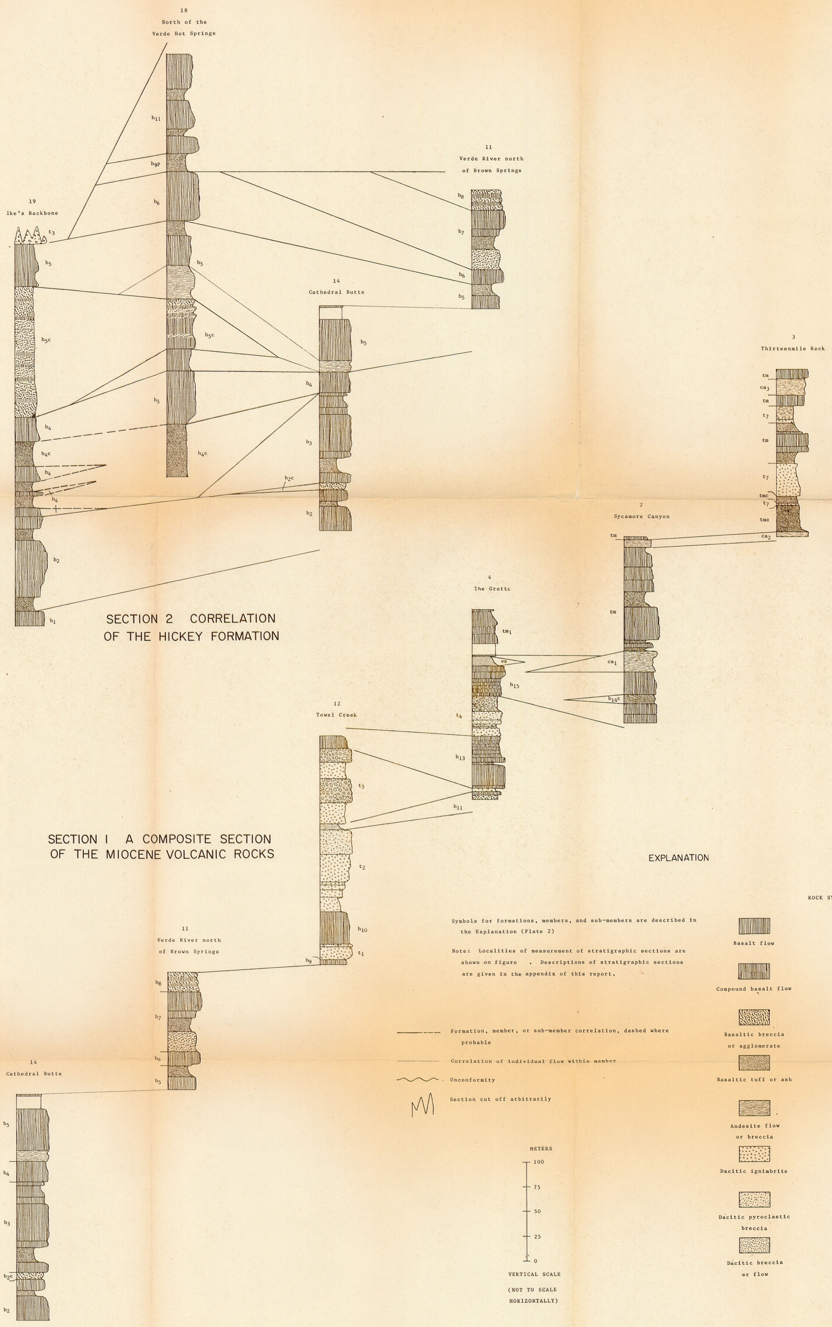
STRATIGRAPHIC SECTIONS SHOWING CORRELATION OF MIOCENE VOLCANIC ROCKS IN THE HACKBERRY MOUNTAIN VOLCANIC CENTER, YAVAPAI COUNTY, ARIZONA
