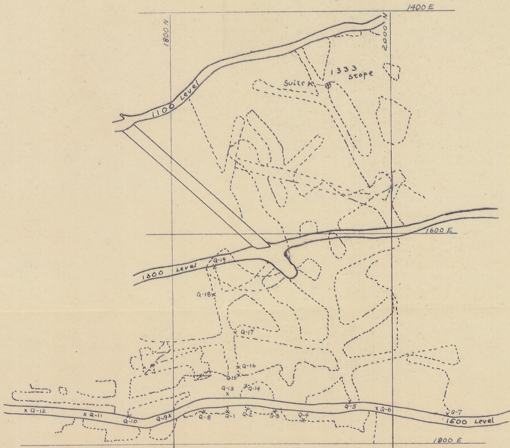
1100, 1300, & 1500 LEVELS, SIXTEEN-TO-ONE MINE ALLEGHANY, CALIF.
