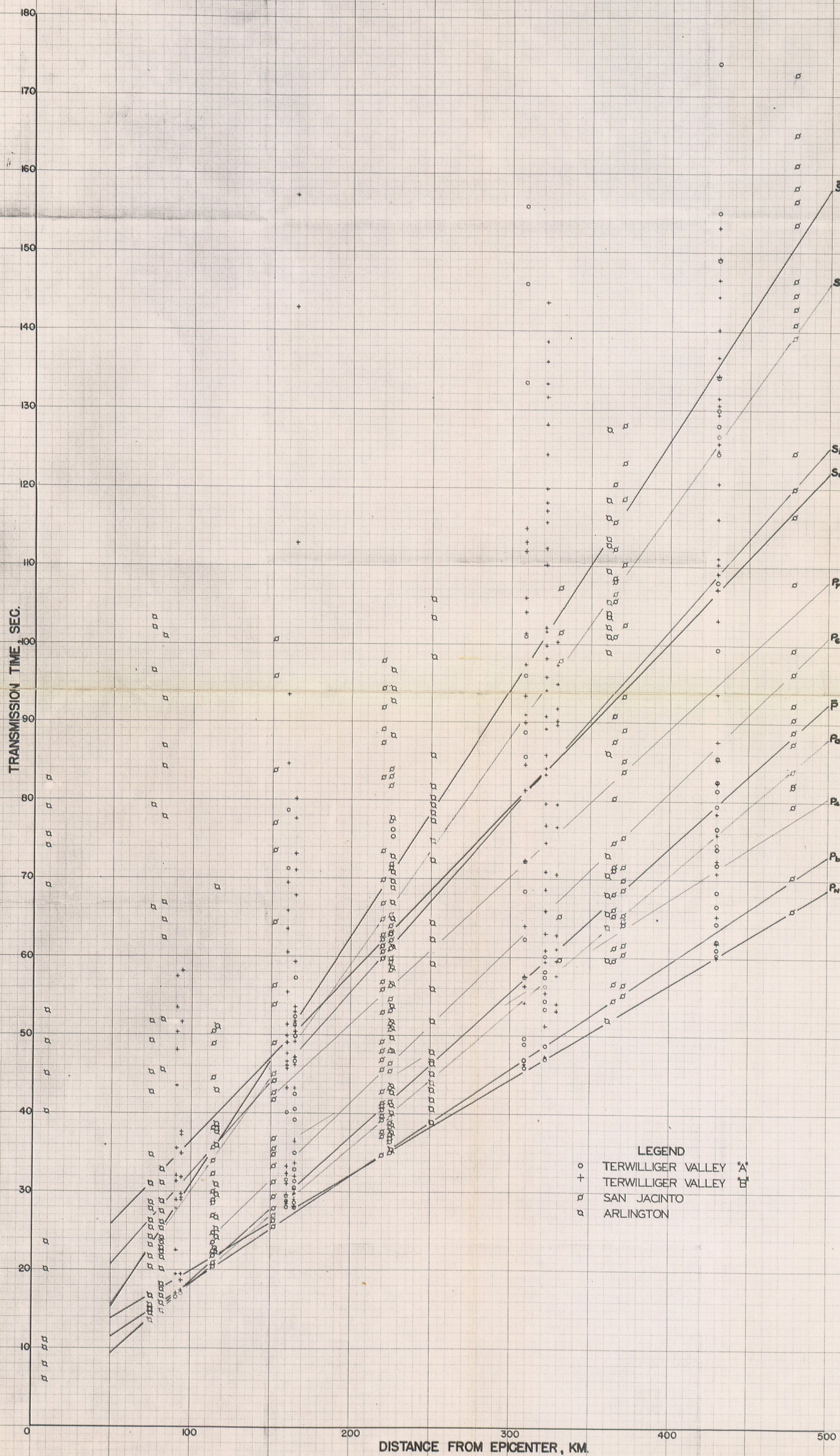
FIG. 2 TRAVEL TIME - DISTANCE CURVES TO ACCOMPANY REPORT BY A.J.GROBECKER
