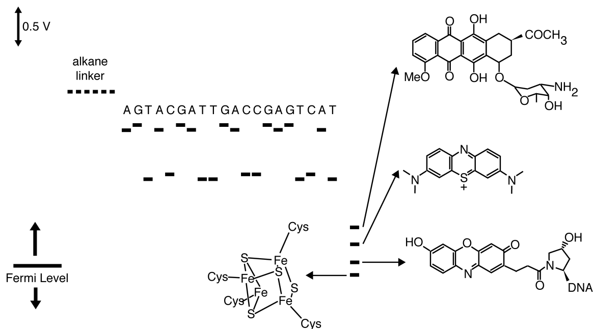
Figure 1.7. Scale diagram describing the relevant potentials for DNA-mediated CT through DNA self-assembled monolayers on gold. The potentials of the individual nucleotides are not accessible within the window of electrochemistry of DNA monolayers on Au. Nevertheless, facile DNA-mediated electrochemistry is observed for redox probes over DNA bridges. For all probes and sequences of well-matched duplexes, the tunneling through the alkane linker is rate limiting ( \sim 30 \text{ s}^{-1} ). Shown, in order from top, are daunomycin, methylene blue, Redmond Red, and a [4\text{Fe-4S}] cluster similar to those in the redox-active repair proteins EndoIII and MutY.
