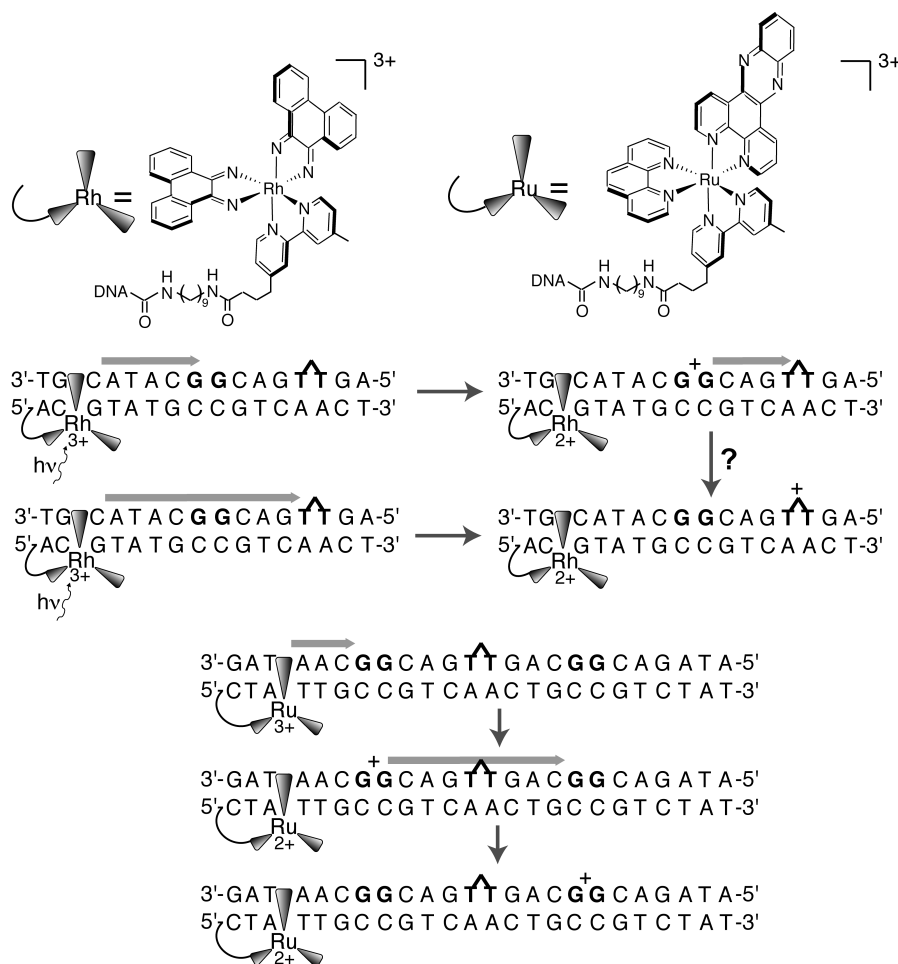
Figure 1.6. Oxidation and repair of thymine dimer ( \sim 1.8 eV) by tethered photoexcited [\text{Rh}(\phi)_2(\text{bpy}')]\text{DNA} ( 2.0 V) is unaffected by the intervening double guanine site ( 1.2 eV). Oxidation of double guanine sites by [\text{Ru}(\text{phen})(\text{bpy}')(\text{dppz})]\text{DNA} ( 1.5 eV) is unaffected by the presence of thymine dimer, which this oxidant lacks sufficient driving force to repair. The latter result implies that guanine radical is not competent to repair thymine dimers, in accordance with the known potentials. Hence either the guanine radical oxidized by [\text{Rh}(\phi)_2(\text{bpy}')]\text{DNA} does not relax prior to migration to the thymine dimer, or the guanine radical is not an intermediate in DNA-mediated oxidation of thymine dimer by [\text{Rh}(\phi)_2(\text{bpy}')]\text{DNA} .
