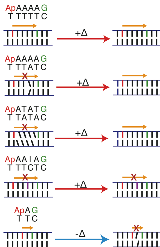
Figure 1.4. The sequence and temperature dependence of single-step oxidation of guanine by photoexcited 2-aminopurine (Ap) in DNA. 35,54,117 CT yield in well-matched Ap(A) 4 G increases with temperature ( +\Delta ), up to duplex melting. Two perturbations that disturb CT due to poor stacking dynamics, an A-A mismatch and the sequence ATAT, attenuate CT at room temperature but are comparable to the A 4 sequence at higher temperature, while CT through a perturbation that disturbs CT due to an electronic barrier, AAIA, is only partially recovered at high temperature. This argues that the CT activation is related to the flexibility of the bridge. At low temperature (77K), an intervening adenine eliminates CT from Ap to G, implying that the equilibrium conformation is not the CT active conformation.
