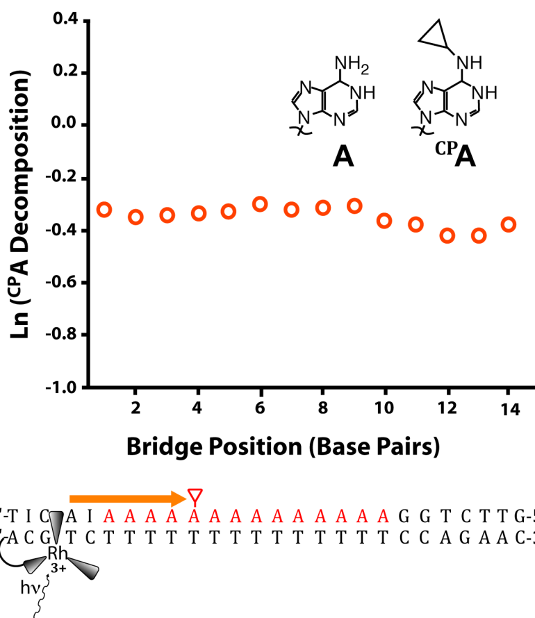
Figure 1.10. CT from photoexcited [\text{Rh}(\text{phi})_2(\text{bpy}') ]^{3+} to N -cyclopropyladenosine ( \text{CPA} ) across an adenine tract is distance-independent over 14 adenines. The rate of CT across the adenine tract, then, must be much faster than BET from the first adenine to the reduced rhodium. The driving force for recombination is only about 1.7 V, implying that BET should not be in the inverted region, consistent with evidence that BET from adenine to this rhodium complex is facile. 68 The lack of distance-dependence, in a system with a rapid competing process in BET and a charge trap that samples pre-equilibrium CT dynamics, implies extensive delocalization across the bridge. Adapted from Reference 17.
