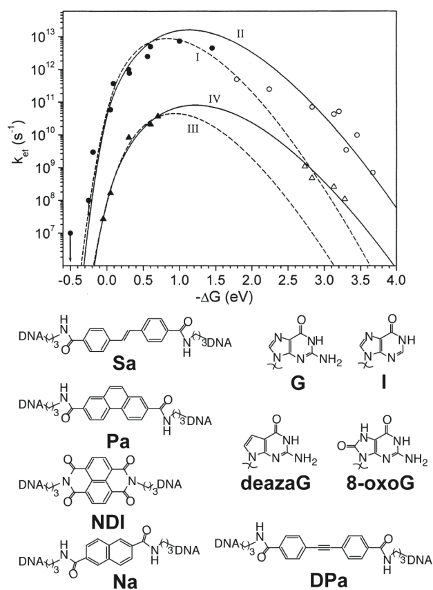
Figure 1.8. The driving force dependence for CT in photooxidant-bridged DNA hairpins is determined from time-resolved transient absorption studies of a series of five stilbene-derived photooxidants and four hole acceptor bases, following both charge separation (filled) and charge recombination (empty). Case I,II (circles): donor and acceptor are in contact. Case III,IV (triangles): donor and acceptor are separated by two TA base pairs. Case I,III are fit only to charge separation rates (dotted), while Case II,IV are fit to both charge separation and charge recombination rates (solid). Similar reorganization energies, about 1 eV for the nuclear reorganization energy and \sim 0.2 V for the solvent reorganization energy, are found for both Case II and Case IV. Adapted from Reference 167.
