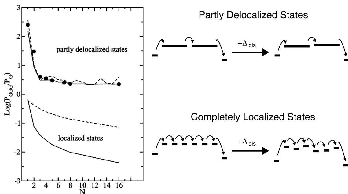
Figure 1.11. The variable-range hopping model predicts a shallow distance dependence for the rate of CT between G and GGG across an adenine tract of the opposing strand. Delocalized states, even in the absence of disorder (dashed lines), yield larger and shallower CT rates due to the smaller reorganization energy, and a shorter effective bridge length. In the presence of static disorder (solid lines), localized hopping is substantially attenuated due to the rugged energy landscape. Delocalized hopping, however, is relatively unaffected by static disorder, as the coupling is strong enough to allow tunneling through local barriers. Adapted from Reference 217, which fit data of Reference 207 using the interbase couplings of Reference 212, which are similar to the most recent calculated values. 208
