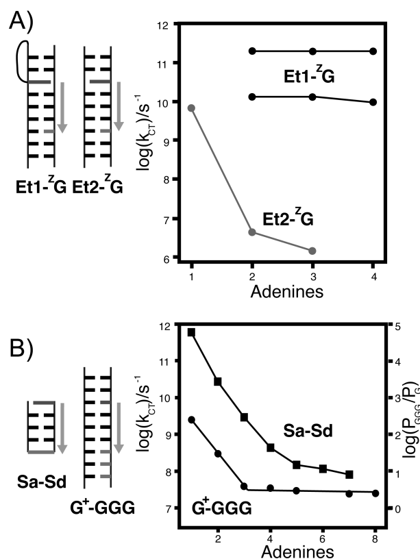
Figure 1.5. (A) The rate of coherent deazaguanine ( ^ZG ) oxidation by ethidium bromide is the same over short distances for both the flexible linkage ( Et1 , black, both CT rates shown) and the rigid linkage ( Et2 , gray). 27 For two intervening nucleotides, a sharp drop in rate is observed for the rigid Et^+ , but the rate is unaffected for the flexible Et^+ . (B) This steep drop in rate over short distances is consistent with that observed for oxidation of guanine by a photoinduced sugar radical (circles), 207 and CT between hairpin capping stilbenes (squares, photooxidation of Sd by Sa ), 125 and has been attributed to a crossover between coherent superexchange and incoherent hopping. In the latter case, comparison of injection and hole arrival rates supports superexchange for one or two intervening base pairs, and hopping for three or more base pairs between the stilbenes. Adapted from References 27, 207, and 125.
