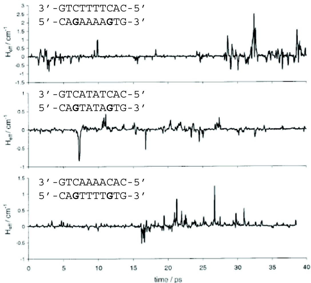
Figure 1.9. The time-dependent couplings between guanines separated by three different four-base sequence contexts, based on conformations generated through molecular dynamics. It is clear that the average value of coupling can be several orders of magnitude lower than the maximum coupling. For the poorly stacked, flexible ATAT sequence, strong coupling between the guanines is not achieved over the time-scale of the simulation. Adapted from Reference 211.
