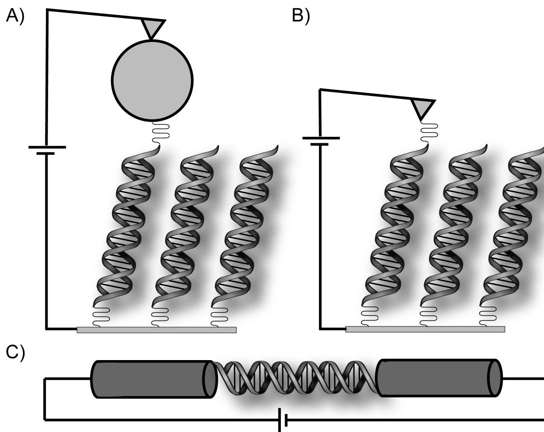
Figure 1.3. Devices for measurement of single molecule DNA conductivity through molecular contacts. In each case, currents between 10 and 100 nA are obtained for modest source-drain and gating voltages. A) A gold nanoparticle allows strong coupling between the EC-AFM tip and an individual 26mer DNA molecule on a gold electrode. 37 B) The gold STM tip is slowly brought in contact with thiol-modified DNA (8mer), allowing a histogram of conductance over many different orientations. 45 C) A single 15mer DNA is covalently attached across a gap between single-walled carbon nanotubes. 34
