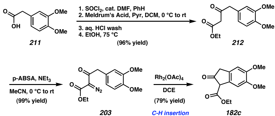
Scheme A6.1 The synthesis of \beta -ketoester 182c .
