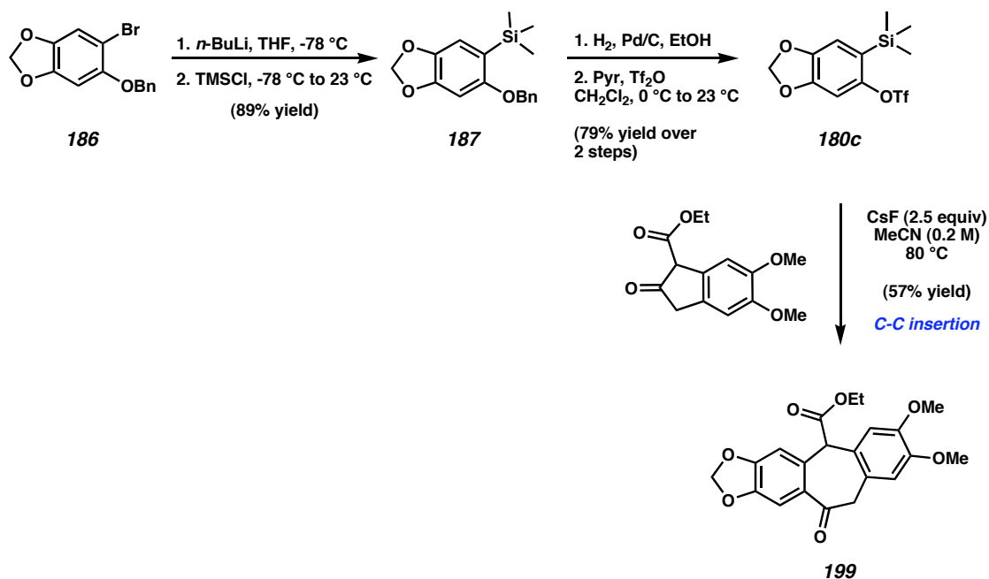
Scheme A6.2 The synthesis of ketoester 199 .
