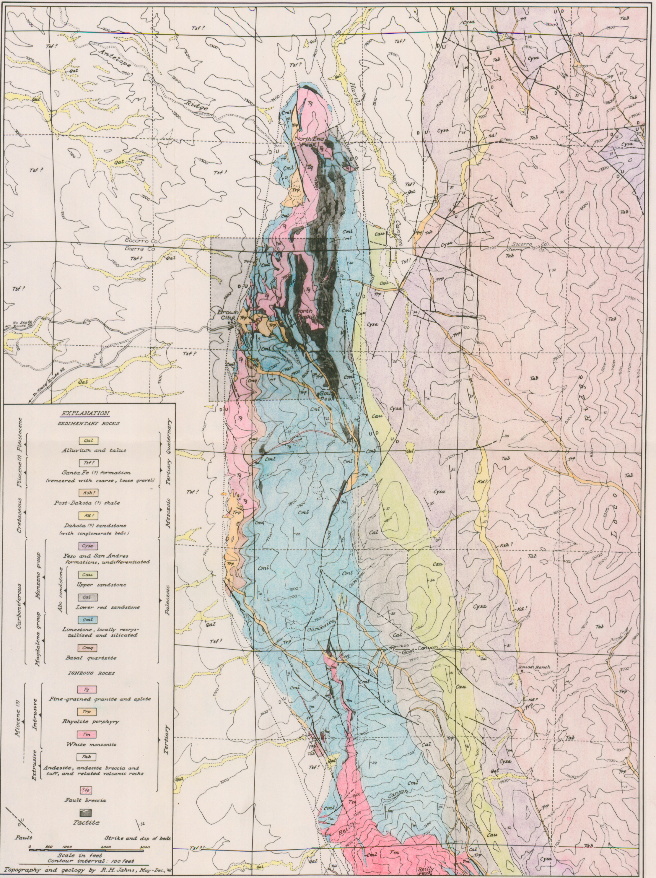
Plate 1. Geologic map of Iron Mountain and vicinity, Sierra and Socorro Counties, New Mexico
