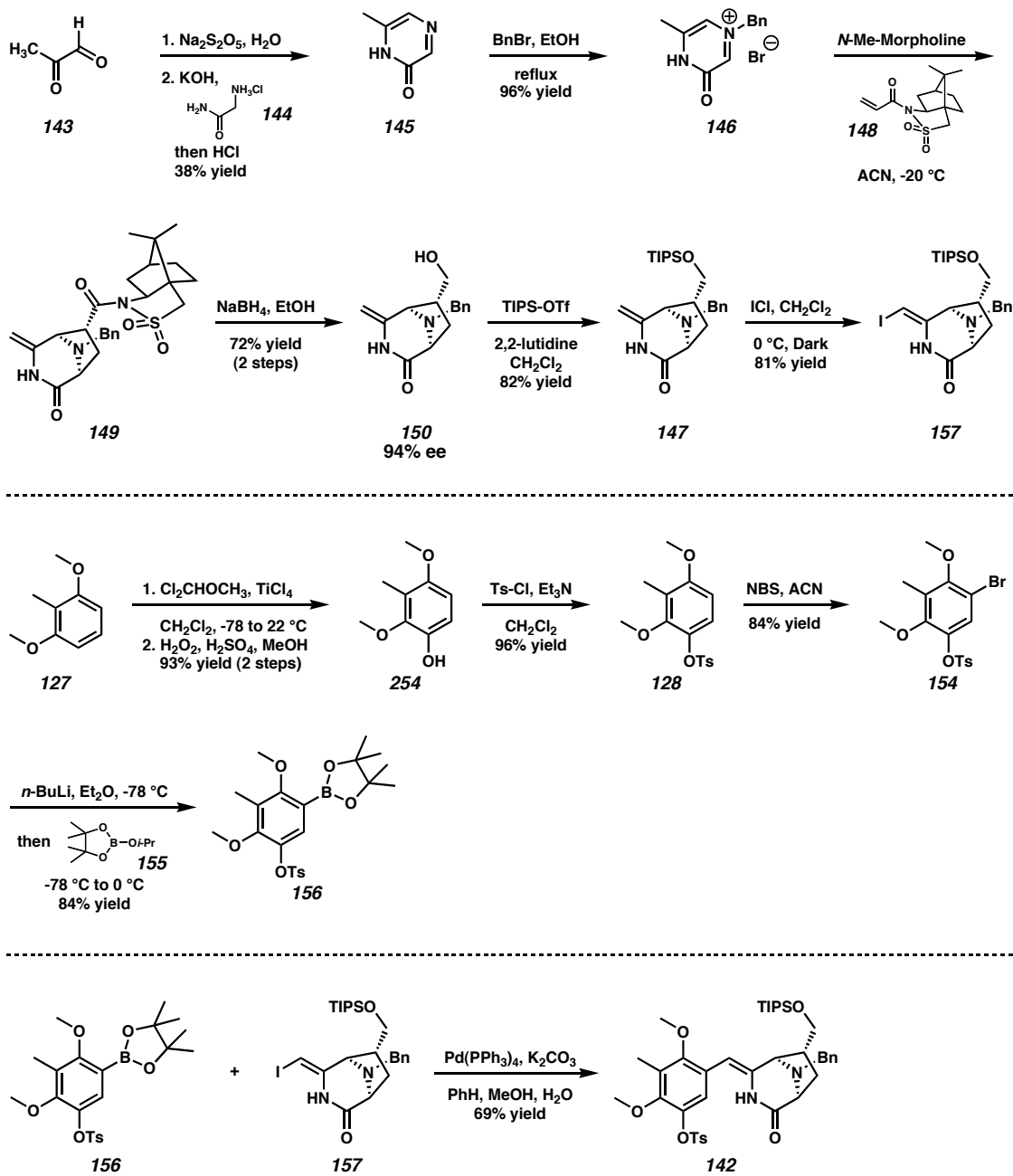
Scheme A1.1 Synthesis and Coupling of the Suzuki Substrates
