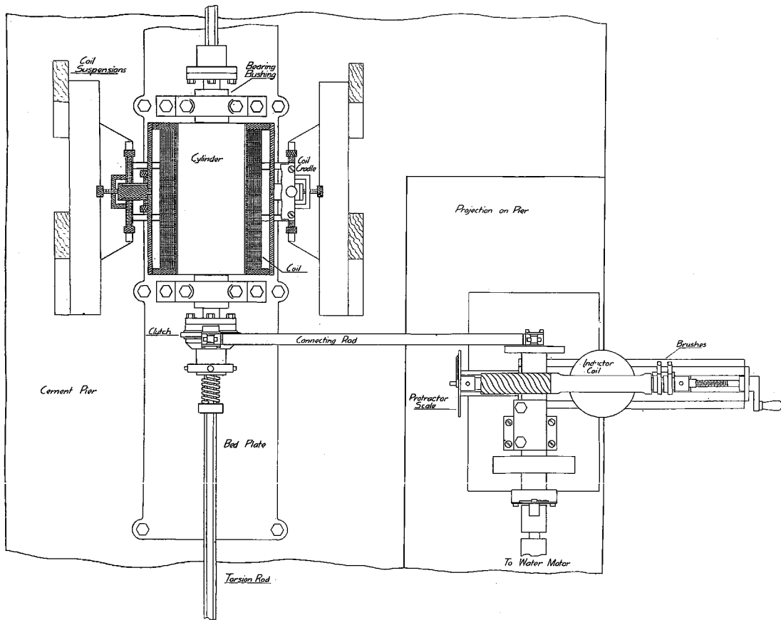
Figure 2 Front View of Apparatus
