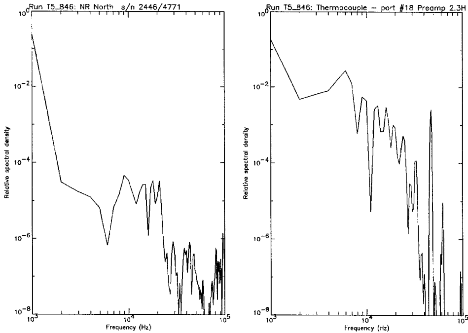
Figure 3.16: Frequency spectra of nozzle reservoir pressure and surface heat flux (gauge #18) for type IV flow at condition A; Shot T5-846.
