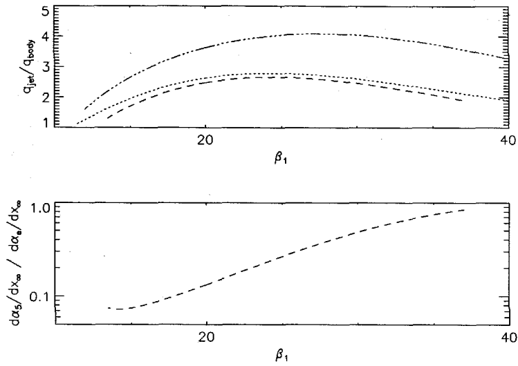
Figure 4.21: INFLUENCE OF IMPINGING SHOCK WAVE ANGLE, \beta_1 , AND REACTION RATE ON TYPE IV HEAT TRANSFER INTENSIFICATION AT MODERATE MACH NUMBER; P_\infty = 0.025 . The remaining parameters and format are the same as figure 4.19.
