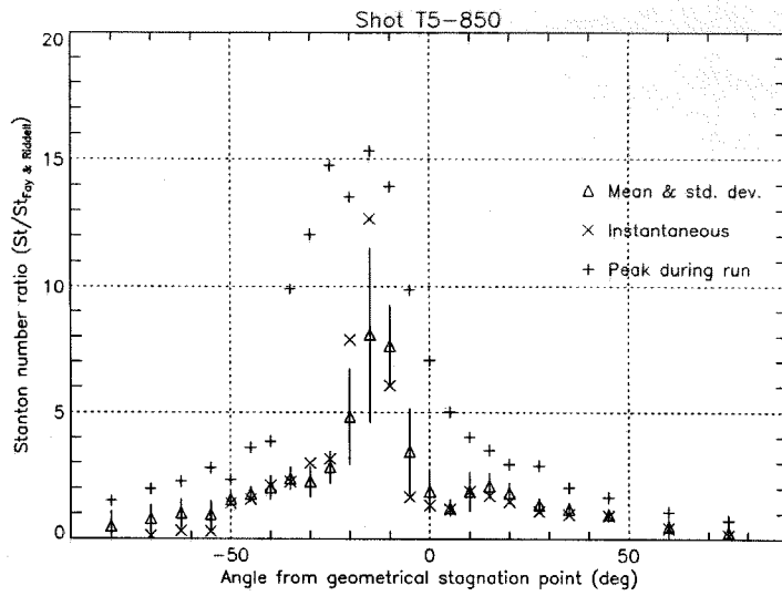
Figure C.10: Shot T5-850; condition A, g/D = 2.396 .
