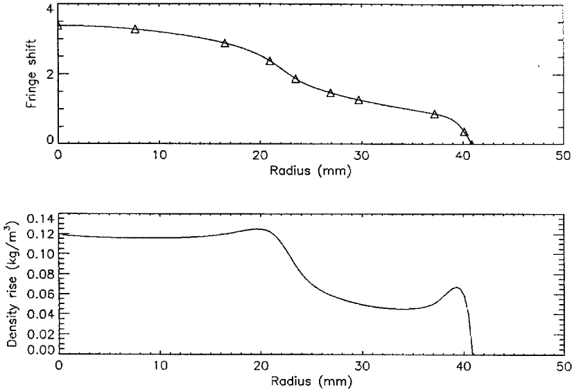
Figure B.4: Abel transformation of density field for flow over the blunt faced cylinder at test condition A; Shot T5-819.
