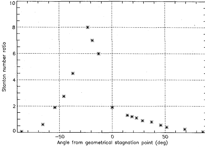
Figure 3.9: Envelope of maximum heat transfer rates about a spherical model (Edney [8]); M_\infty = 7 , \delta_1 = 5^\circ .
