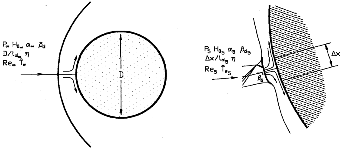
Figure 4.17: Adaption of the Fay & Riddell stagnation point solution to the jet impingement problem.
