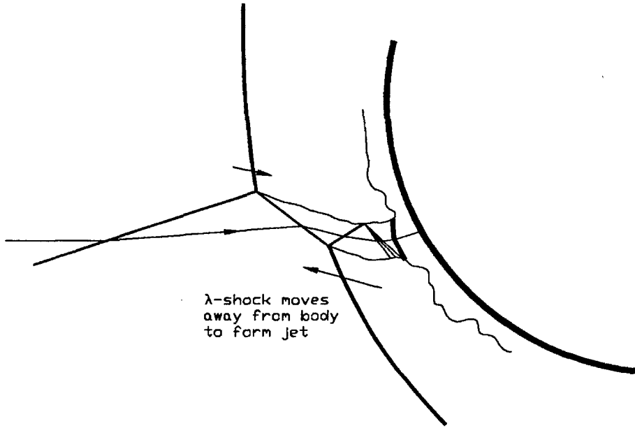
Figure 3.4: Interpretive sketch of jet formation.
