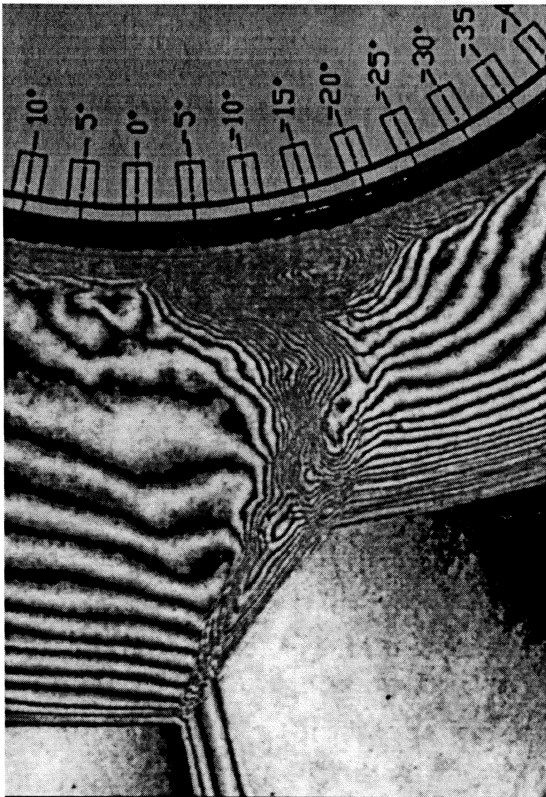
Figure C.11: Magnified view of holographic interferogram; Shot T5-850
