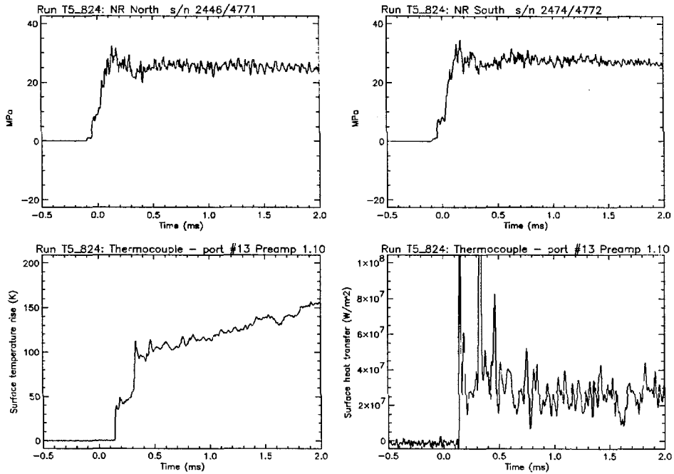
Figure 3.12: TEMPORAL CHARACTERISTICS OF THE FLOW WITHOUT SHOCK IMPINGEMENT AT CONDITION C; SHOT T5-824. Top row plots are the nozzle reservoir pressure. Bottom row plots are the stagnation point surface temperature and the heat flux inferred from it.
