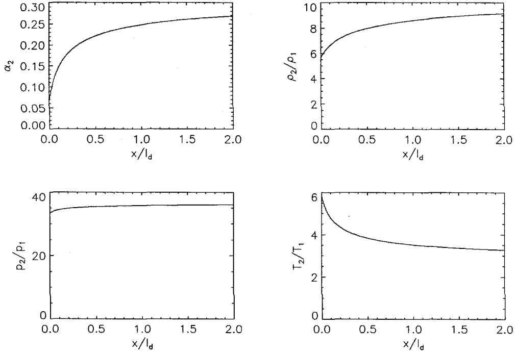
Figure 4.4: NONEQUILIBRIUM SOLUTION FOR THE RELAXATION DOWNSTREAM OF A TRANSLATIONAL DISCONTINUITY IN AN IDEAL DISSOCIATING GAS. The free-stream conditions are P = 0.0254 , H_0 = 0.56 , \hat{p}_d = 8.3 \times 10^6 , \alpha_1 = 0.051 , \eta = -2.5 . These conditions are equivalent to the high enthalpy test condition C that was used in the experimental portion of this investigation. For these conditions the characteristic length, \ell_d = 0.544\text{mm} , so that for a model diameter of 40 mm the flow is close to equilibrium.
