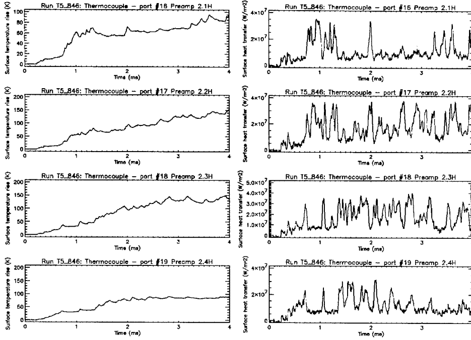
Figure 3.13: TEMPORAL VARIATION OF THE SURFACE HEAT FLUX FOR TYPE IV FLOW AT CONDITION A; SHOT T5-846. Top-bottom: \theta = -15^\circ, -20^\circ, -25^\circ, -30^\circ .
