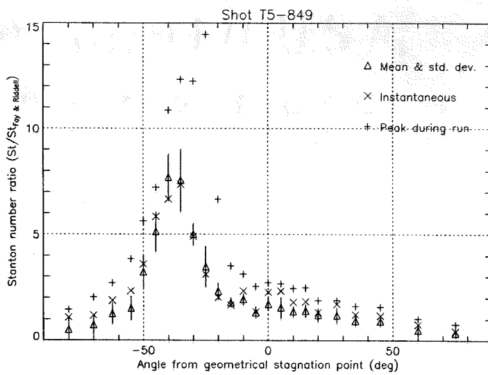
Figure C.4: Shot T5-849; condition A, g/D = 2.339 .
