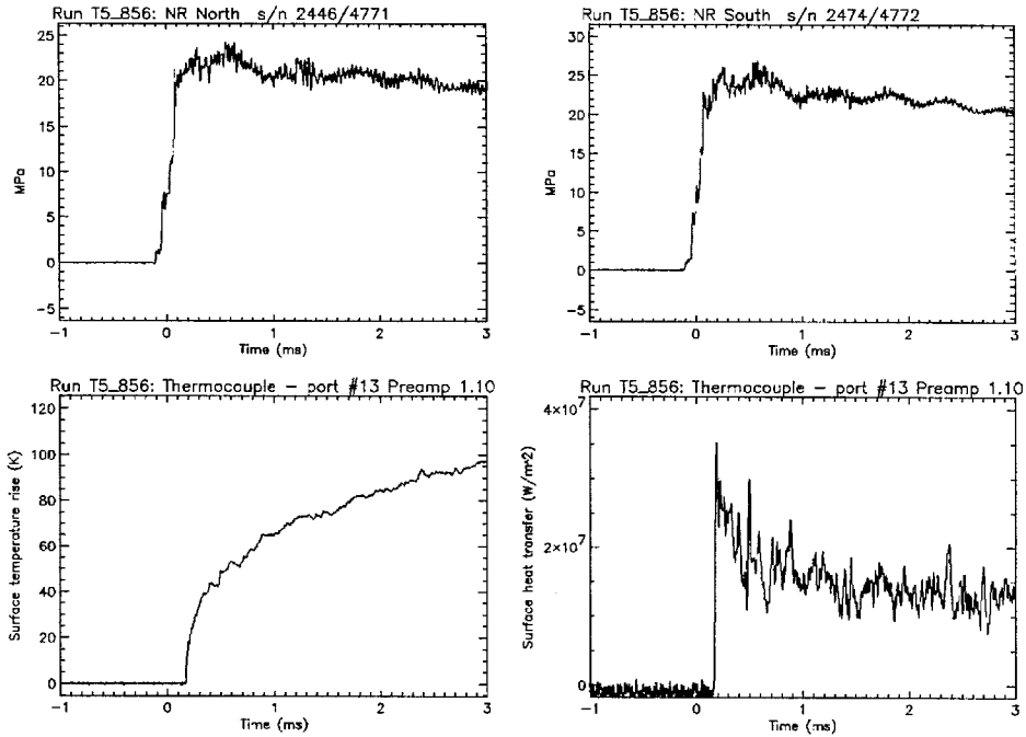
Figure 3.11: TEMPORAL CHARACTERISTICS OF THE FLOW WITHOUT SHOCK IMPINGEMENT AT CONDITION B; SHOT T5-856. Top row plots are the nozzle reservoir pressure. Bottom row plots are the stagnation point surface temperature and the heat flux inferred from it.
