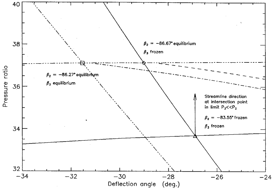
Figure 4.12: REPRESENTATION OF THE IDG \lambda -SHOCK CONFIGURATION IN THE p - \delta PLANE. Solid curves are the frozen shock loci. — · · — curves are the equilibrium shock loci. Solution points are; \Delta -frozen limit, \diamond -nonequilibrium approximation, square-equilibrium limit. — — — and — · — are the streamlines behind shock 2 in the nonequilibrium approximation and equilibrium limit respectively. Free-stream conditions are P = 0.025 , H_{0\infty} = 0.56 , \alpha_\infty = 0 , \hat{p}_d = 1 \times 10^7 , \beta_1 = 16^\circ .
