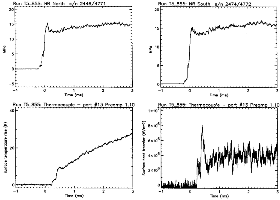
Figure 3.10: TEMPORAL CHARACTERISTICS OF THE FLOW WITHOUT SHOCK IMPINGEMENT AT CONDITION A; SHOT T5-855. Top row plots are the nozzle reservoir pressure. Bottom row plots are the stagnation point surface temperature and the heat flux inferred from it.
