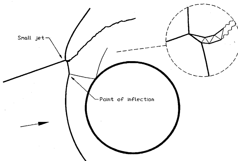
Figure A.6: Schematic of type V interference flow.
