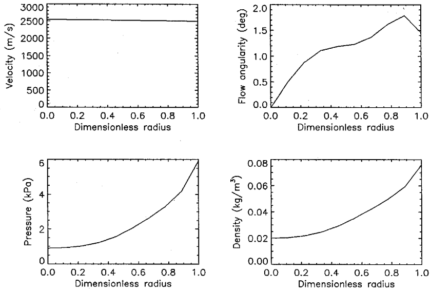
Figure B.1: Flow nonuniformity in the nozzle exit plane for test condition A.
