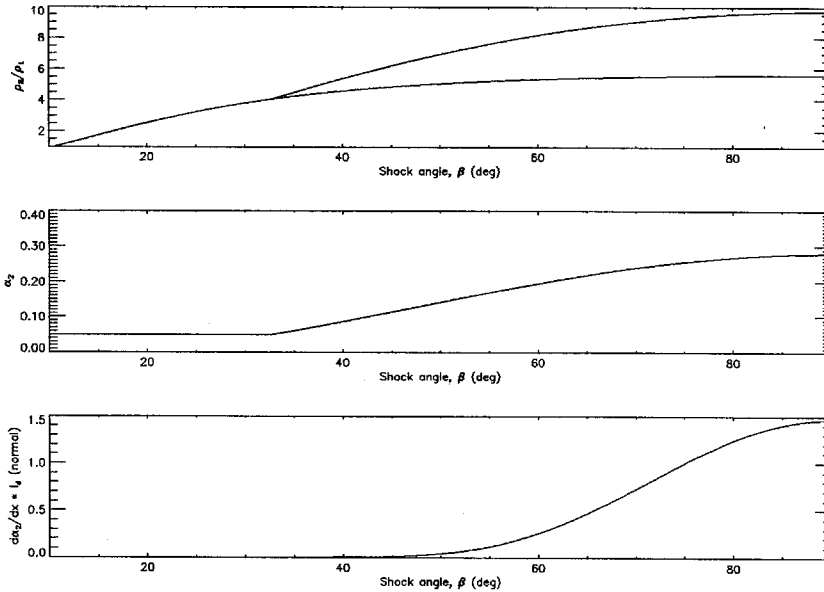
Figure 4.6: Frozen and equilibrium density ratio, equilibrium dissociation level, and initial dissociation rate as functions of shock angle for an oblique wave in an ideal dissociating gas. The free-stream conditions are P = 0.025 , H_0 = 0.55 , \alpha_1 = 0.05 , \hat{p}_d = 1 \times 10^7 . The discontinuity in slope at \beta = 33^\circ arises intentionally as a consequence of the frozen free-stream dissociation level, \alpha_1 .
