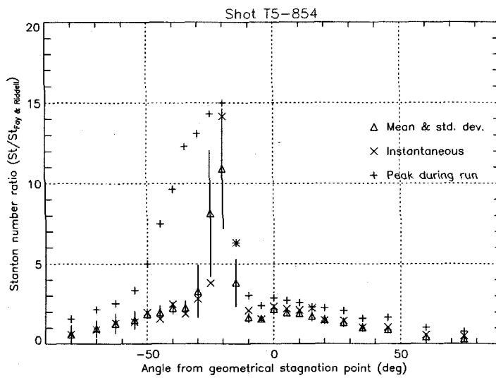
Figure C.6: Shot T5-854 (holographic shadowgraph); condition A, g/D = 2.368 .
