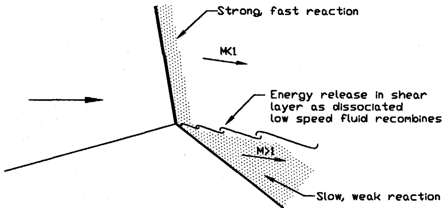
Figure 1.8: Real gas effects at a \lambda -shock intersection point.
