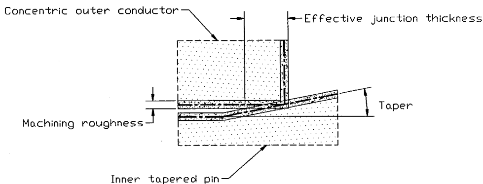
Figure E.3: Effective thickness of thermocouple junction.
