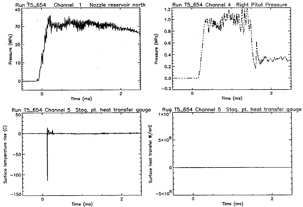
Figure E.5: STAGNATION POINT HEAT TRANSFER MEASUREMENT FOR SPHERE IN HYPERVELOCITY FLOW USING DUMMY CONSTANTAN – CONSTANTAN THERMOCOUPLE AT CONDITION C. The large drop in the pitot pressure at t = 1.5\text{ms} was caused by the passage of an oblique shock wave.
