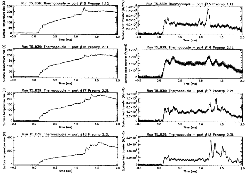
Figure 3.15: TEMPORAL VARIATION OF THE SURFACE HEAT FLUX FOR TYPE IV FLOW AT CONDITION C; SHOT T5-839. Top-bottom: \theta = -10^\circ, -15^\circ, -20^\circ, -25^\circ .
