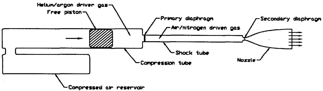
Figure 2.1: Schematic representation of the T5 free piston driver shock tunnel.
