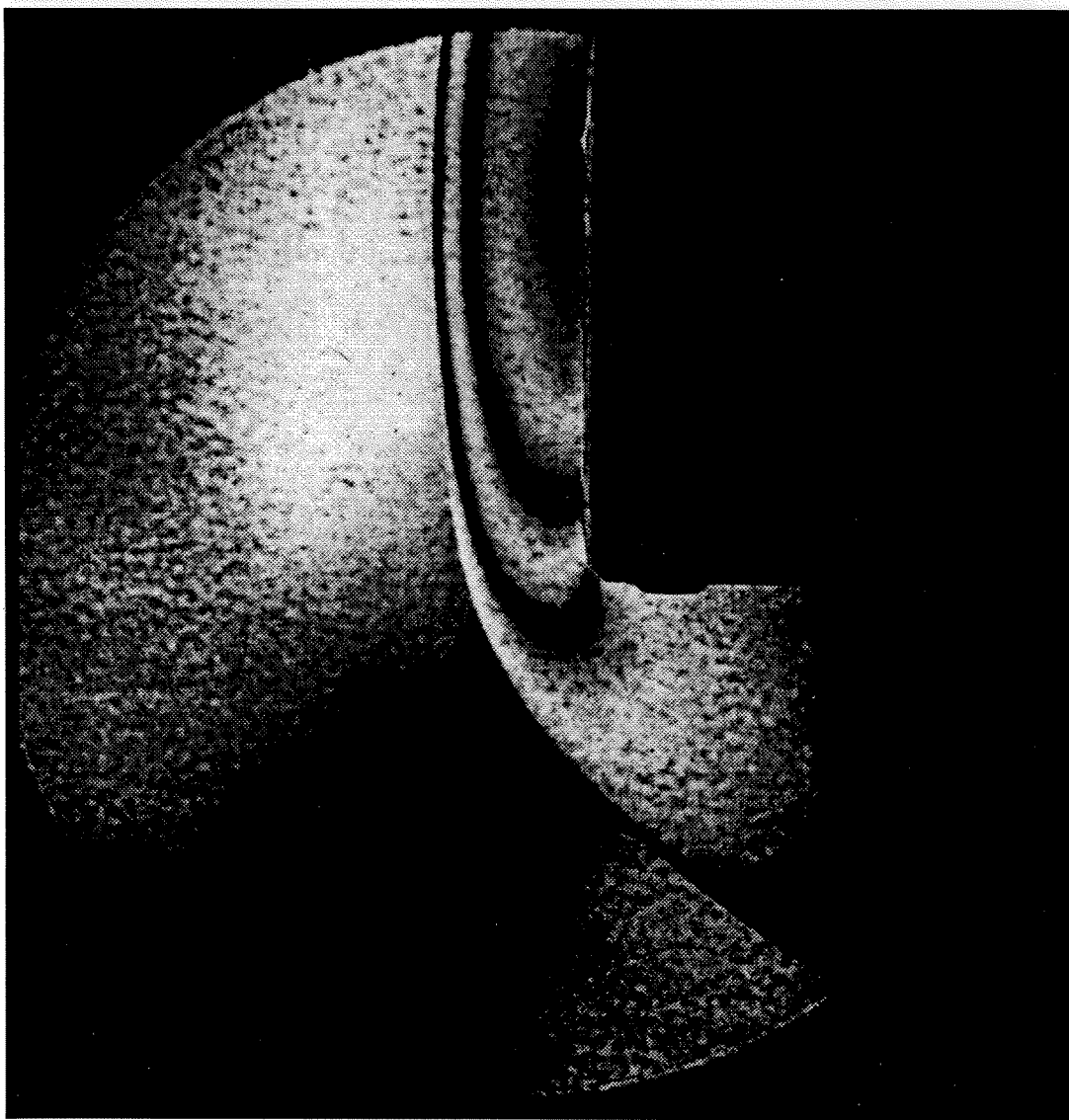
Figure C.49: Flow over a \phi 50\text{mm} blunt cylinder without shock impingement. Shot T5-820; condition C.
