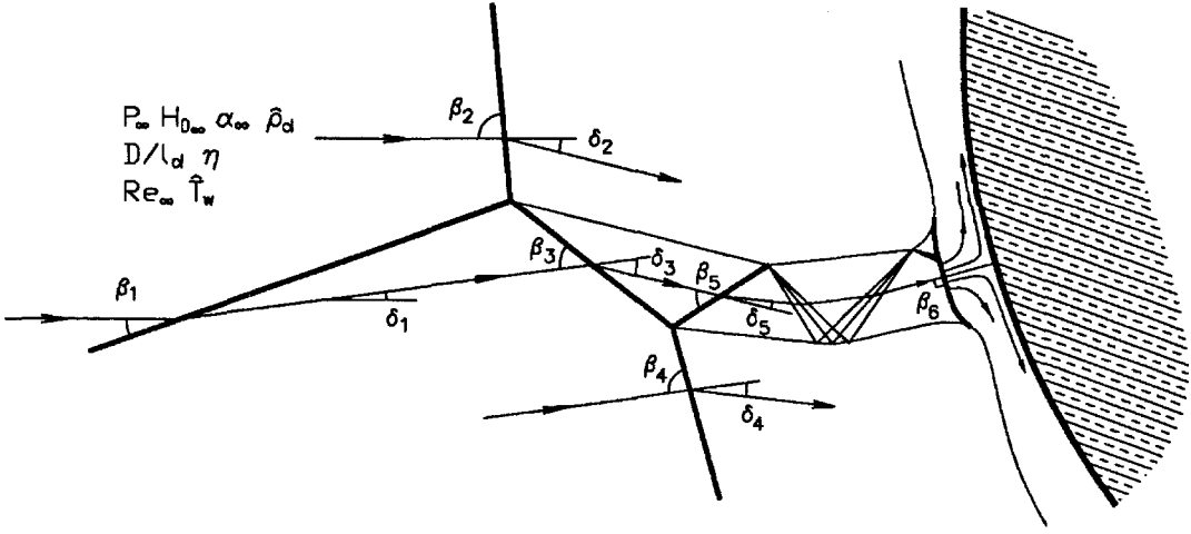
Figure 4.10: Schematic of flow field and shock wave notation for the type IV interaction in the vicinity of the impingement point.
