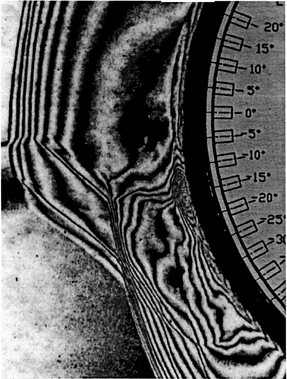
Figure C.33: Magnified view of holographic interferogram; Shot T5-837
