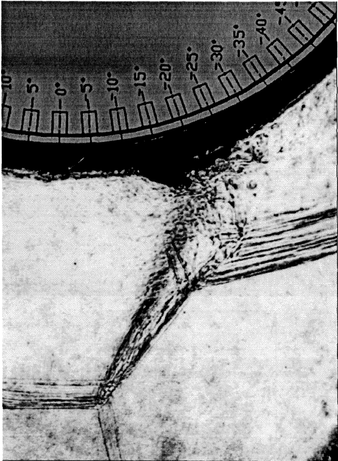
Figure C.7: Magnified view of holographic shadowgraph; Shot T5-854
