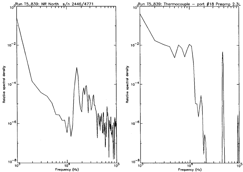
Figure 3.18: Frequency spectra of nozzle reservoir pressure and surface heat flux (gauge #18) for type IV flow at condition C; Shot T5-839.
