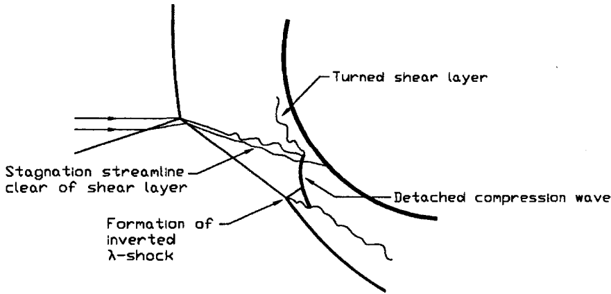
Figure 3.3: Interpretive sketch of detachment of the compression wave.
