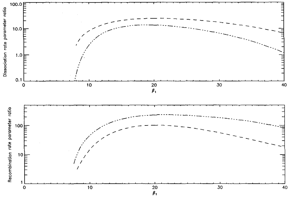
Figure 4.24: REACTION RATE PARAMETERS FOR THE TYPE IV JET STAGNATION POINT. Upper plot is the ratio of the dissociation rate parameters in the form, \frac{\Delta_s}{\Delta_\infty} \cdot \frac{D}{\Delta x} . Lower plot is the ratio of the recombination rate parameters, \frac{\Sigma_s}{\Sigma_\infty} \cdot \frac{D\zeta_{2jet}}{\Delta x\zeta_{2body}} . — · — curves are the equilibrium solutions. — — — curves are the nonequilibrium solutions. The free-stream conditions are P_\infty = 0.010 , H_{0\infty} = 0.6 , \hat{\rho}_{d\infty} = 1 \times 10^7 , \alpha_\infty = 0 .
