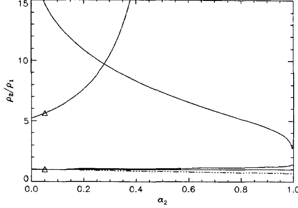
Figure 4.3: EQUILIBRIUM SHOCK SOLUTION IN THE \hat{\rho} - \alpha_2 PLANE. The free-stream conditions are P = 0.025 , H_0 = 0.55 , \hat{\rho}_d = 1 \times 10^7 , \alpha_1 = 0.05 .
