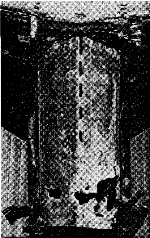
Figure 1.2: Damage to X-15 vertical stabilizer caused by impingement of scram-jet inlet shock wave (Edney [8]).
