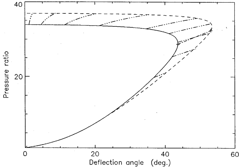
Figure 4.7: p - \delta PLANE REPRESENTATION OF AN OBLIQUE SHOCK WAVE FOR AN IDEAL DISSOCIATING GAS. Solid curve is the frozen locus. Dashed curve is the equilibrium locus. \cdots are streamlines for shock angles \beta = 40^\circ, 50^\circ, 60^\circ, 68.5^\circ, 75^\circ, 80^\circ, 85^\circ, 87.5^\circ, 89^\circ and 89.75^\circ respectively. -\cdot- is the mapping of the frozen sonic line connecting the frozen and equilibrium limits (+). The free stream conditions approximate test condition C that was used in the experimental investigation; P = 0.025, H_0 = 0.55, \hat{p}_d = 1 \times 10^7, \alpha_1 = 0.05 .
