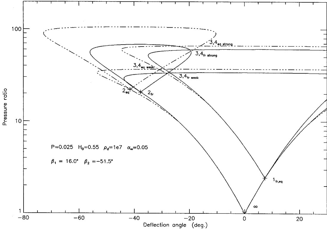
Figure 4.9: p - \delta PLANE REPRESENTATION OF THE INTERACTION OF OBLIQUE SHOCK WAVES IN AN IDEAL DISSOCIATING GAS. The shock angles are \beta_1 = 16^\circ , \beta_2 = -51.5^\circ and the numbering of the states is given in figure A.3. The free-stream conditions are P = 0.025 , H_0 = 0.55 , \hat{\rho}_d = 1 \times 10^7 , \alpha_1 = 0.05 . Solid curves are the frozen shock loci. — · · · — are the equilibrium shock loci.
