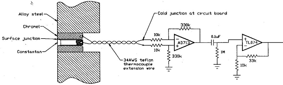
Figure E.4: Schematic of amplifier circuit.
