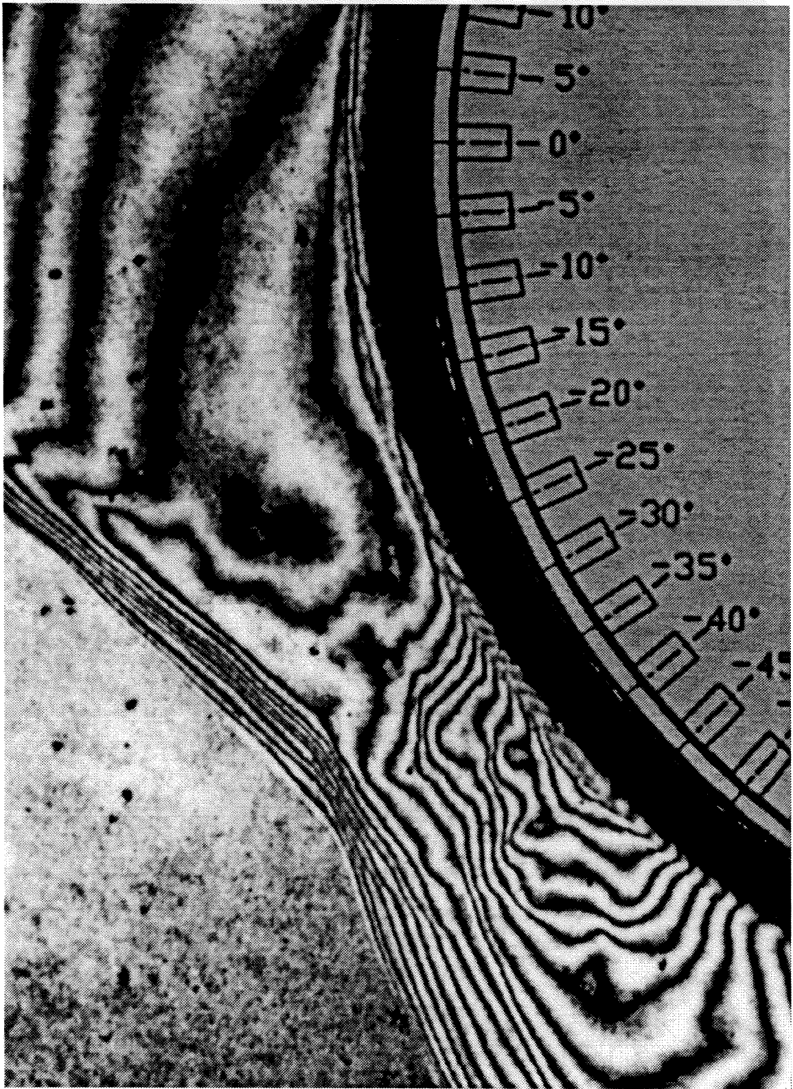
Figure C.27: Magnified view of holographic interferogram; Shot T5-838
