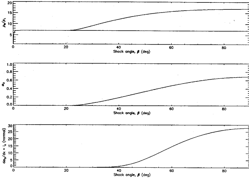
Figure 4.5: Frozen and equilibrium density ratio, equilibrium dissociation level, and initial dissociation rate as functions of shock angle for an oblique wave in an ideal dissociating gas. The free-stream conditions are P = 1 \times 10^{-6} , H_0 = 1.0 , \alpha_1 = 0 , \hat{p}_d = 1 \times 10^8 .
