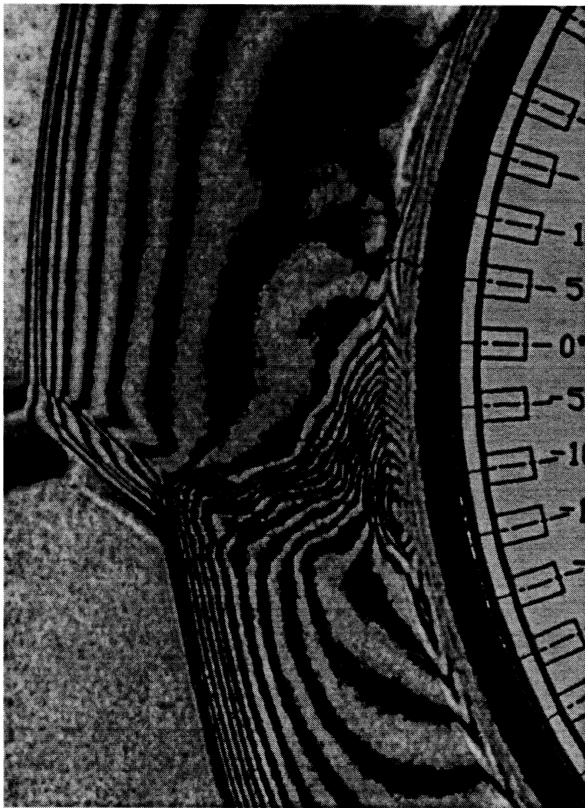
Figure C.39: Magnified view of holographic interferogram; Shot T5-829
