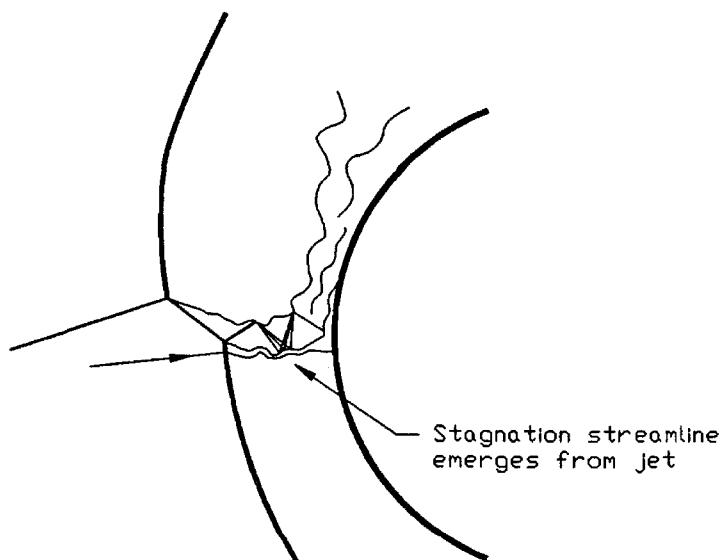
Figure 3.5: Emergence of the stagnation streamline from the supersonic jet.
