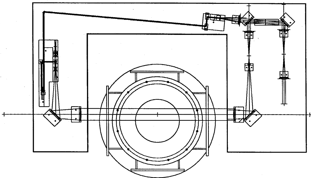
Figure 2.7: Arrangement of the optical apparatus with respect to the test section.
