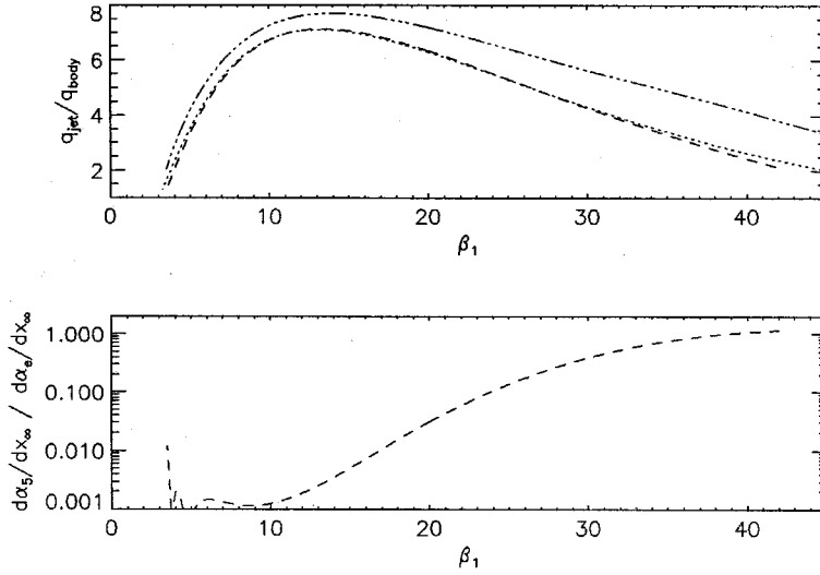
Figure 4.19: INFLUENCE OF IMPINGING SHOCK WAVE ANGLE, \beta_1 , AND REACTION RATE ON TYPE IV HEAT TRANSFER INTENSIFICATION AT VERY HIGH MACH NUMBER; P_\infty = 0.002 . From top: Heat transfer intensification, \frac{q_{jet}}{q_{body}} \sqrt{\frac{\Delta x}{D} \frac{\zeta_{1body}^2 \zeta_{2body}}{\zeta_{1jet}^2 \zeta_{2jet}}} and jet reaction rate ratio, \frac{d\alpha_s}{d\hat{x}_\infty} / \frac{d\alpha_e}{d\hat{x}_\infty} . . . . . curve is the frozen solution. — . . . — curve is the equilibrium solution. --- curve is the nonequilibrium solution in the limit \frac{d\alpha_1}{d\hat{x}_\infty}, \frac{d\alpha_3}{d\hat{x}_\infty}, \frac{d\alpha_5}{d\hat{x}_\infty} \ll \frac{d\alpha_2}{d\hat{x}_\infty}, \frac{d\alpha_4}{d\hat{x}_\infty}, \frac{d\alpha_6}{d\hat{x}_\infty} . The parameters are H_{0\infty} = 0.6 , \hat{\rho}_d = 1 \times 10^7 and \alpha_\infty = 0 .
