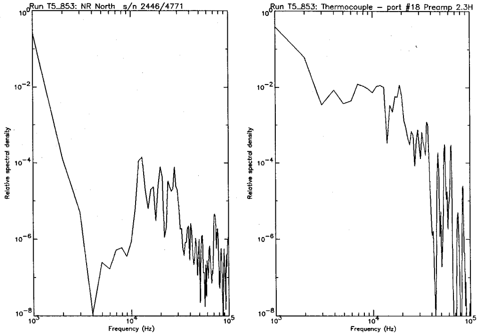
Figure 3.17: Frequency spectra of nozzle reservoir pressure and surface heat flux (gauge #18) for type IV flow at condition B; Shot T5-853.
