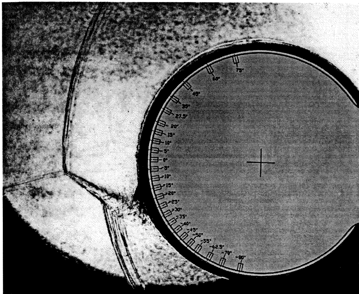
Figure 1.4: Holographic shadowgraph of the impingement of an oblique shock wave near the geometrical stagnation point of a cylinder in hypersonic flow. Following Edney [8], this flow is categorized as type IV.
