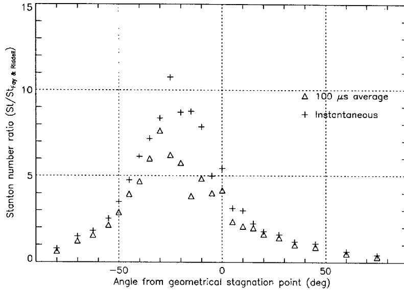
Figure 3.7: Envelope of maximum heat transfer rates around the model at condition B.
