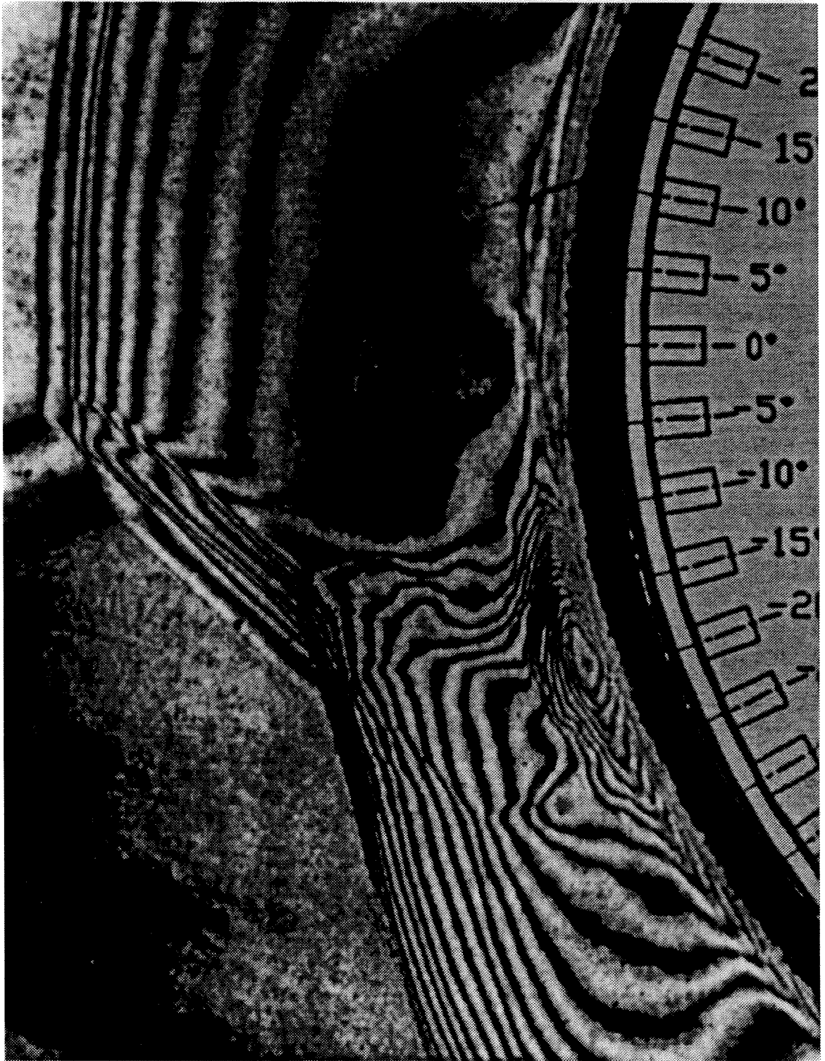
Figure C.35: Magnified view of holographic interferogram; Shot T5-830
