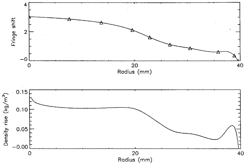
Figure B.5: Abel transformation of density field for flow over the blunt faced cylinder at test condition C; Shot T5-820.
