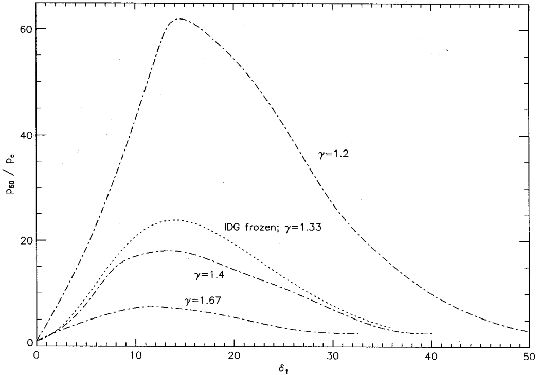
Figure 1.7: RATIO OF JET IMPINGEMENT PRESSURE TO UNDISTURBED STAGNATION POINT PRESSURE AS A FUNCTION OF INCIDENT SHOCK FLOW DEFLECTION ANGLE, \delta_1 . — · — curves are for the perfect gas model with M_\infty = 10 (after Edney [8]; Figure 7-9). · · · · curve is for the IDG model in the frozen limit with P_\infty = 0.0075 and \alpha_\infty = 0 .
