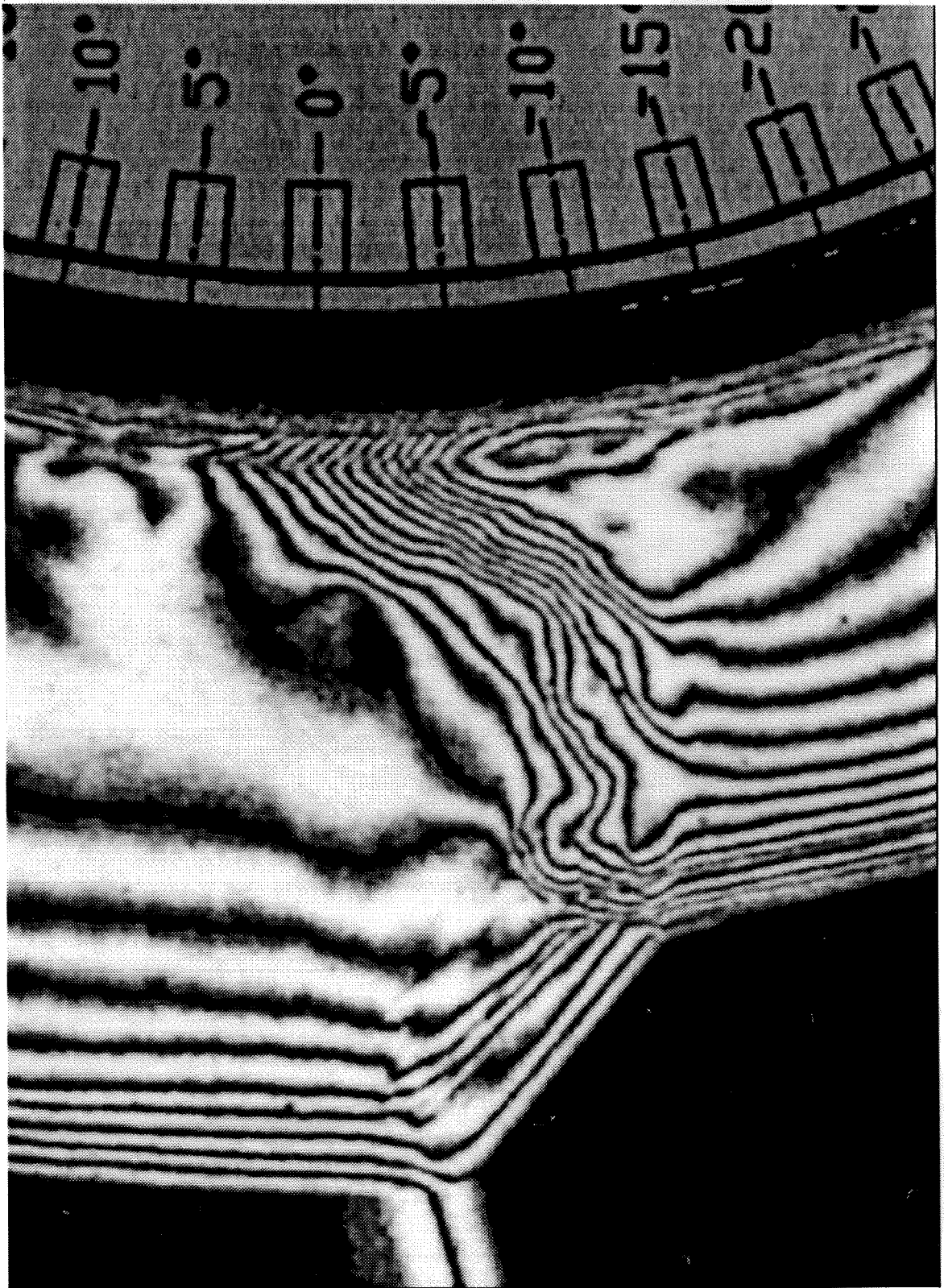
Figure C.18: Magnified view of holographic interferogram; Shot T5-852
