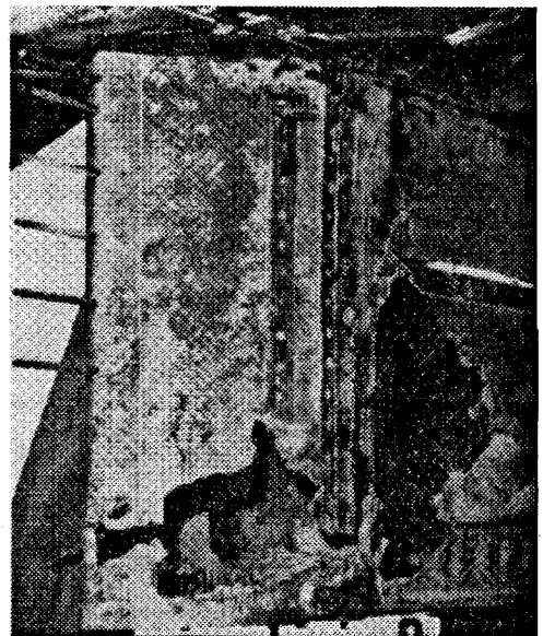
Figure 1.2: Damage to X-15 vertical stabilizer caused by impingement of scram-jet inlet shock wave (Edney [8]).
