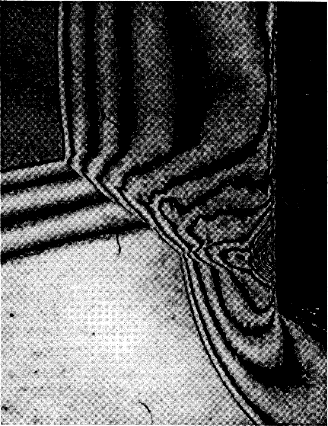
Figure C.48: Flow over a \phi 50\text{mm} blunt cylinder with type IV shock impingement. Condition A.
