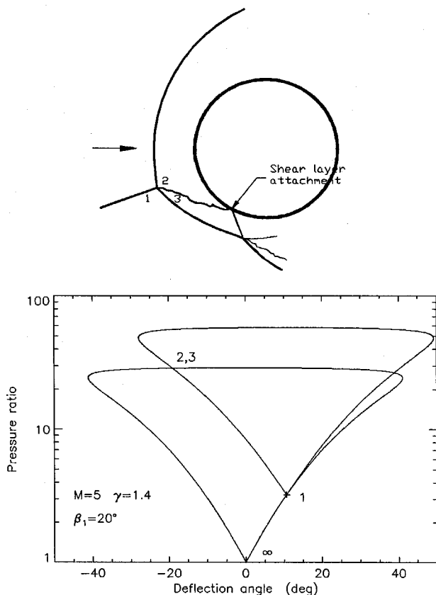
Figure A.5: Schematic of type III interference flow and its representation in the p - \delta plane.
