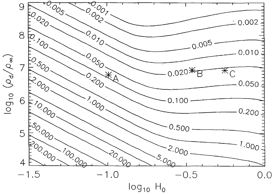
Figure 4.16: CONTOUR PLOT OF THE RECOMBINATION RATE PARAMETER, \Sigma \frac{\zeta_2 \ell_a}{D} , AS A FUNCTION OF DIMENSIONLESS STAGNATION ENTHALPY, H_0 , AND EQUILIBRIUM DENSITY RATIO, \hat{\rho}_d . The contours values are indicated on the plot and the remaining parameters are taken as P = 0 , \alpha_\infty = 0 , \eta = -2.5 . The dependence on P for large Mach numbers is weak. At low enthalpies where the dissociation levels are low the contours asymptote to slope \eta . At higher enthalpies \Sigma is insensitive to H_0 and exhibits an inverse power dependence on \hat{\rho}_d . The three test conditions used for the current experiments are indicated.
