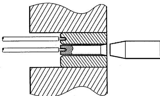
Figure E.2: Layout of new surface junction thermocouple sensor.
