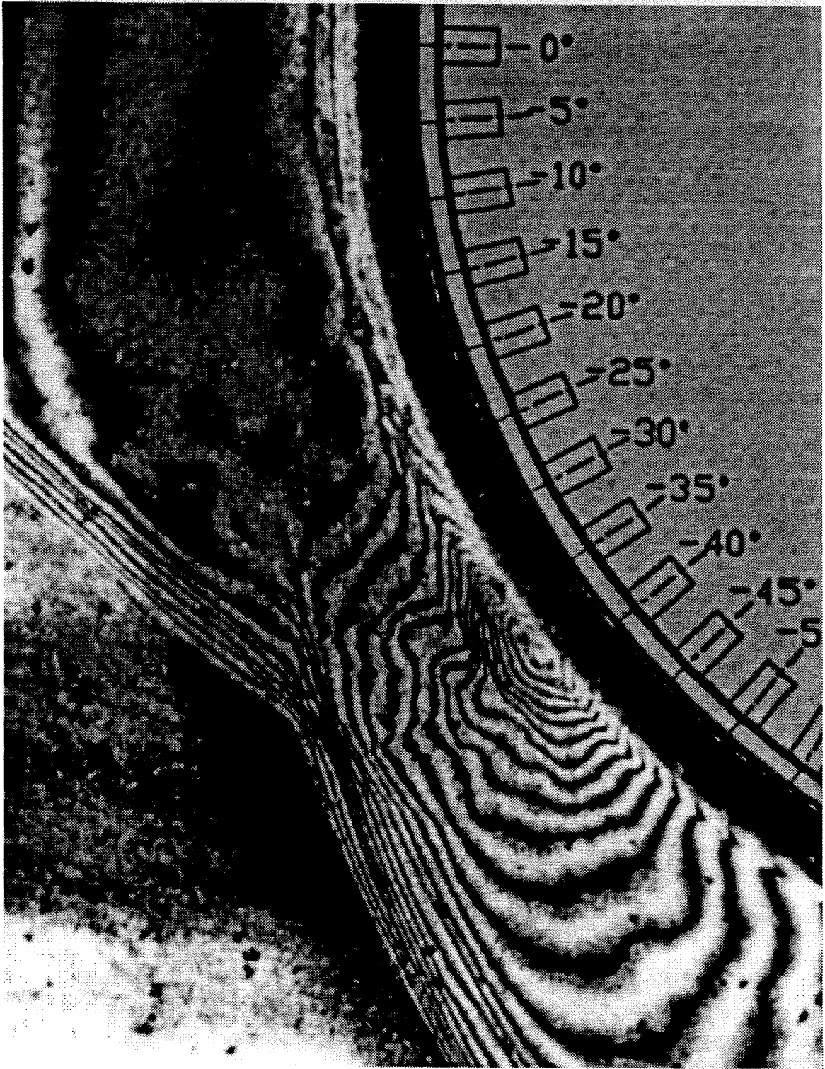
Figure C.29: Magnified view of holographic interferogram; Shot T5-831
