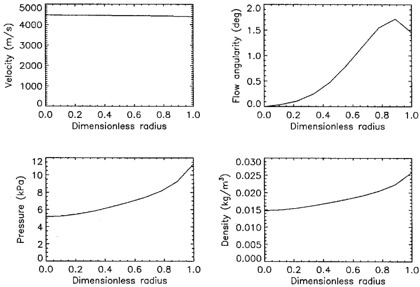
Figure B.2: Flow nonuniformity in the nozzle exit plane for test condition B.
