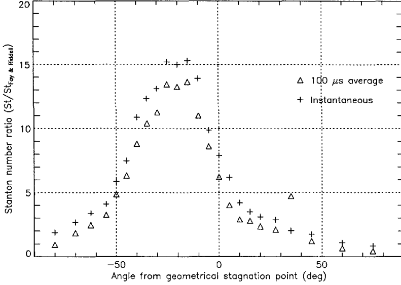
Figure 3.6: ENVELOPE OF MAXIMUM HEAT TRANSFER RATES AROUND THE MODEL AT CONDITION A. The anomalous point at \theta = 35^\circ arises from contributions to the average beyond the ends of the sampling period.
