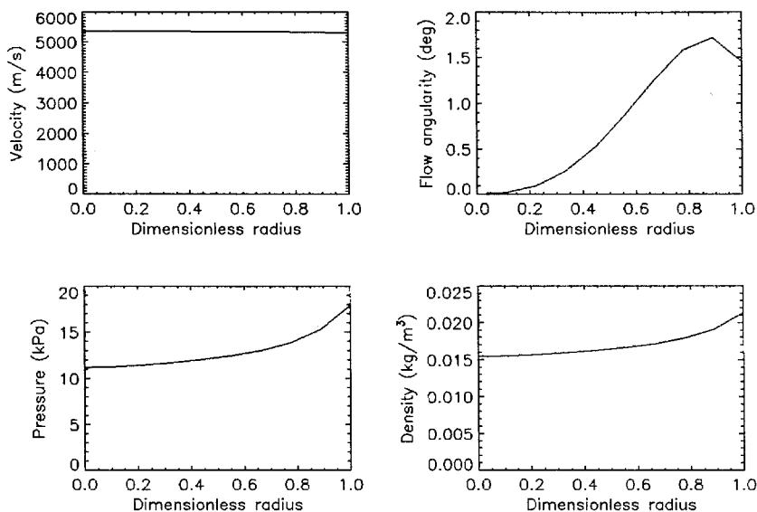
Figure B.3: Flow nonuniformity in the nozzle exit plane for test condition C.
