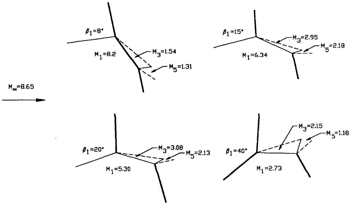
Figure 4.23: VARIATION OF TYPE IV JET SHOCK STRENGTHS WITH IMPINGING SHOCK ANGLE, \beta_1 . Free stream conditions for the frozen solutions are P_\infty = 0.010 , \alpha_\infty = 0 ; \beta_1 = 8^\circ, 15^\circ, 20^\circ, 40^\circ . The shock angles and flow deflection angles shown are to scale.
