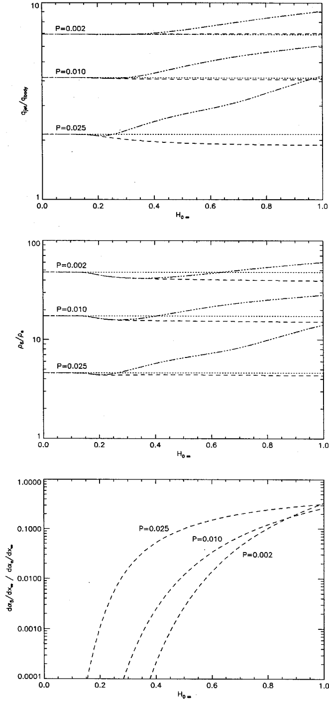
Figure 4.18: INFLUENCE OF DIMENSIONLESS STAGNATION ENTHALPY, H_{0\infty} , MACH NUMBER, \sim 1/\sqrt{P_\infty} AND REACTION RATE ON TYPE IV HEAT TRANSFER INTENSIFICATION. From top: Heat transfer intensification, \frac{\dot{q}_{jet}}{\dot{q}_{body}} \sqrt{\frac{\Delta x}{D} \frac{\zeta_{body}^2 \zeta_{body}}{\zeta_{jet}^2 \zeta_{jet}}} ; stagnation density intensification, \frac{\hat{\rho}_s}{\rho_e} and jet reaction rate ratio, \frac{d\alpha_s/d\alpha_e}{d\alpha_d/d\alpha_e} . . . . . curves are the frozen solutions. — . . . — curves are the equilibrium solutions. --- curves are the nonequilibrium solutions in the limit \frac{d\alpha_1}{d\hat{x}_\infty}, \frac{d\alpha_3}{d\hat{x}_\infty}, \frac{d\alpha_5}{d\hat{x}_\infty} \ll \frac{d\alpha_2}{d\hat{x}_\infty}, \frac{d\alpha_4}{d\hat{x}_\infty}, \frac{d\alpha_6}{d\hat{x}_\infty} . The parameters are P_\infty = 0.002, 0.010, 0.025 , \hat{p}_d = 1 \times 10^7 , \alpha_\infty = 0 and \beta_1 = 16^\circ .
