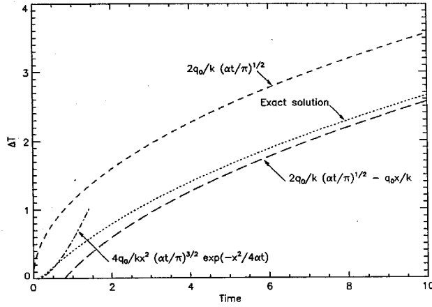
Figure E.1: ASYMPTOTIC BEHAVIOR OF A SURFACE TEMPERATURE SENSOR. For illustrative purposes \alpha = 1 , k = 1 , \dot{q}_0 = 1 , x = 1 .
