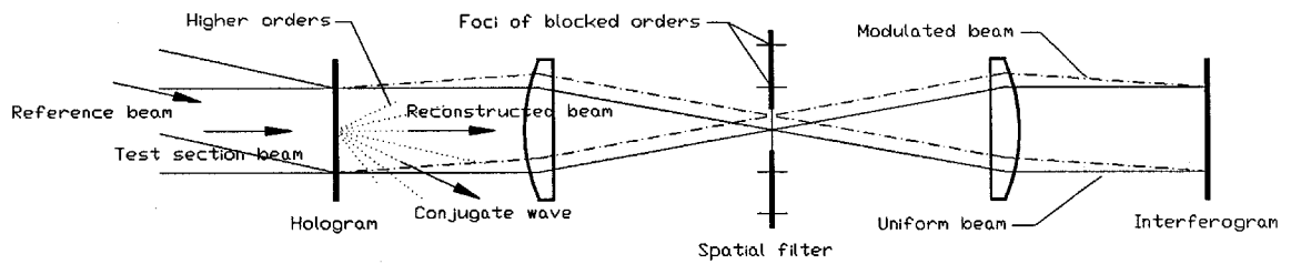
Figure D.2: Geometry of hologram reconstruction and conjugate image separation.
