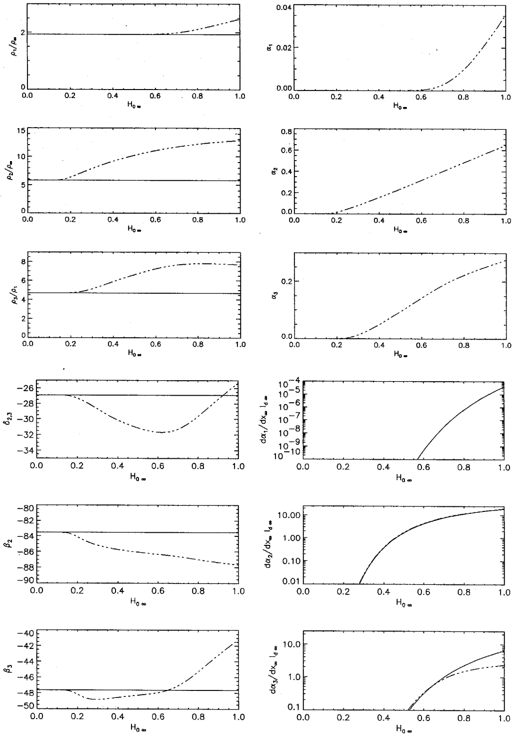
Figure 4.11: DENSITY VARIATIONS, DISSOCIATION LEVELS, SHOCK WAVE ANGLES, STREAMLINE DEFLECTION, AND REACTION RATES AS FUNCTIONS OF STAGNATION ENTHALPY, H_{0\infty} , AT A \lambda -SHOCK POINT IN AN IDEAL DISSOCIATING GAS. The free-stream conditions are P_\infty = 0.025 , \hat{p}_d = 1 \times 10^7 , \alpha_\infty = 0 , \beta_1 = 16^\circ . Solid curves are the frozen solutions. — · · · — are the equilibrium solutions.
