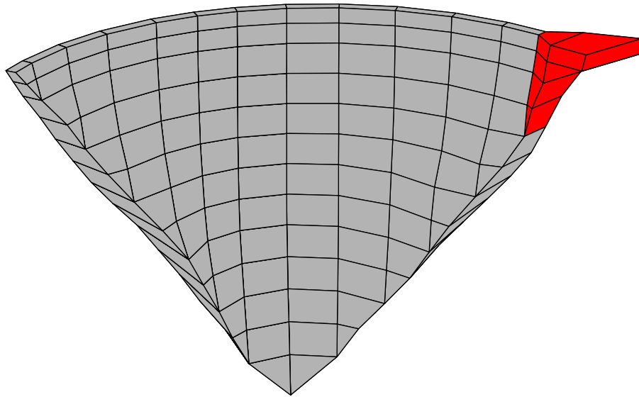
Figure 7.1: Finite element mesh of Pacoima Dam with the thrust block on the left abutment highlighted (viewed from downstream at an elevated vantage)
