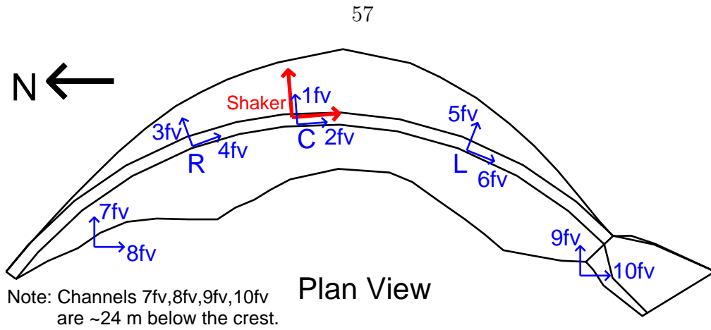
Figure 5.2: Locations of the Rangers and the shaker with orientations
