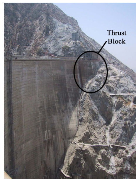
(b) View of left abutment
