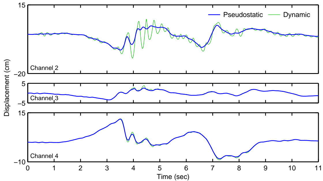
Figure 10.14: Displacement time histories at locations corresponding to channels 2–4 computed from a nonlinear pseudostatic analysis compared to the time histories from a nonlinear dynamic analysis (method 1)
