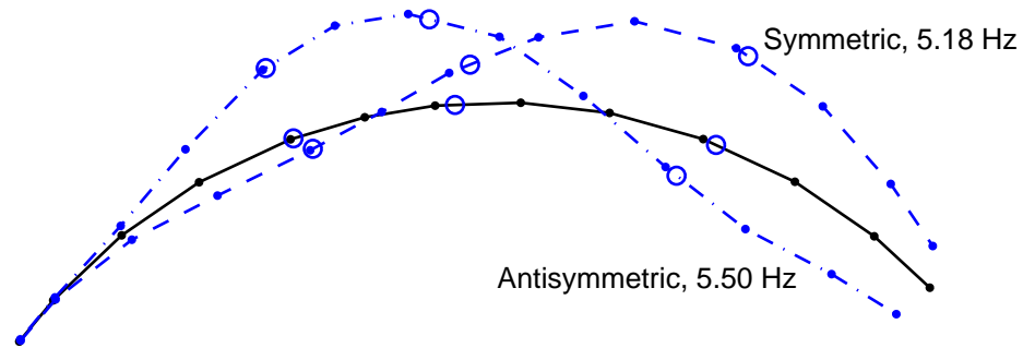
Figure 7.7: Symmetric and antisymmetric mode shapes computed from the linear SCADA model modified to simulate damage with no reservoir, a softened region of foundation and an open joint (The open circles are the locations of the crest level stations and the dots are the locations of the nodes on the crest.)
