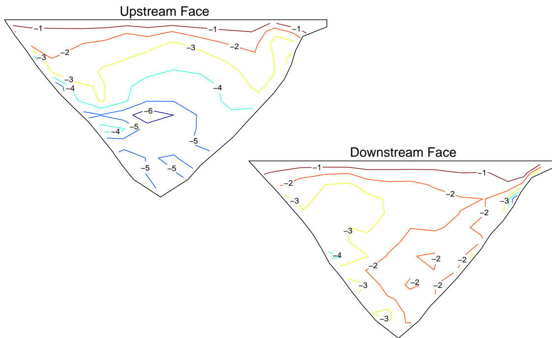
Figure C.24: Maximum compressive cantilever stresses (MPa) computed during a nonlinear analysis with the Northridge earthquake input (method 2)
