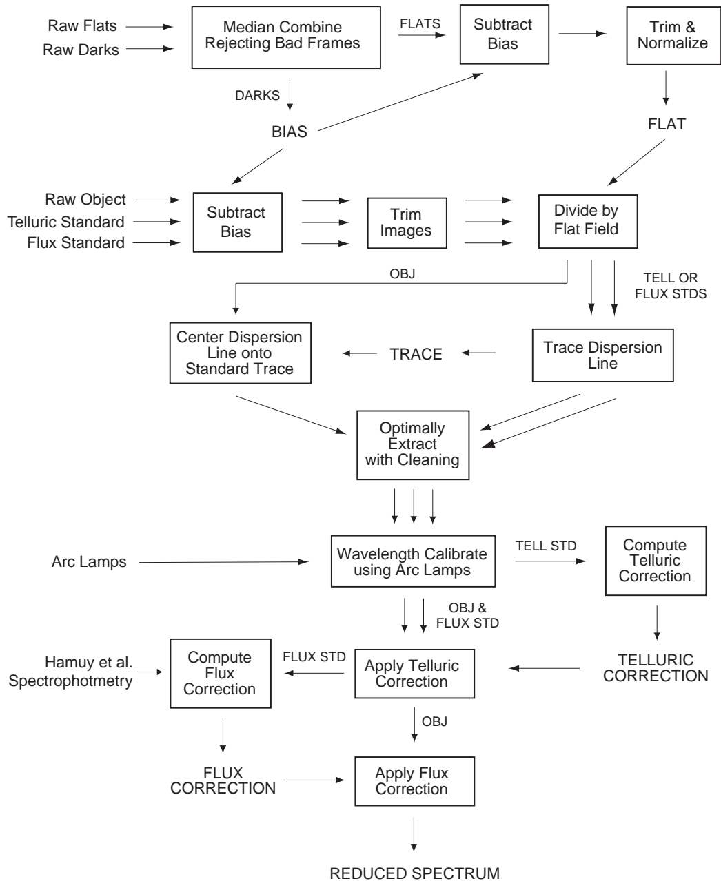
Figure 3.17: A flowchart diagramming the procedures for LRIS spectral data reduction. This algorithm was implemented in the IRAF environment using the APEXTRACT package.
