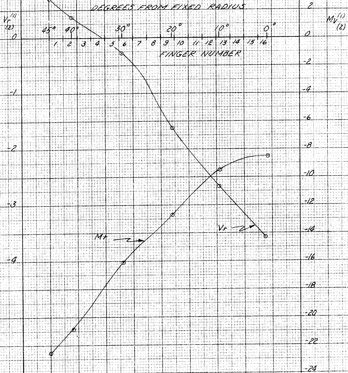
FIG. 6 ARC BOUNDARY LOADING CONDITION NO. 1 M_r \sim INCH POUNDS PER INCH V_r \sim POUNDS PER INCH P_c = 14.58 POUNDS
