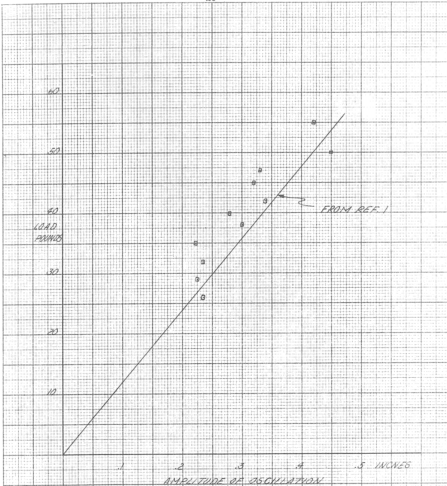
FIG. 1 COMPARISON OF AMPLITUDE OF OSCILLATION WITH STATIC AMPLITUDE COMPUTED USING EI OF REF. 1 SQUARE PATTERN
