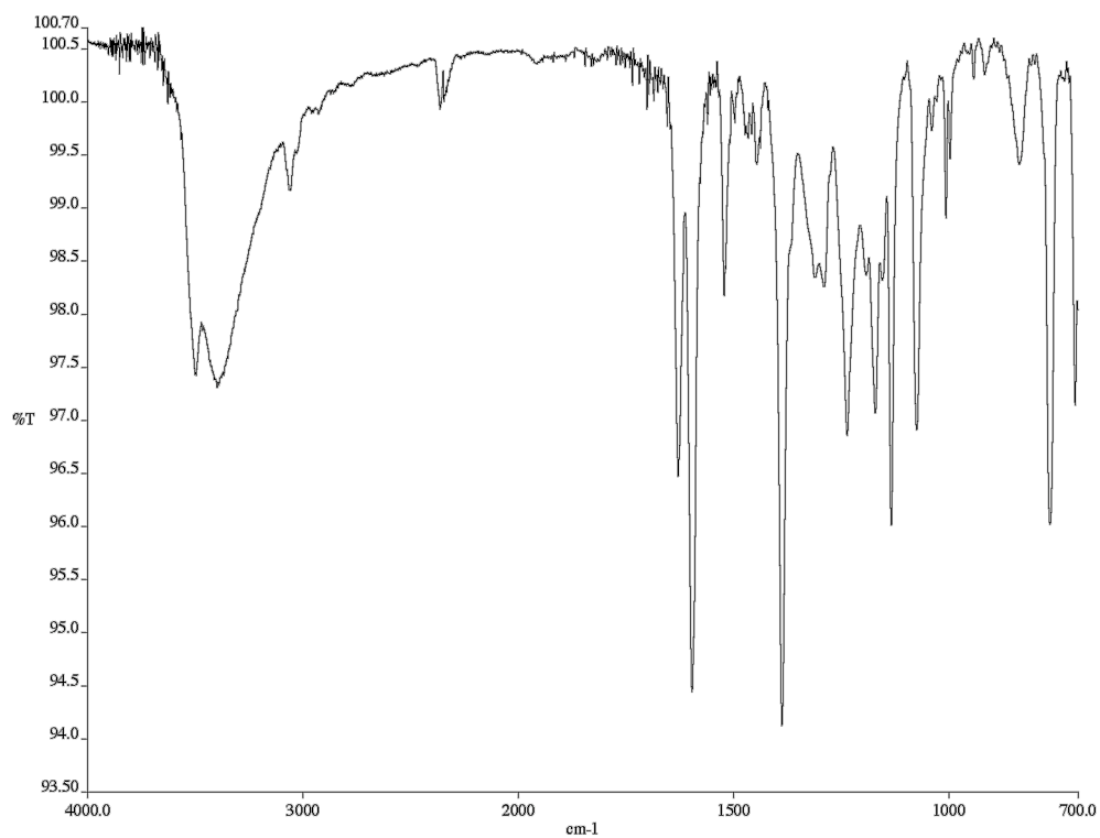
Figure A7.8 Infrared spectrum (thin film/NaCl) of compound 334 .
