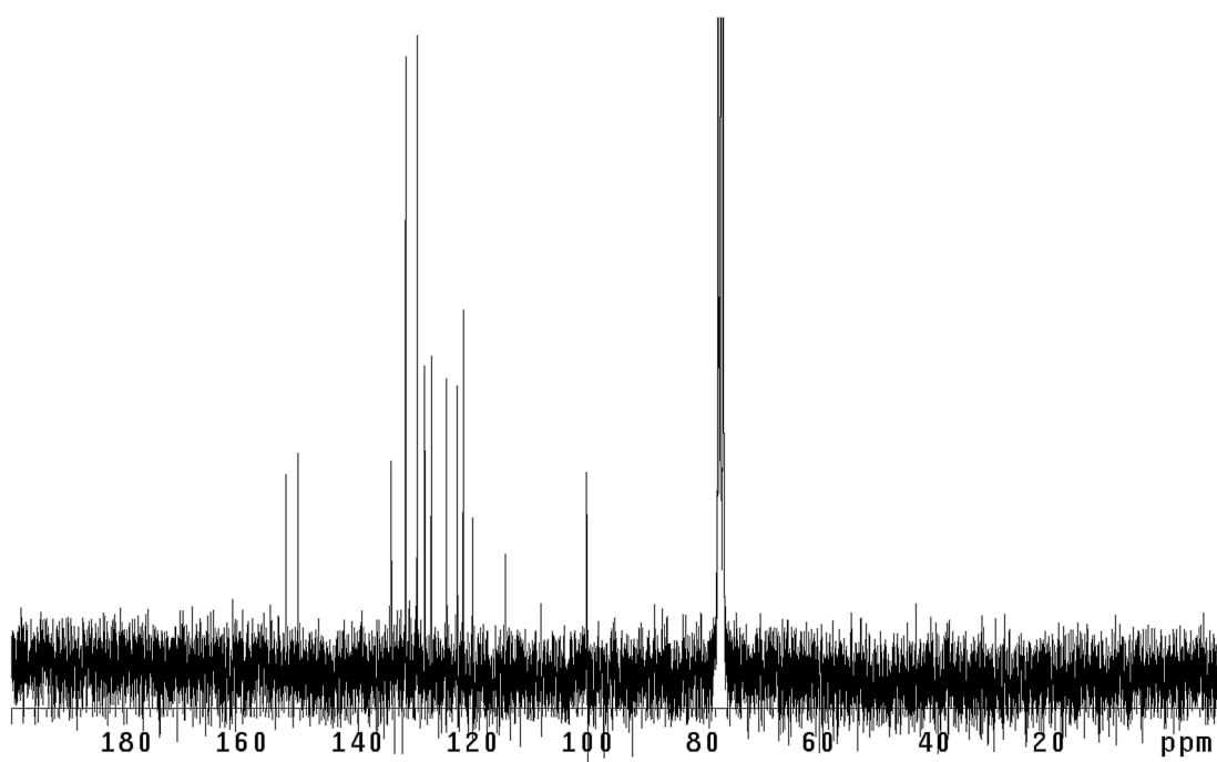
Figure A7.9 13 C NMR (75 MHz, CDCl 3 ) of compound 334 .
