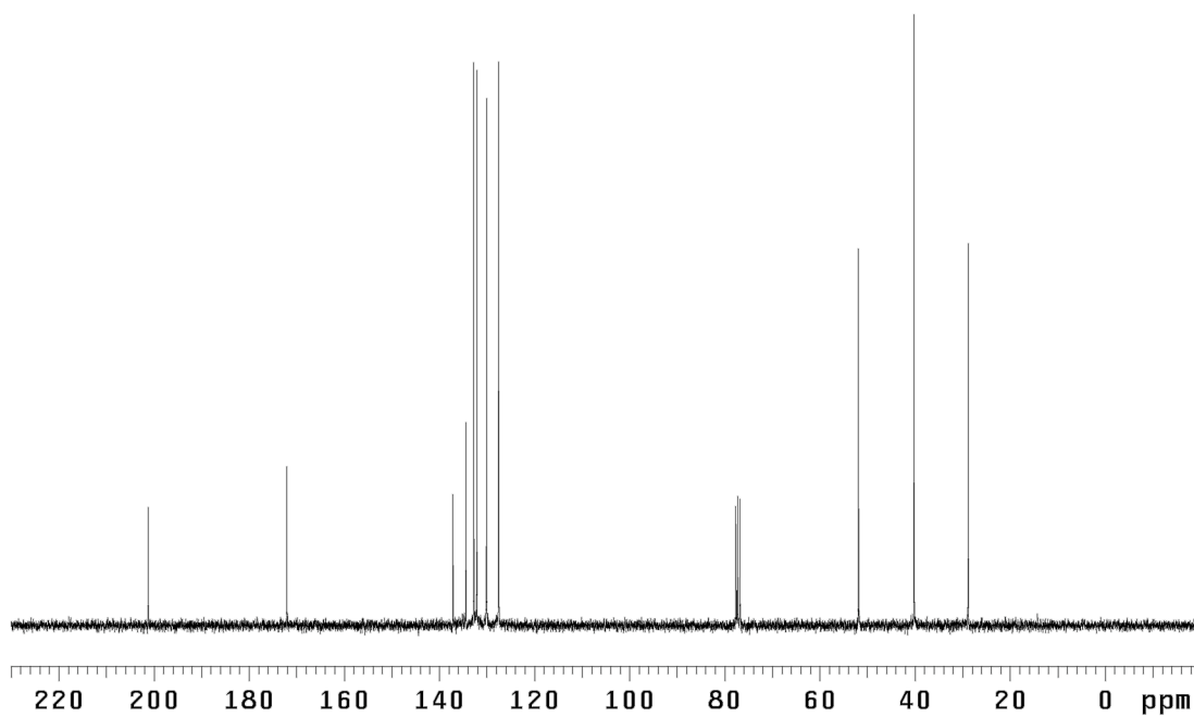
Figure A7.3 13 C NMR (75 MHz, CDCl 3 ) of compound 327 .
