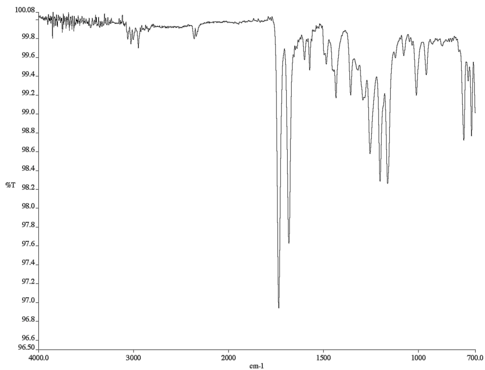
Figure A7.5 Infrared spectrum (thin film/NaCl) of compound 330 .
