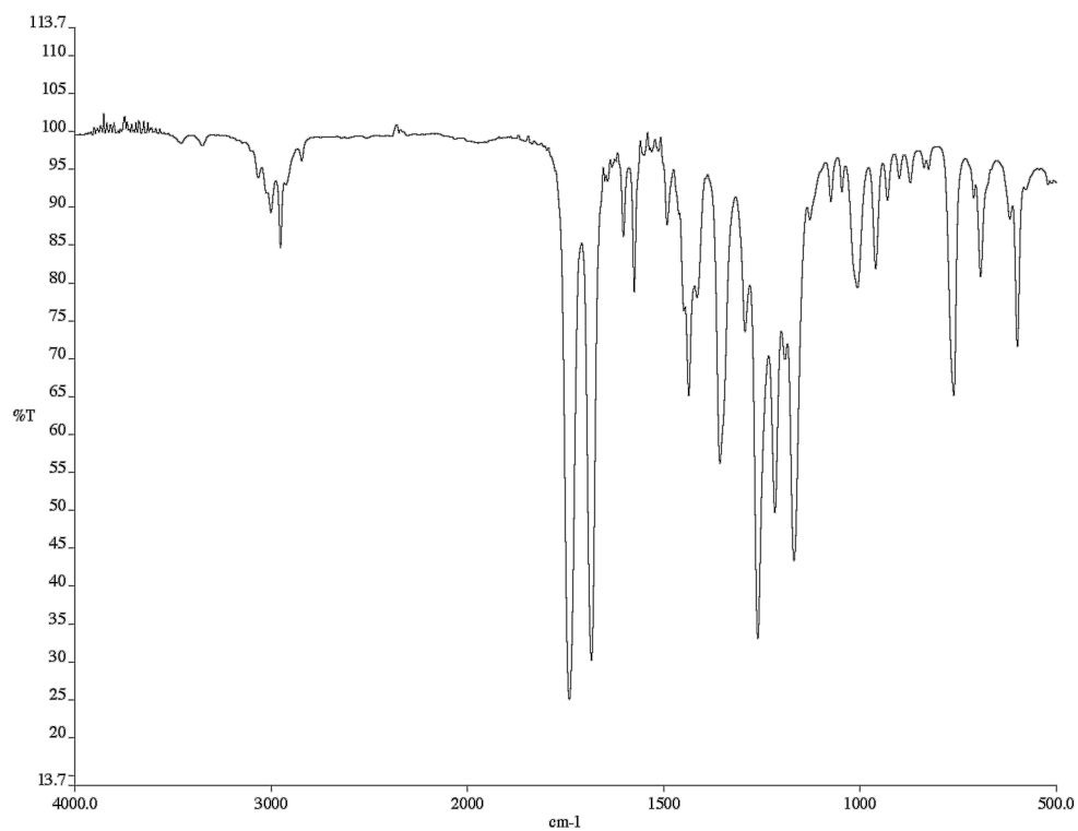
Figure A7.2 Infrared spectrum (thin film/NaCl) of compound 327 .
