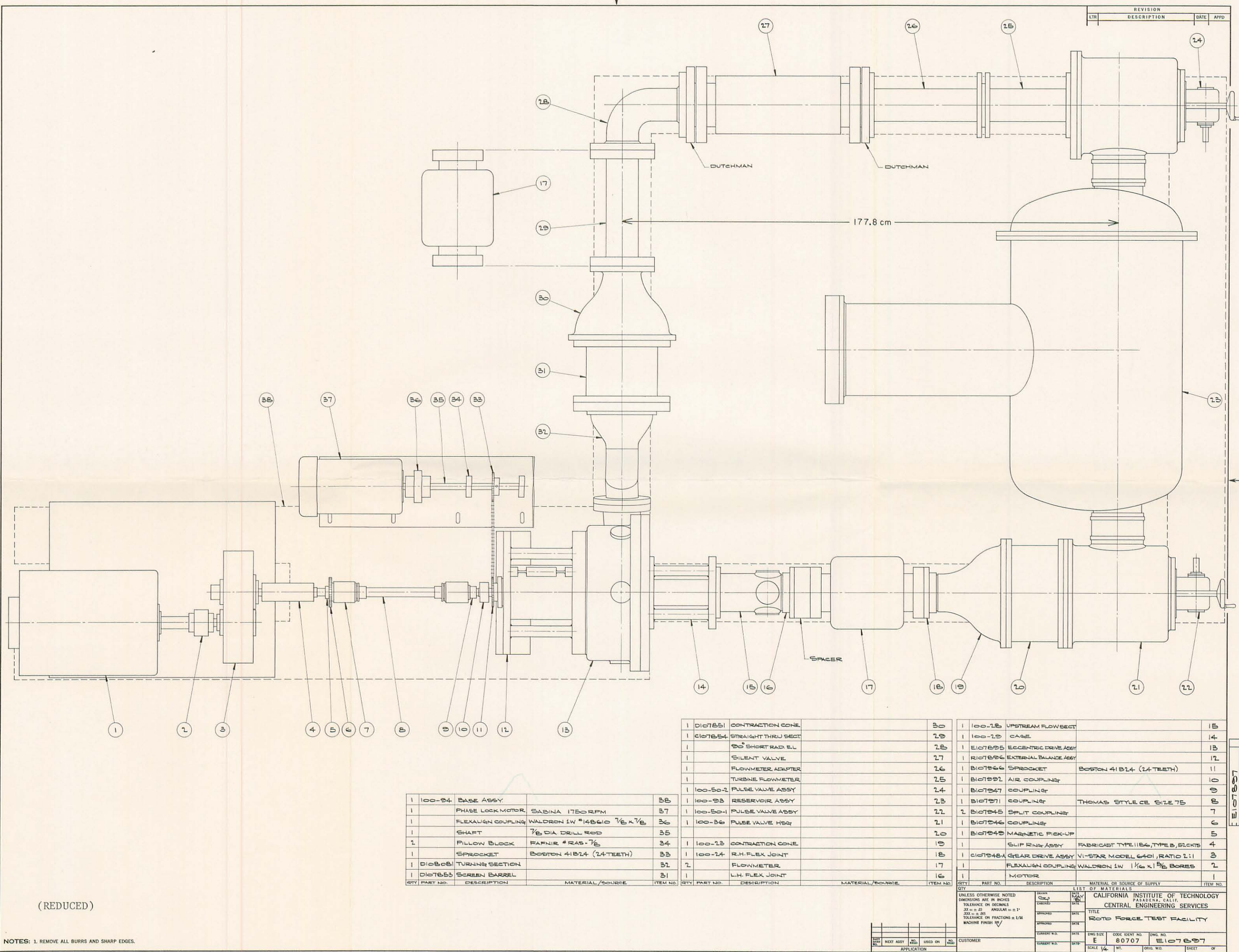
Fig. 2.3. The Dynamic Pump Test Facility after the addition of the Rotor Force Test Facility.
