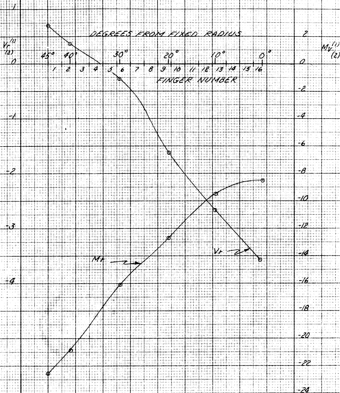
FIG. 6 ARC BOUNDARY LOADING CONDITION NO. 1 M_v \sim INCH POUNDS PER INCH V_r \sim POUNDS PER INCH P_c = 14.58 POUNDS
