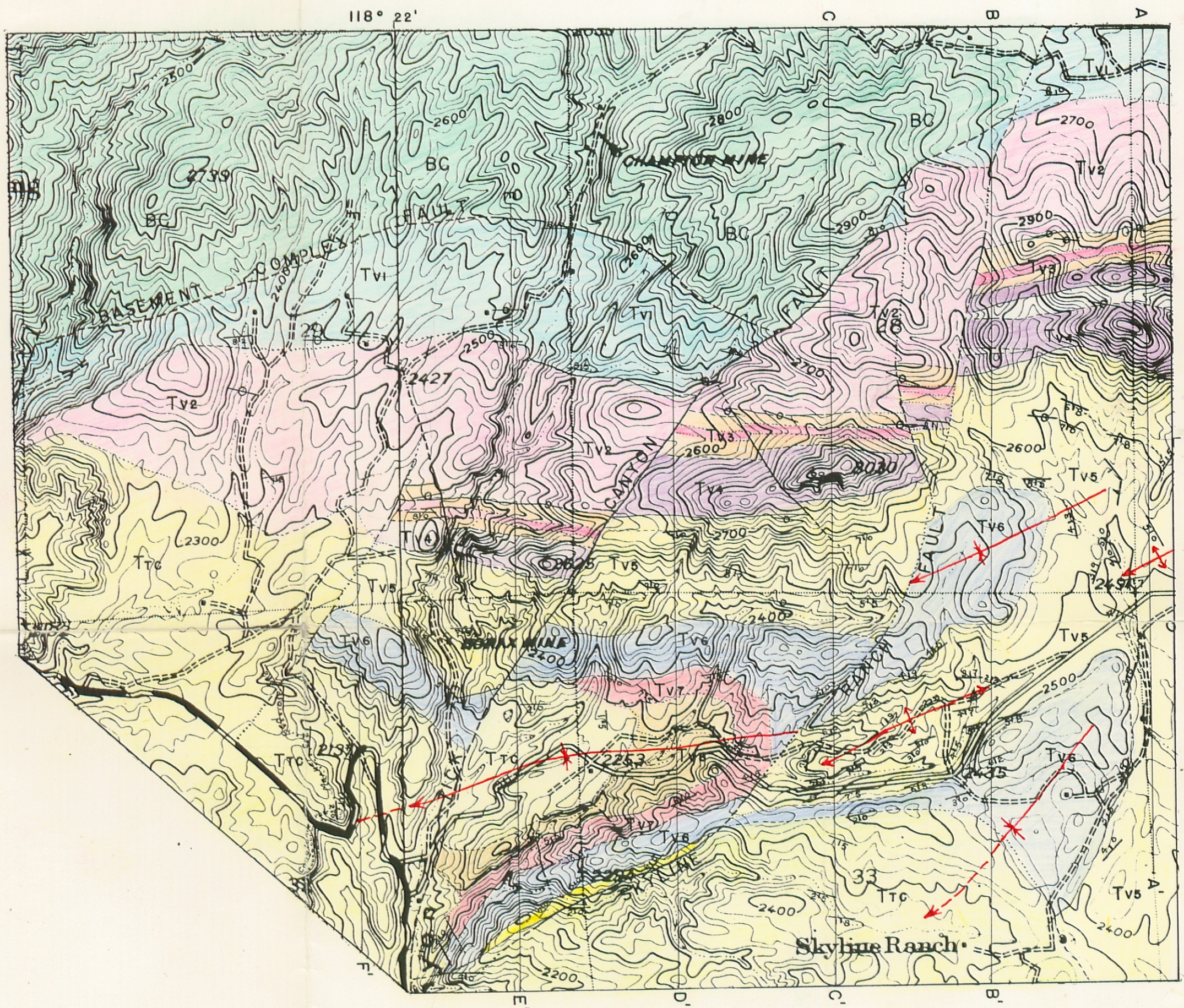
PRE-QUATERNARY GEOLOGY OF THE UPPER TICK CANYON AREA, LOS ANGELES COUNTY, CALIFORNIA.
