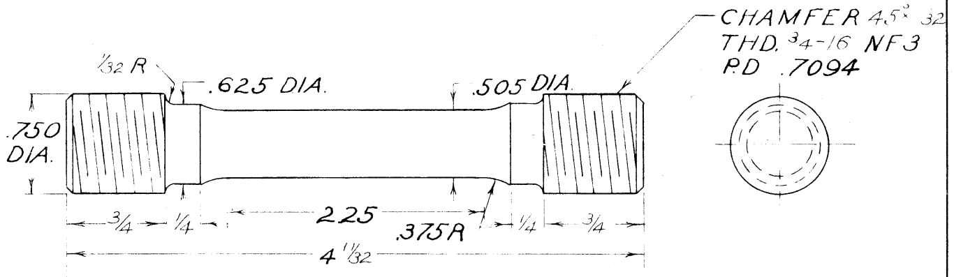
Tension Specimen
