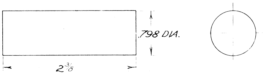
Compression Specimen
