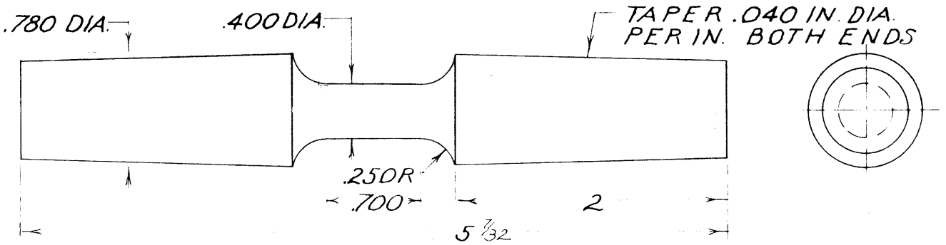
Fatigue Specimen
