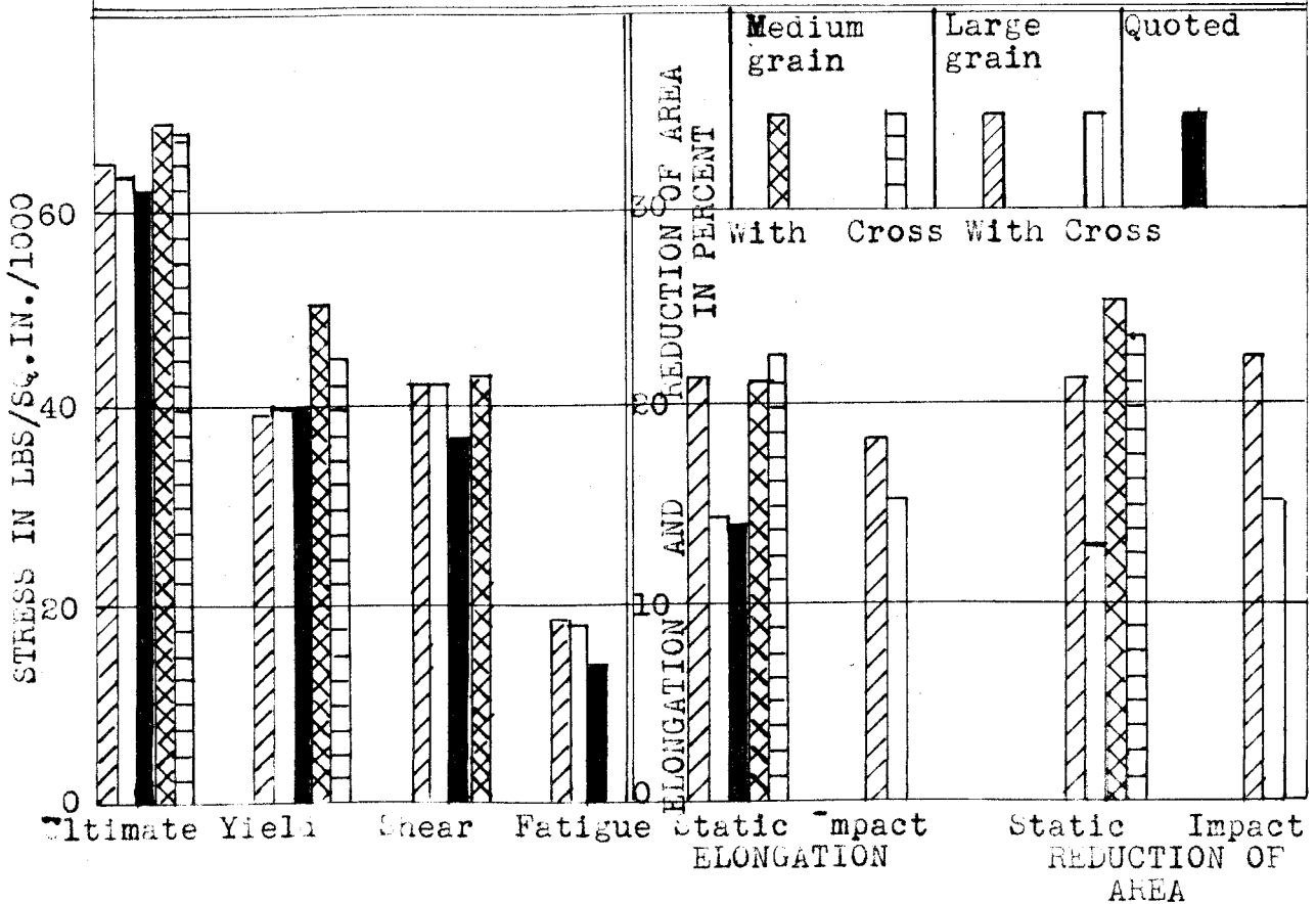
STRENGTH COMPARISONS
