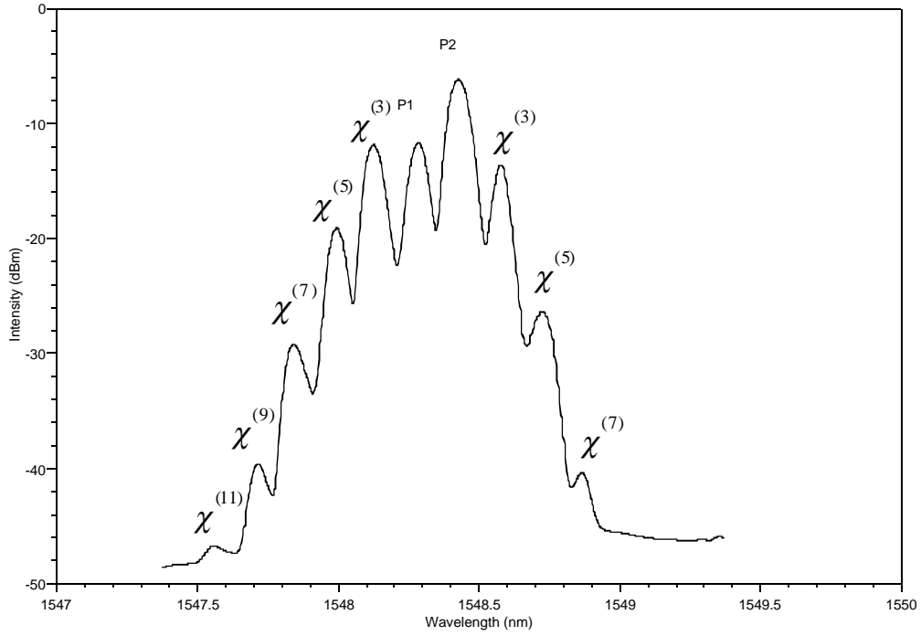
Figure 3.3: Many cascaded FWM processes can occur due to high nonlinearity in a SOA when two waves P1 and P2 are launched
