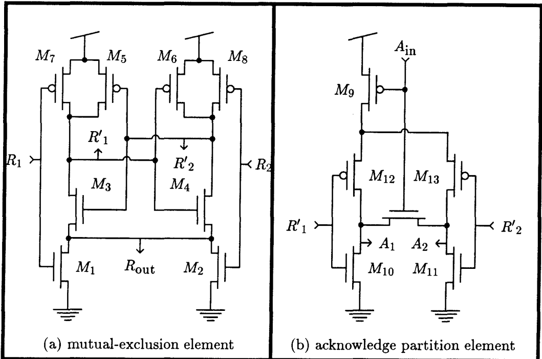
Figure 6.28: The 2-input arbiter cell.
