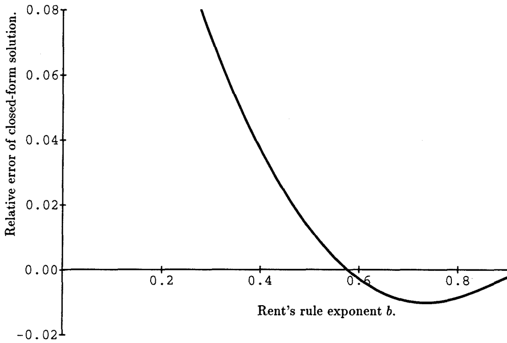
Figure 3.7: Relative error introduced by integrating model from \tau = 0 . This curve is computed from numerical integration of Equation 3.18 and comparison to the closed form expression of Equation 3.19. This error is independent of \gamma .
