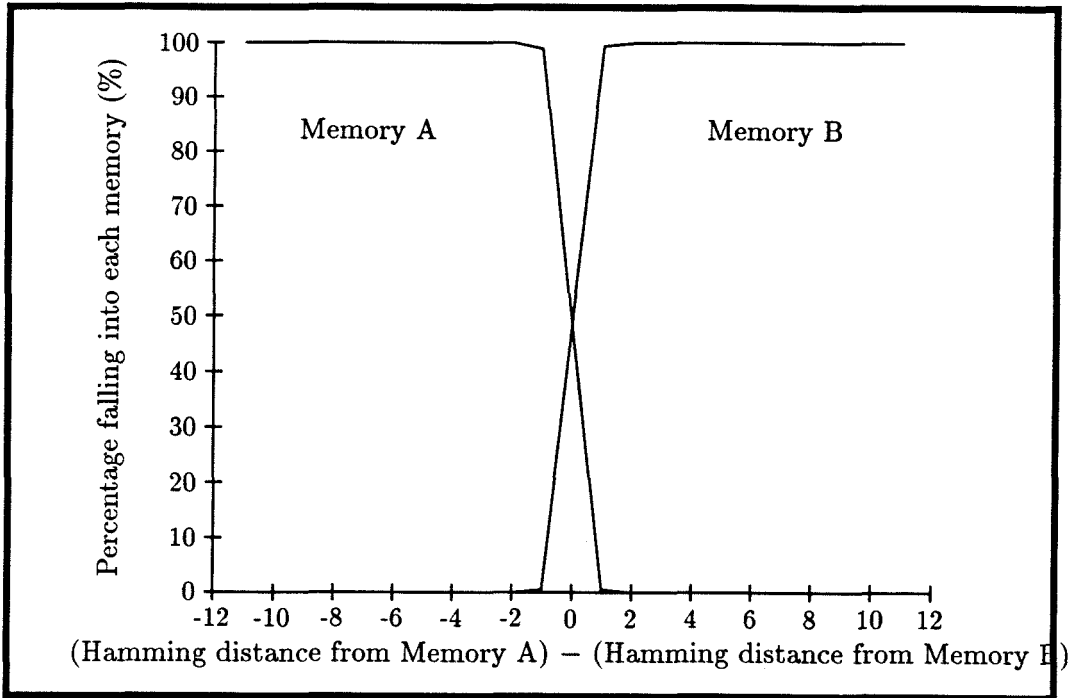
Figure 2.16: ASSOCMEM convergence properties.
