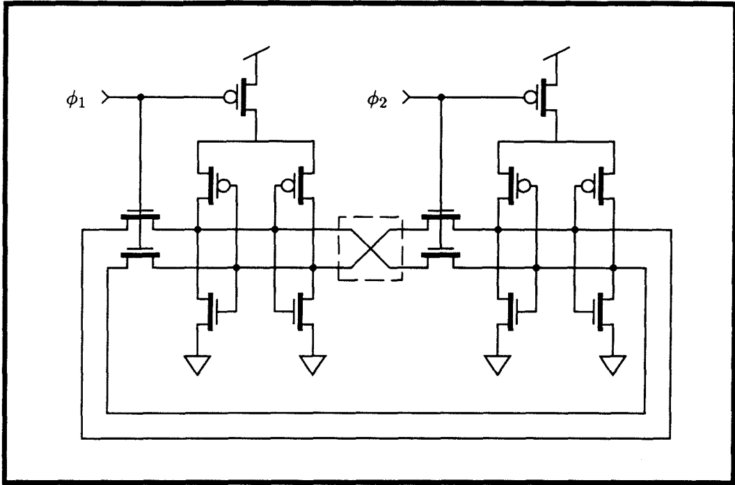
Figure 5.11: If the crossover indicated by the hatched line is absent, this CSRL [MW85] 1-bit counter becomes a latch! Unfortunately, the high degree of symmetry of this circuit make this difficult to detect. Typically, an error is reported at all four pass transistors, as well as their source / drain nodes.
