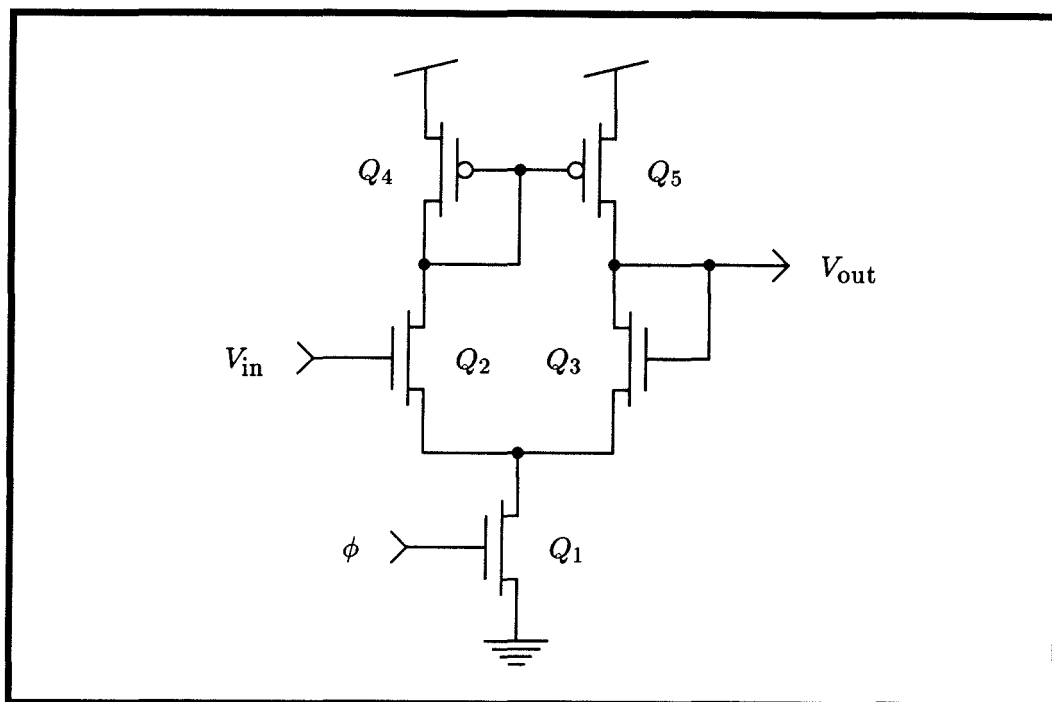
Figure 6.6: Low-noise sample-and-hold circuit.
