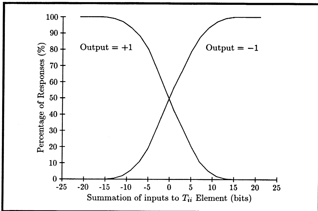
Figure 2.13: T_{ii} transfer characteristic.
