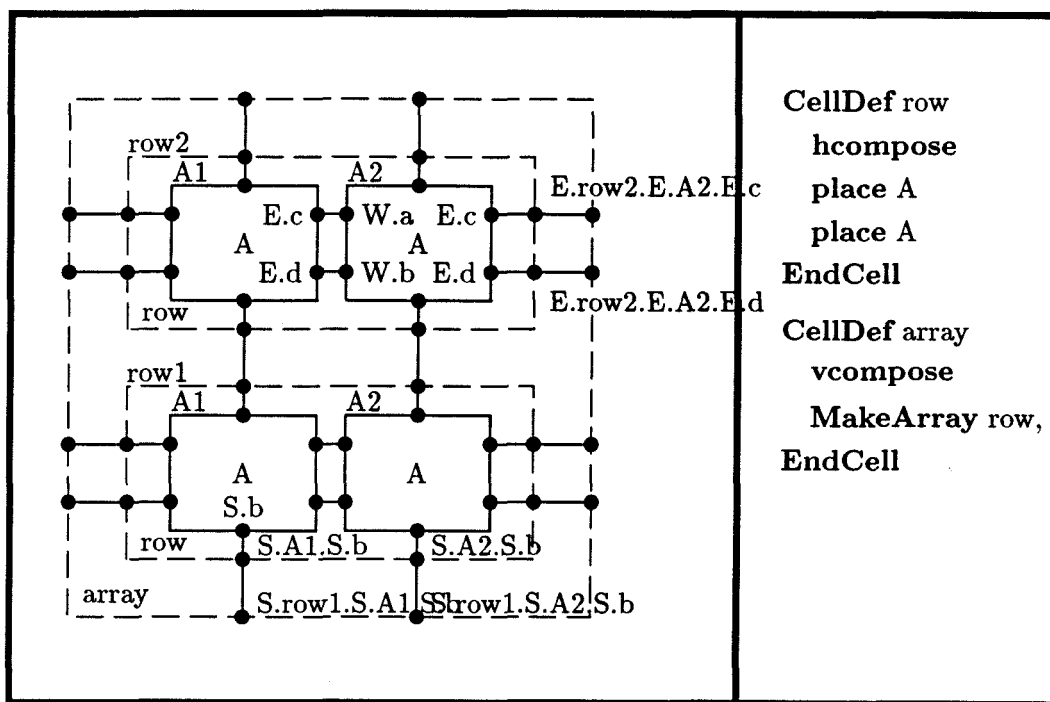
Figure 5.3: Using the NETGEN place operator to connect a row of cells. A direction of cell placement is specified by hcompose / vcompose. The MakeArray operator is simply a shorthand operator for multiple calls to place.
