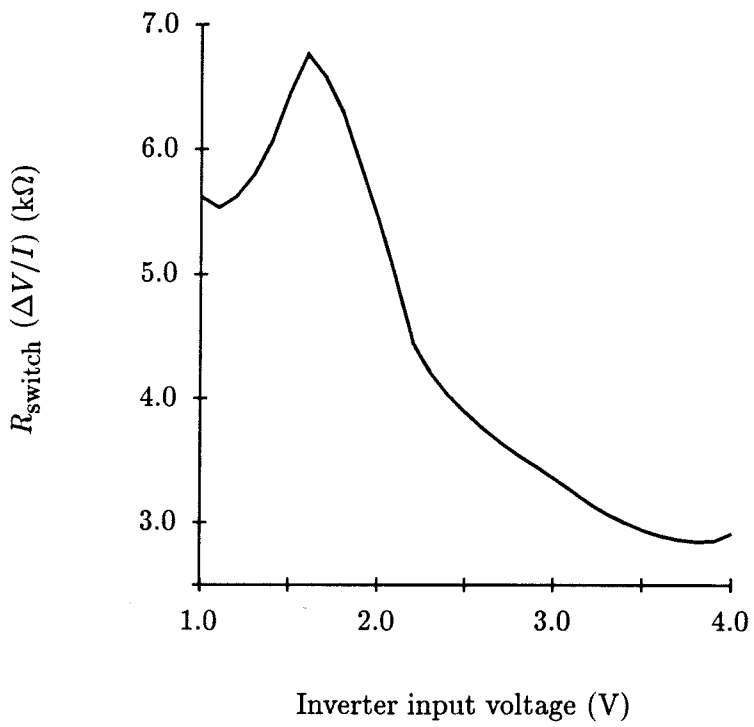
Figure 4.20: Effective large-signal resistance of transmission gates in Figure 4.18.
