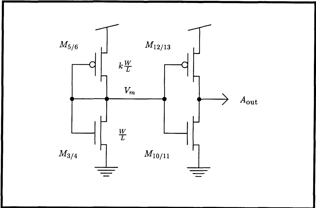
Figure 6.29: Equivalent circuit for arbiter in metastable state.
