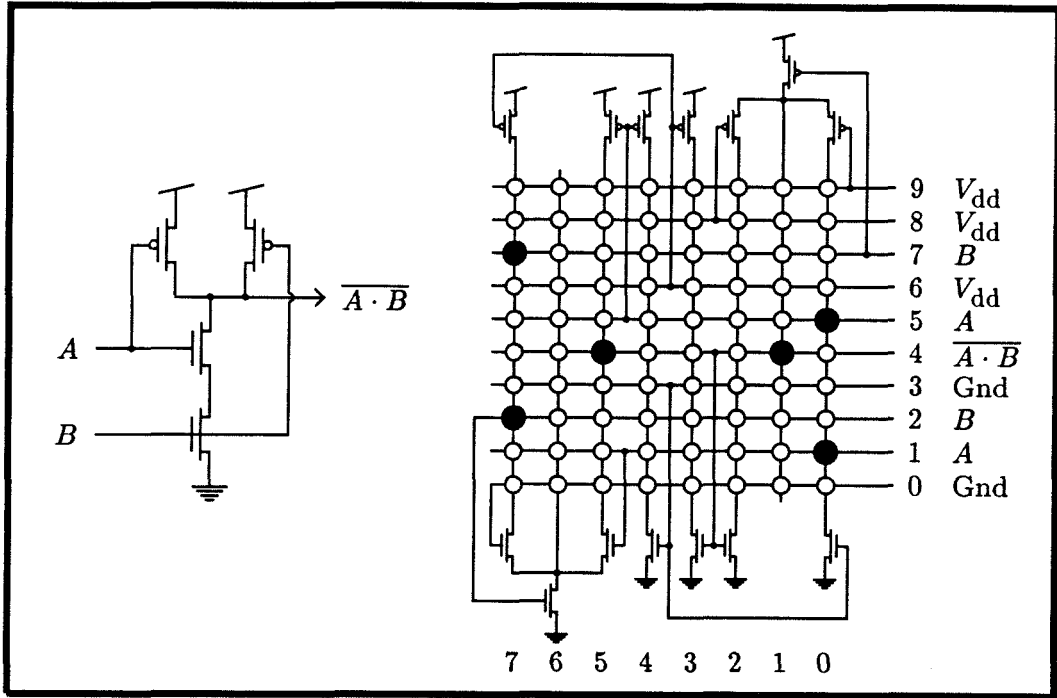
Figure 4.12: NAND gate implemented with analog leaf.
