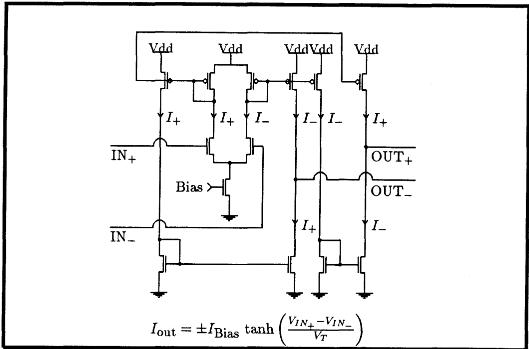
Figure 2.20: Subthreshold CMOS active element.
