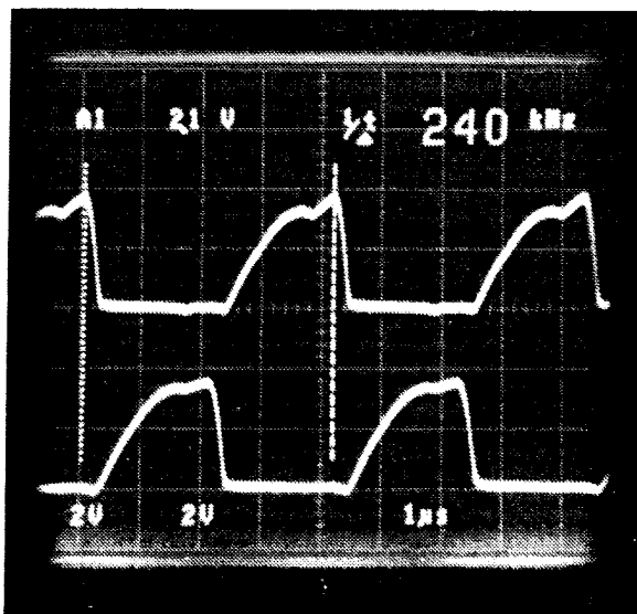
Figure 2.14: Ring oscillator.
