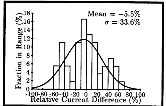
Figure 2.4: Drain current variation in adjacent 24 \times 24 \mu MOS transistors.
