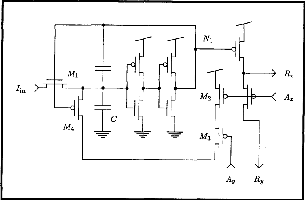
Figure 6.26: Delta-modulation cell.
