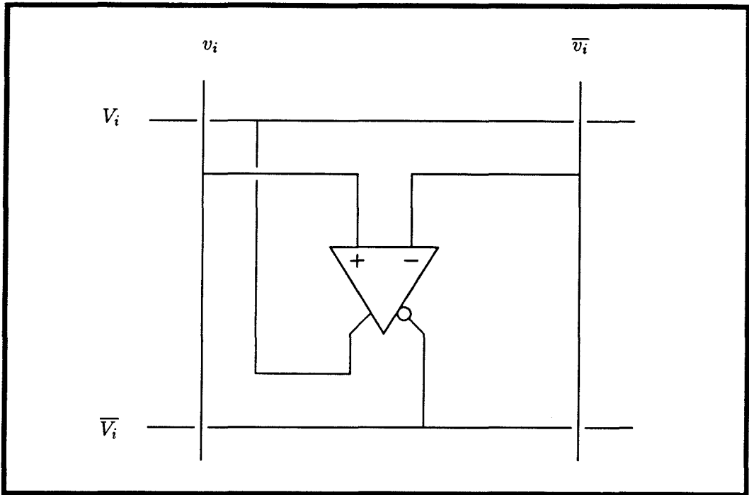
Figure 2.6: Dual-rail signal representation.
