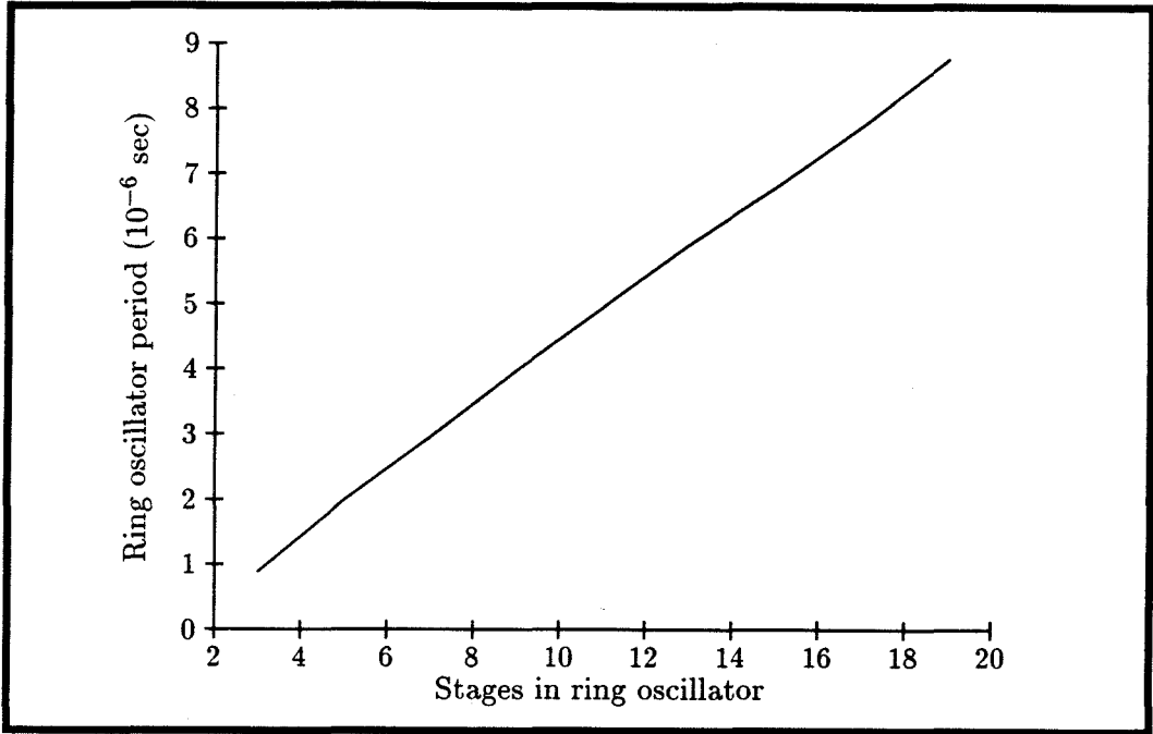
Figure 2.15: Ring oscillator periods.
