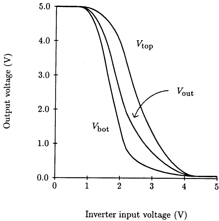
Figure 4.19: Transfer curve for inverter in Figure 4.18. A non-negligible voltage drop across each transmission gate is clearly visible.
