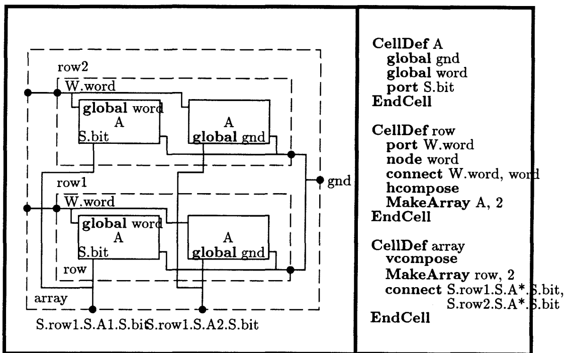
Figure 5.4: Dynamic scoping of identifiers.
