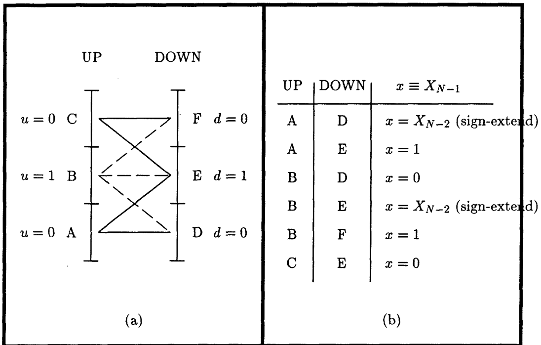
Figure 6.19: Synthesis of an up-down counter from two up-counters. We can interpret the difference between two up-counters uniquely, if we also keep track of in which subrange ( u = \{0, 1\}, d = \{0, 1\} ) the two up-counters are operating. In the worst case, the dynamic range of the synthesized difference output is [-M, M] , corresponding to (N - 1) bits of precision.
