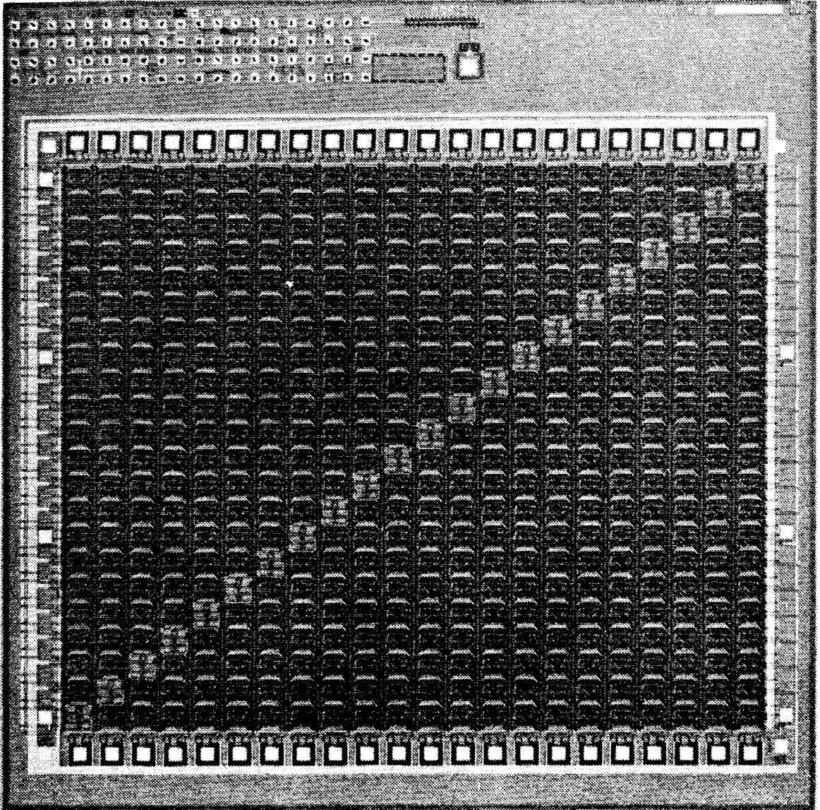
Figure 2.12: The ASSOCMEM.
