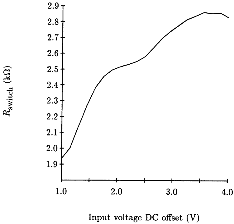
Figure 4.16: Transmission gate small-signal resistance. The experimental data describe the small-signal resistance of a scaled transmission gate. Unfortunately, we did not compensate for the shortening of the channel due to diffusion of the source-drain implants under the gate.
