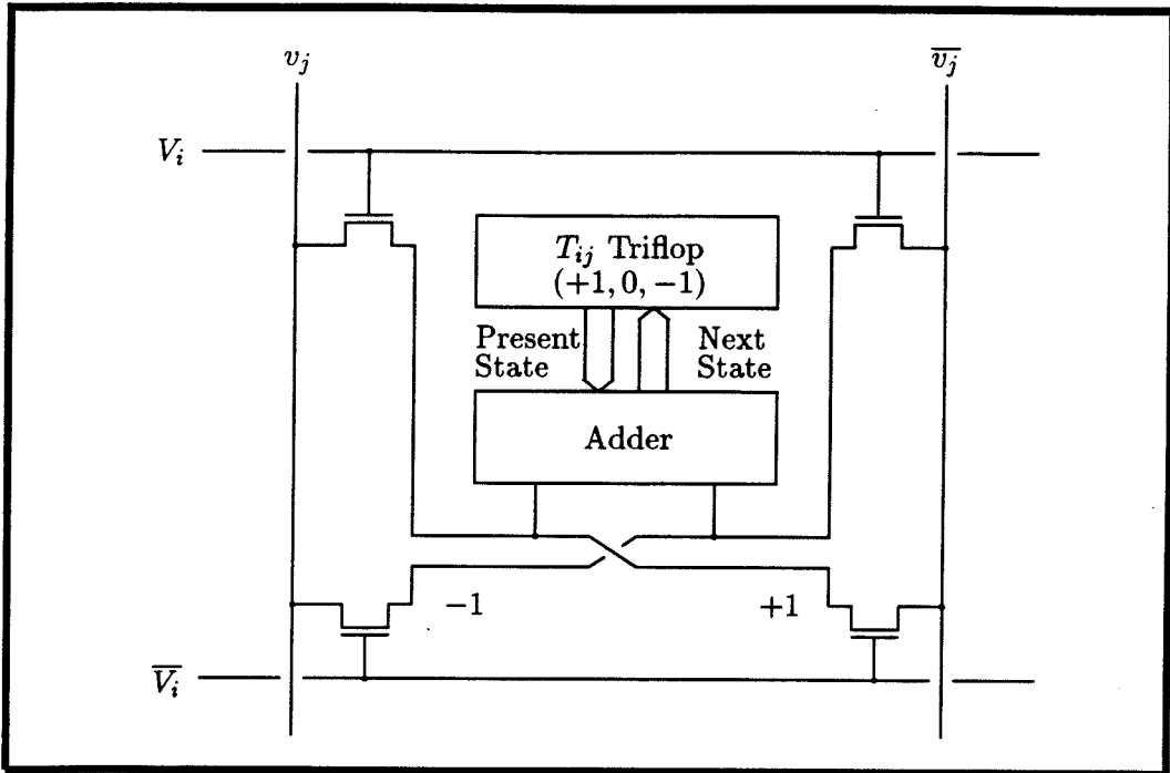
Figure 2.10: Programming the T_{ij} matrix.
