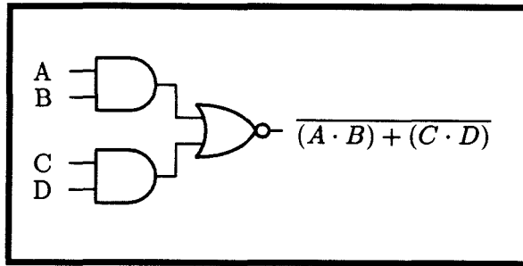
Figure 5.12: A typical and-or-invert (AOI) gate. Here, pins A and B are logically interchangeable, as are pins C and D.
