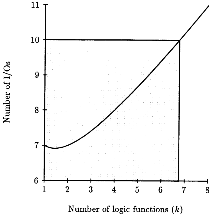
Figure 4.13: Tradeoff between inputs and outputs in digital leaf.
