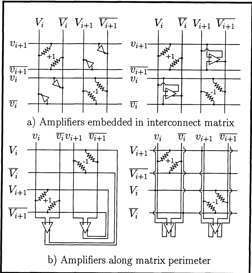
Figure 2.19: Fully-connected associative memory layout strategies.
