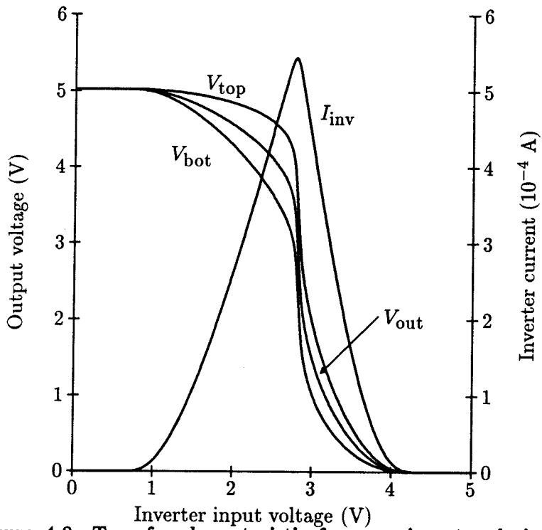
Figure 4.8: Transfer characteristic for poor inverter design of Figure 4.18. The inverter has two diffusion switches in series with high-current path.
