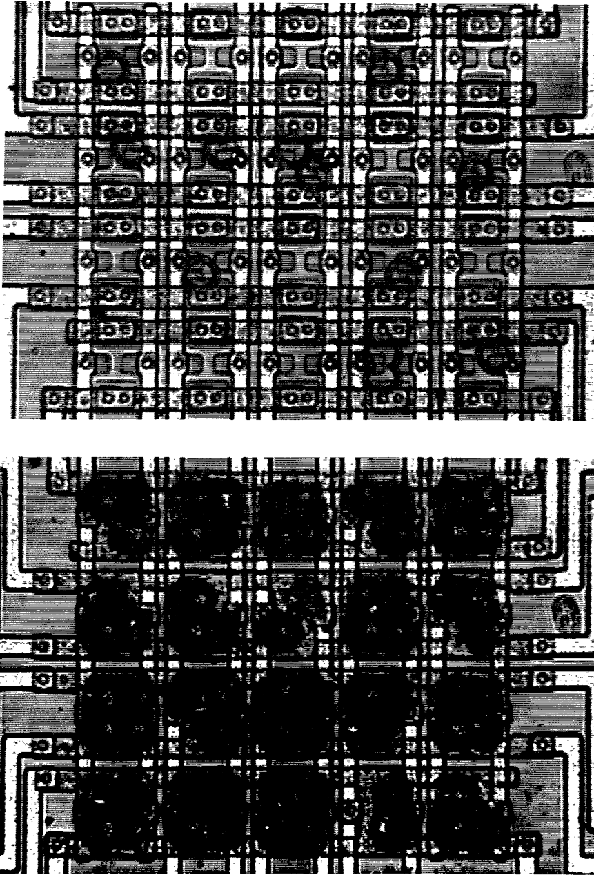
Figure 4.7: Photographs of laser-programmed interconnect matrix. The upper photograph shows the laser-controlled linking of adjacent diffusion areas; the lower photograph shows the same interconnect matrix, obtained by cutting metal lines.
