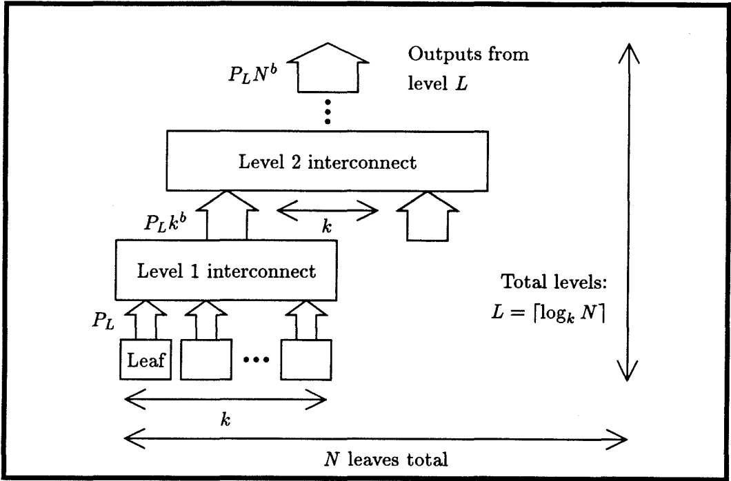
Figure 4.2: Hierarchical interconnect parameters.
