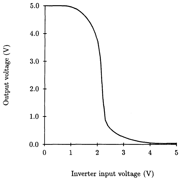
Figure 4.21: Transfer curve for an inverter designed with no transmission gates in series with high-current path.
