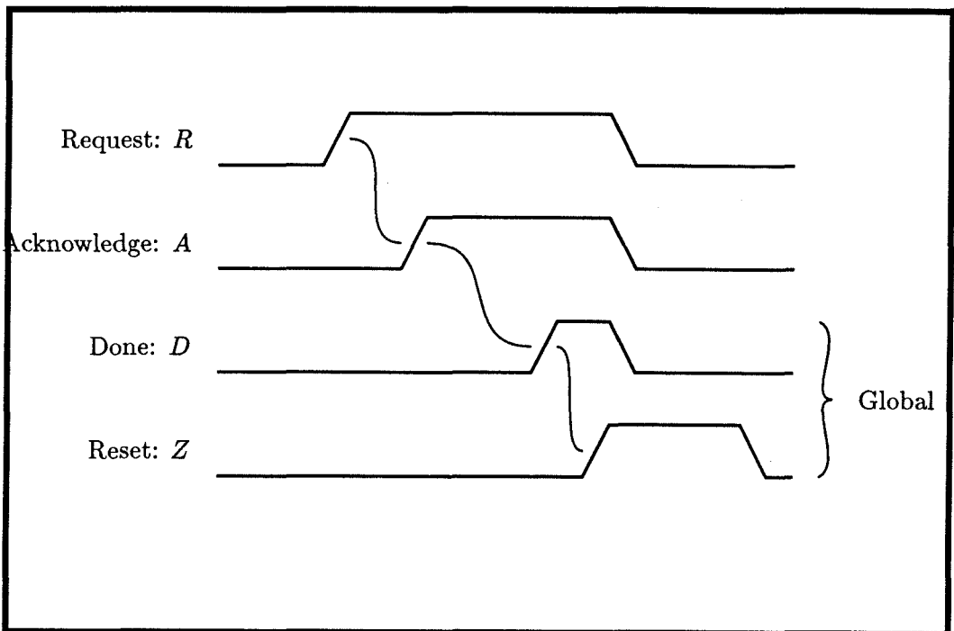
Figure 6.24: The self-timed retina asynchronous communication protocol.
