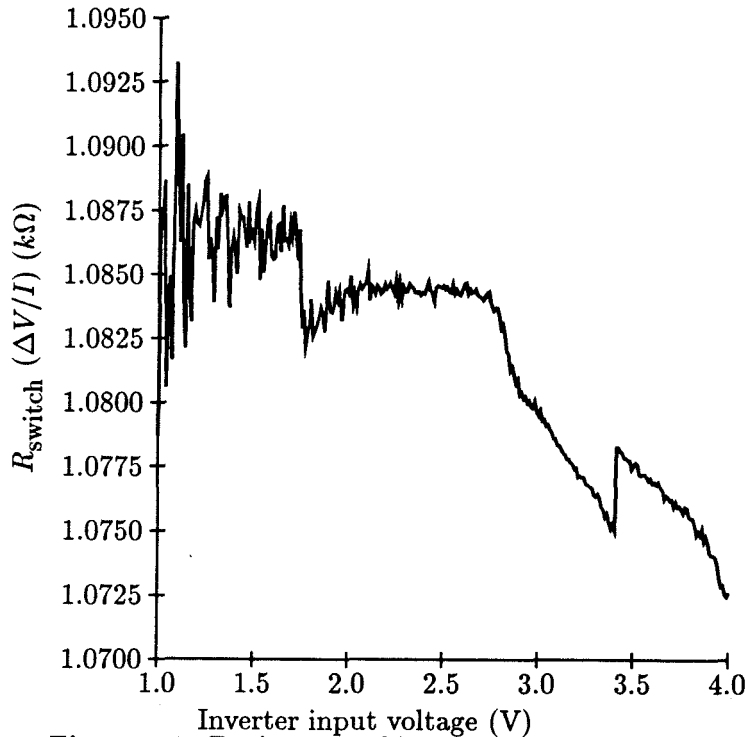
Figure 4.9: Resistance of laser-programmed link.
