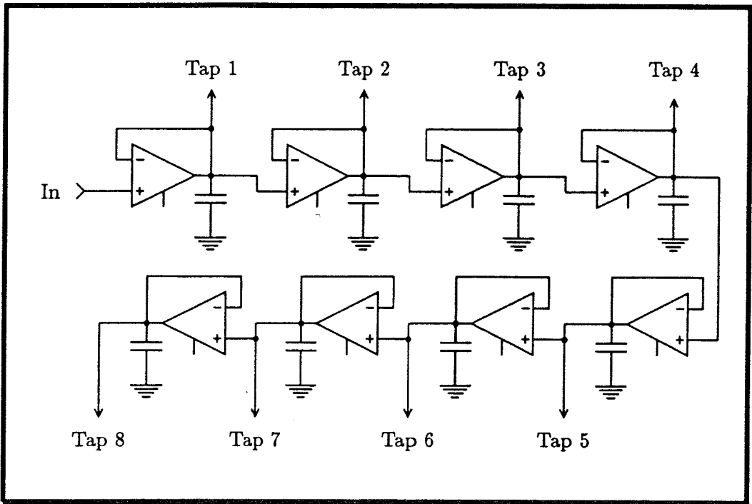
Figure 4.22: A follower-integrator delay line constructed of first-order sections (see [Mea89]).
