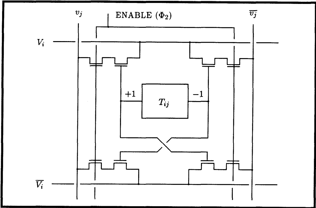
Figure 2.9: Resistive interconnect.
