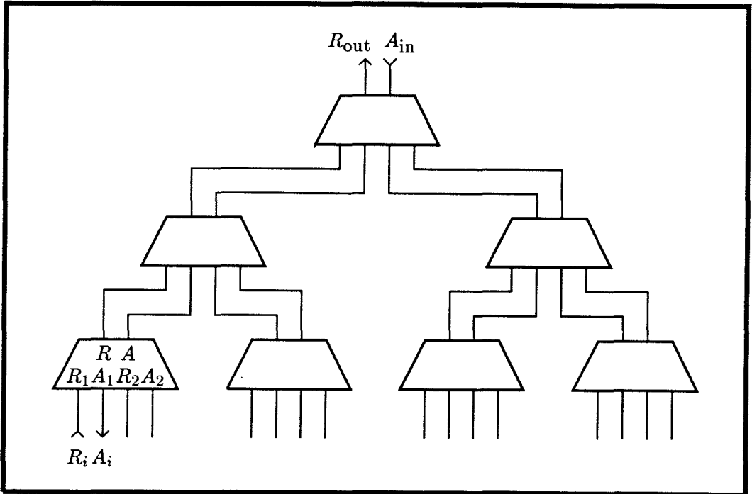
Figure 6.27: Binary tree of 2-input arbiters.
