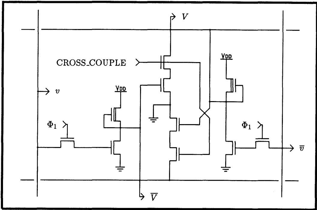
Figure 2.8: T_{ii} element schematic.
