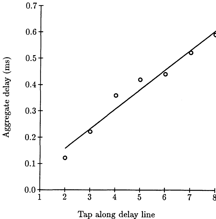
Figure 4.23: Waveform delay as a function of distance down the delay line of Figure 4.22.
