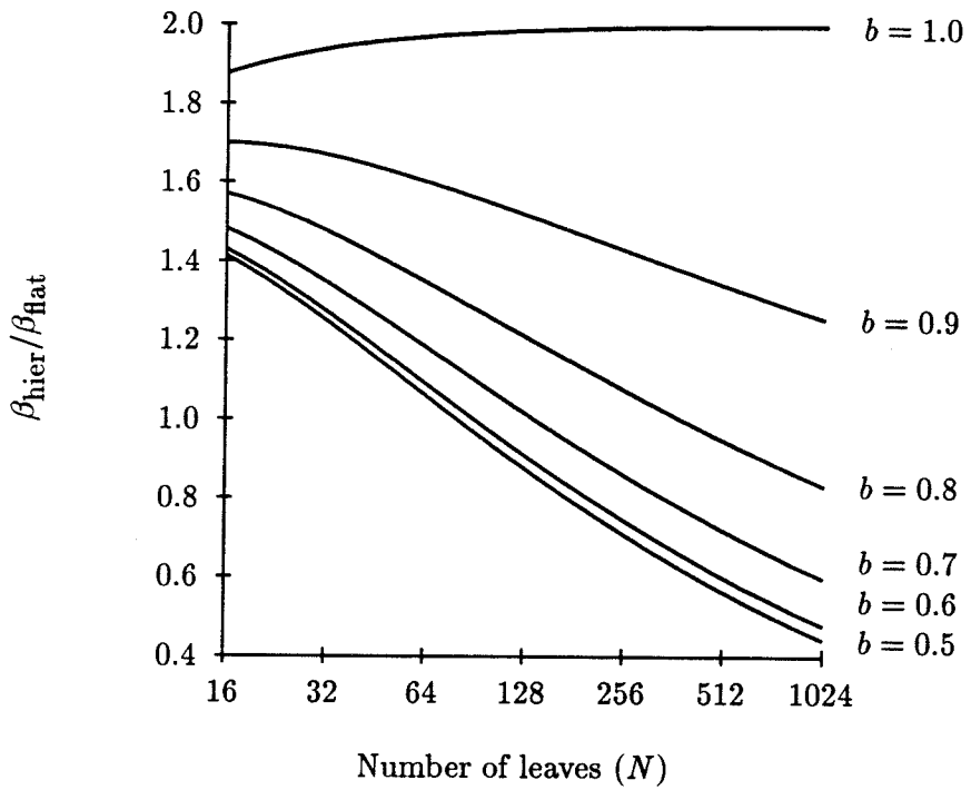
Figure 4.3: Number of switches in hierarchical interconnect relative to flat Rent's rule interconnect. Equation 4.2 is plotted for k = 2 .
