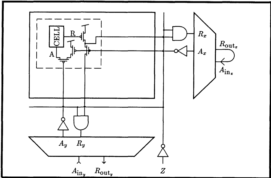
Figure 6.25: Self-timed retina design frame.
