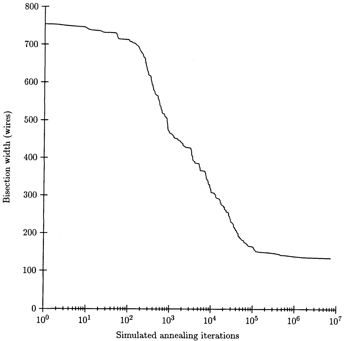
Figure 5.23: Minimum graph-bisection width found by simulated annealing, as a function of annealing algorithm iterations. The graph contained 1000 elements of degree 3, with random connectivity.
