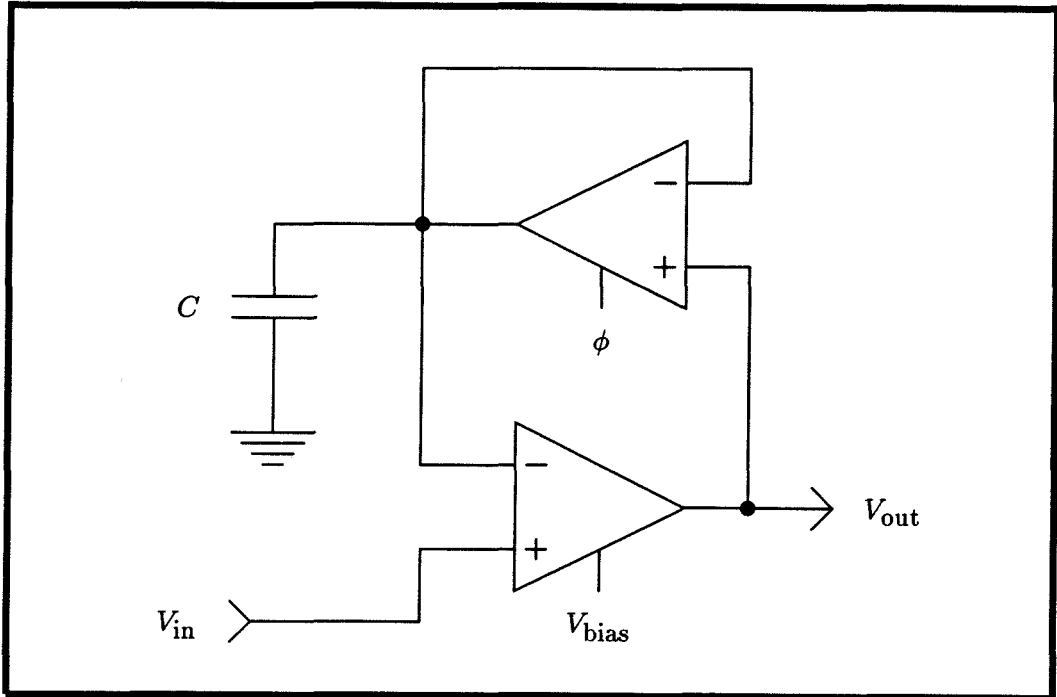
Figure 6.8: The discrete-time differentiator.
