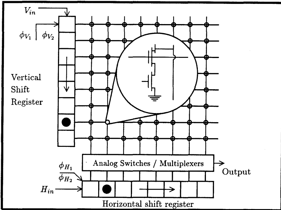
Figure 6.23: First-generation retina design frame.
