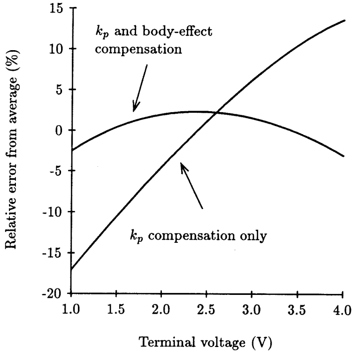
Figure 4.5: Transmission gate small-signal resistance variation. Zero-order compensation is obtained by scaling both devices inversely with their majority carrier mobilities (and hence k_p ). A slightly different scaling can be used to minimize the variation caused by the first-order threshold voltage changes due to the body effect.
