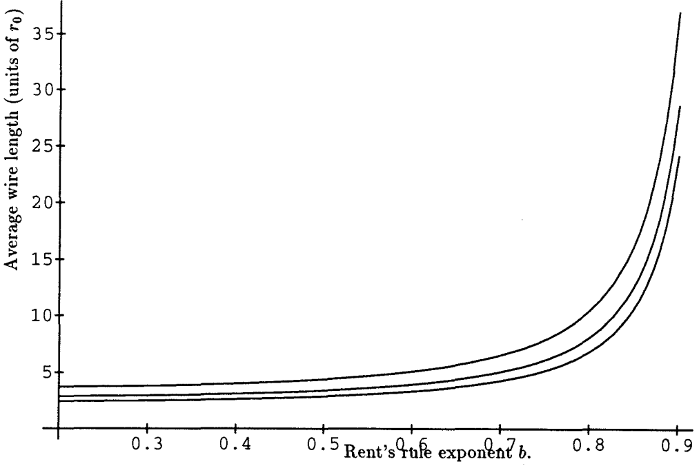
Figure 3.8: Average wire length predicted by model. The wire length is in units of r_0 , and is plotted as a function of the Rent's rule coefficient b , for \gamma = 0.3, 0.5 , and 0.7 .
