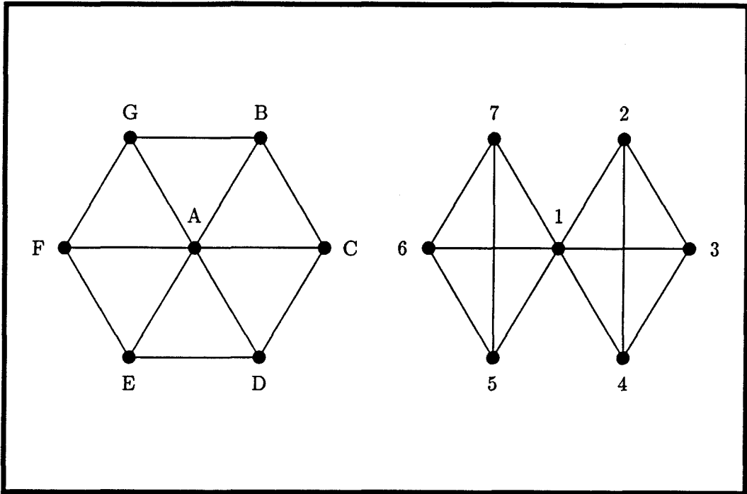
Figure 5.9: Two graphs that are different yet are incompletely partitioned. The algorithm terminates with the equivalence classes \{A, 1\} , \{B, C, D, E, F, G, 2, 3, 4, 5, 6, 7\} . However, exhaustively trial-matching all elements of the second equivalence class yields no self-consistent partition, and hence the graphs are not isomorphic.
