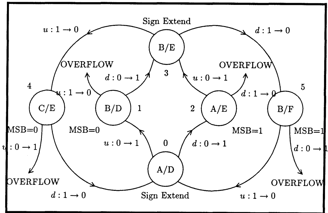
Figure 6.20: State-transition diagram for up-down counter. Transitions in the most significant bits ( u and d ) of the two up-counters are monitored; in conjunction with the current MSB ( x ), they determine the next state.
