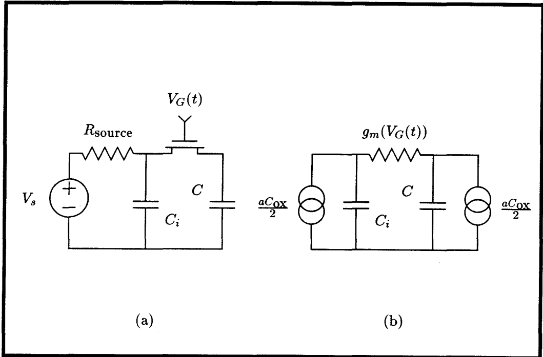
Figure 6.5: A model for MOS channel-charge injection [Vit85].
