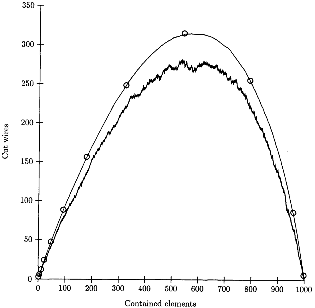
Figure 5.22: Graph bisection width found by greedy algorithm, as a function of number of contained elements. The graph contained 1000 elements of degree 3, with random connectivity. The curves represent the average bisection width (top curve), the best bisection width found (bottom curve—given 100 iterations with random initial element selection), and the predictions of the model (open circles represent data taken from Table 5.2).
