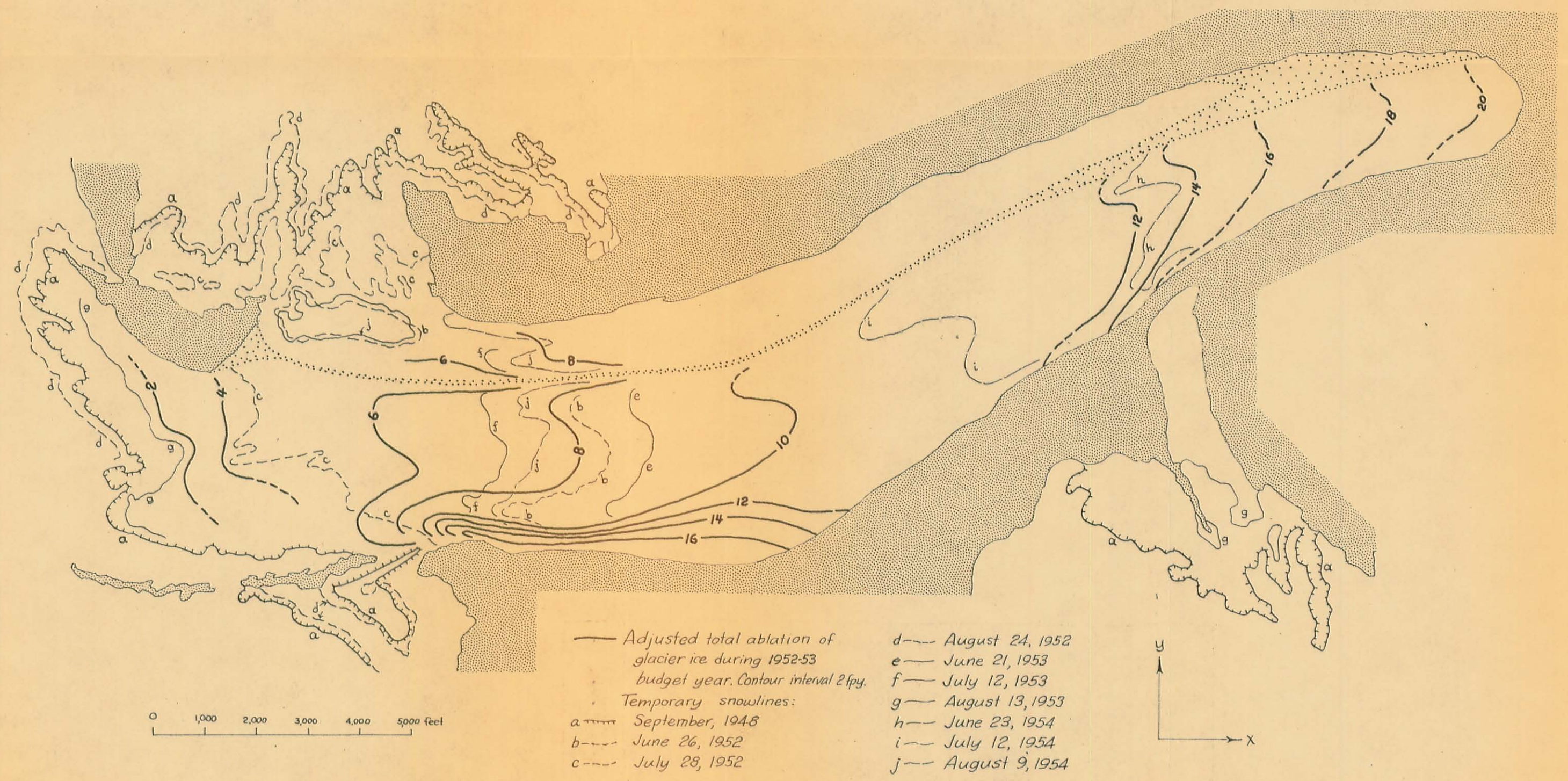
Figure 9. - Total ablation and positions of temporary snowlines
