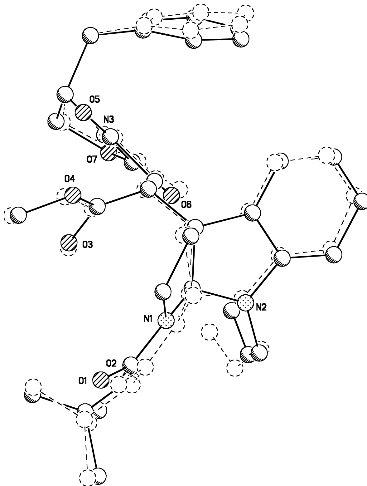
Figure 19. Superposition of molecules A and B of JFA03.
