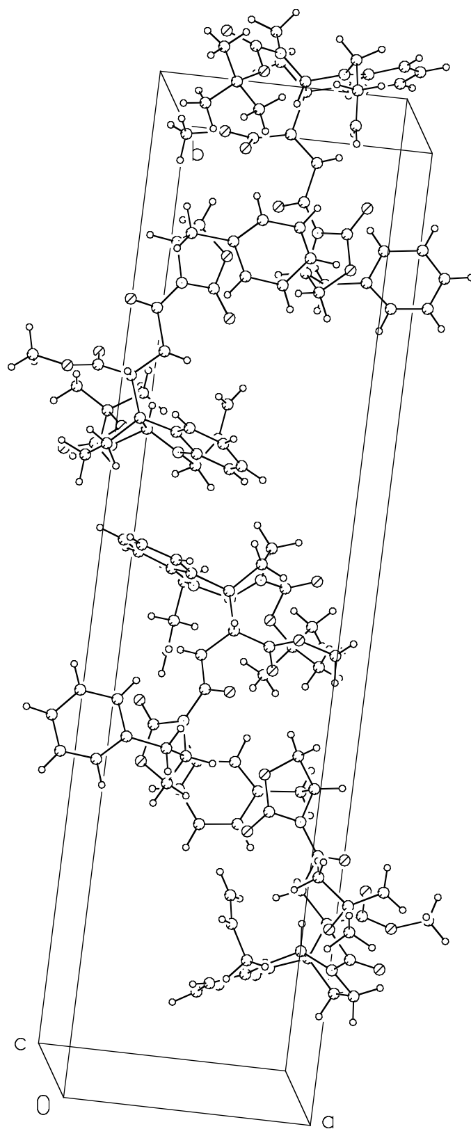
Figure 20. Unit cell contents of JFA03.
