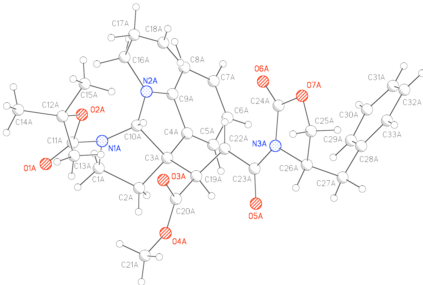
Figure 17. Molecule A of JFA03 with labels.
