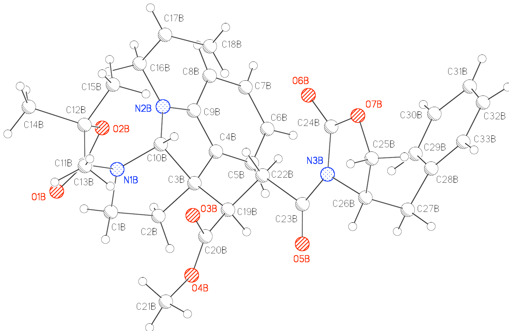
Figure 18. Molecule B of JFA03 with labels.
