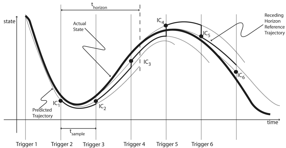
Figure 5.19: Illustration of timing scheme with prediction.
