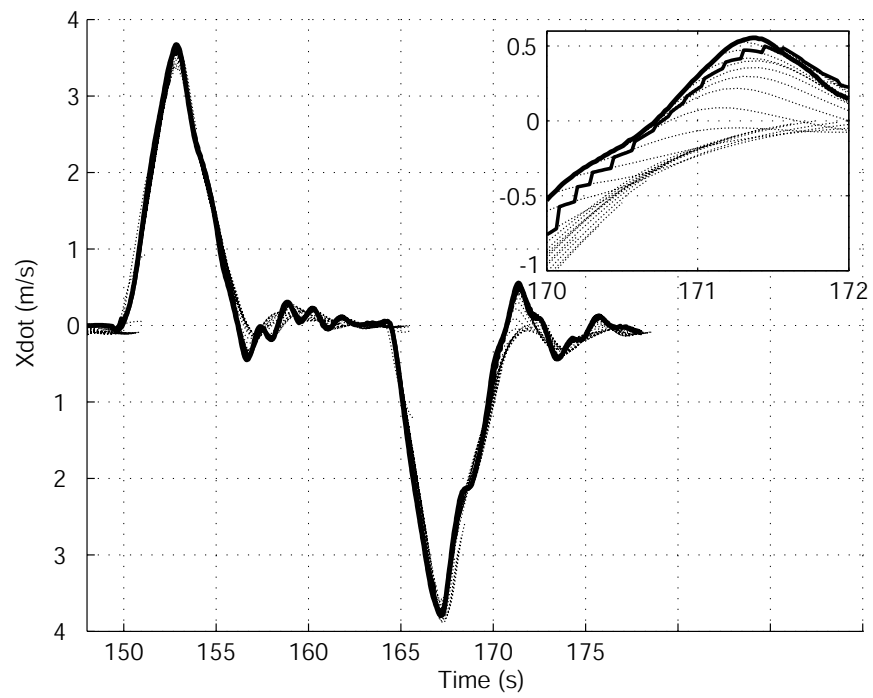
Figure 5.24: The spatial horizontal velocity of the ducted fan
