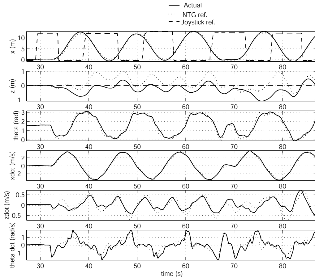
Figure 5.6: “Shuttle” maneuver depicting joystick command , NTG reference trajectory, and actual state
