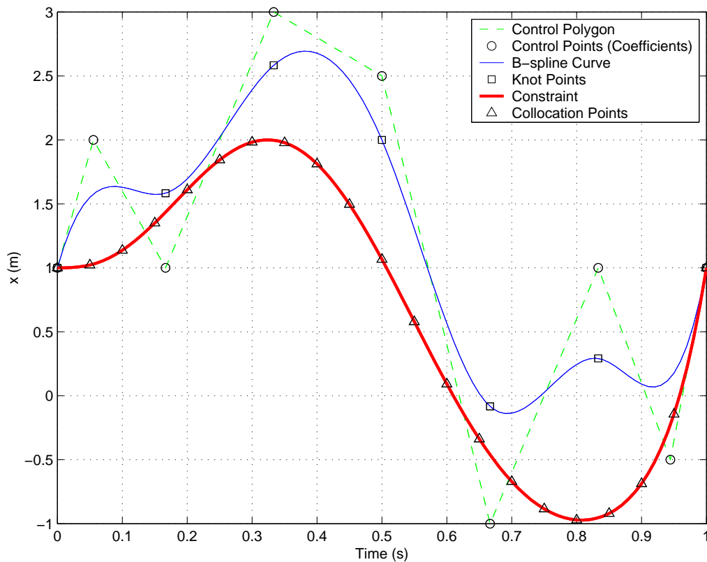
Figure 3.1: In this hypothetical problem, the B-spline curve has six intervals ( l = 6 ), fourth order ( k = 4 ), and is C^3 at the breakpoints (or smoothness s = 3 ). The constraint on the B-spline curve (to be larger than the constraint in this example) will be enforced at the 21 collocation points. The nine control points are the decision variables.
