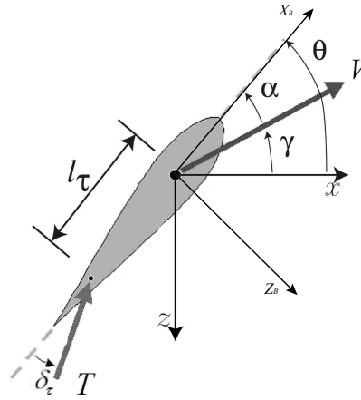
Figure 5.2: Ducted fan coordinate frames
