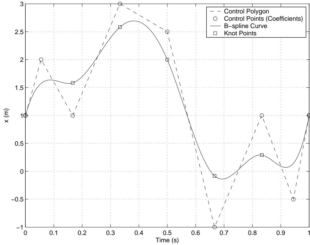
Figure 2.6: The B-spline curve has six intervals ( l = 6 ), fourth order ( k = 4 ), and is C^3 at the breakpoints (or smoothness s = 3 ). The nine control points are the decision variables.
