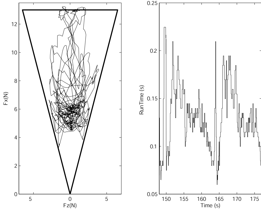
Figure 5.25: Force constraints and computation times.
