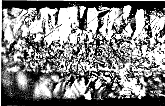
Alloy 2(0.23 At% Cr)
