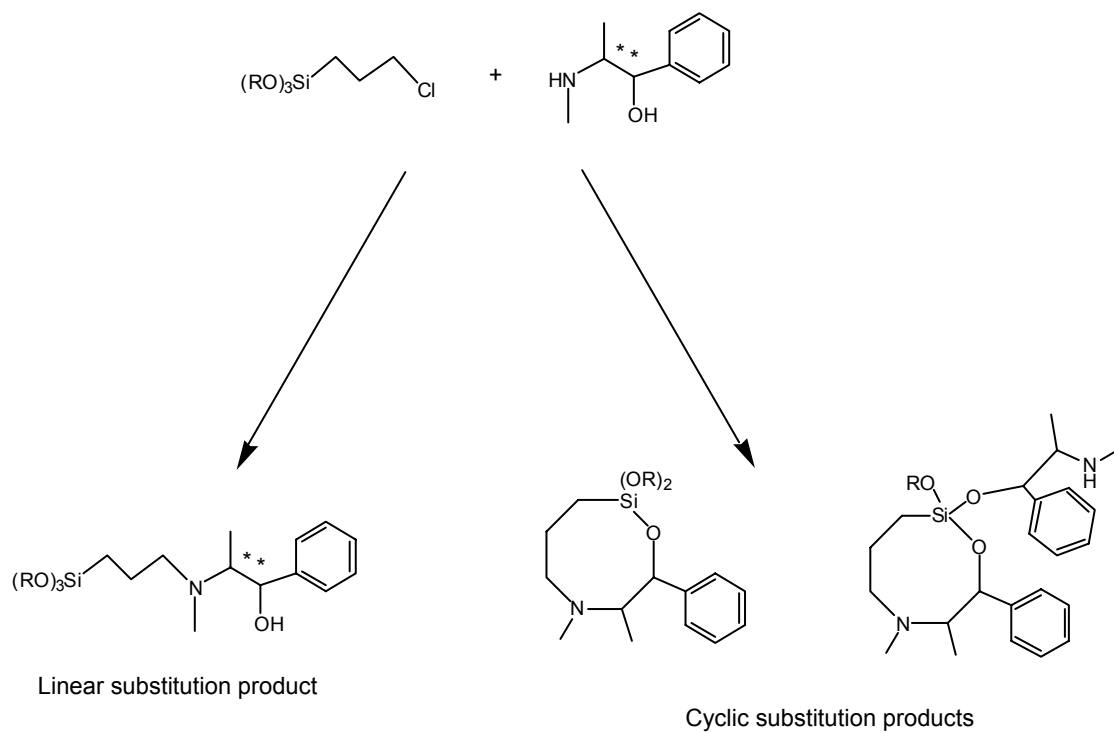
Scheme 3.24 Products of nucleophilic substitution of chloropropylsilane and (-)-ephedrine. Adapted from ref. 40.
