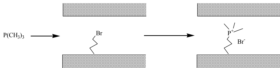
Scheme 4.6 Shape-selective nucleophilic displacement within extracted Br-*BEA.
