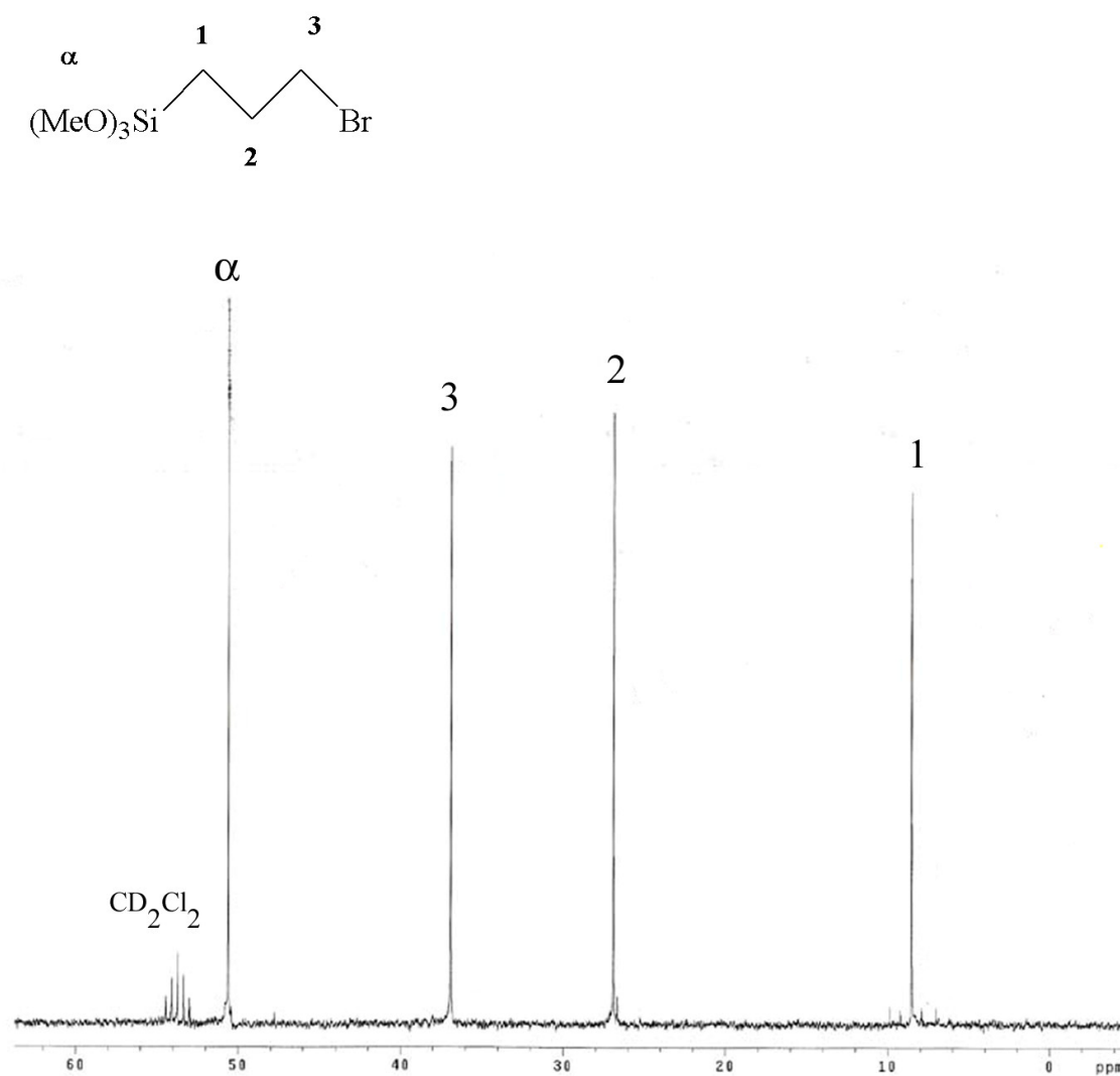
Figure 4.2 ^{13}\text{C} liquid NMR of 3-bromopropyltrimethoxysilane obtained from United Chemicals Technologies, Inc., in \text{CD}_2\text{Cl}_2 .
