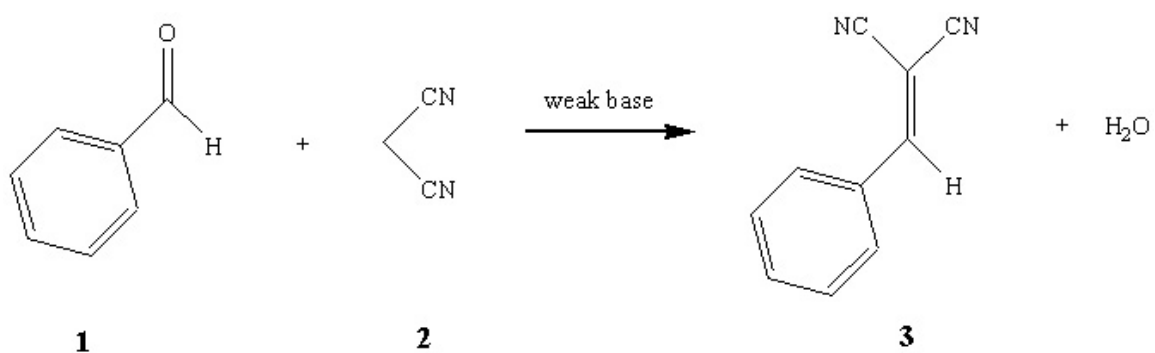
Scheme 5.1 Knoevenagel condensation of benzaldehyde ( 1 ) and malononitrile ( 2 ).
