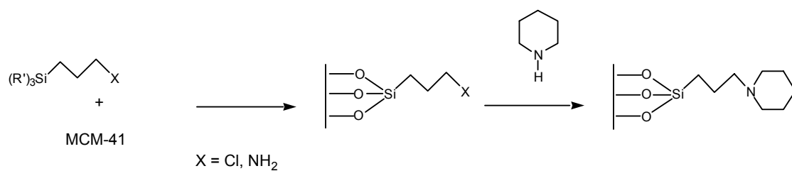
Scheme 3.14 Preparation of amine-containing MCM-41 hybrids for monoglyceride synthesis. Adapted from ref. 27.
