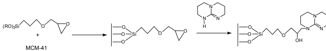
Scheme 3.15 Synthesis of guanidine hybrid materials. Adapted from ref. 29.
