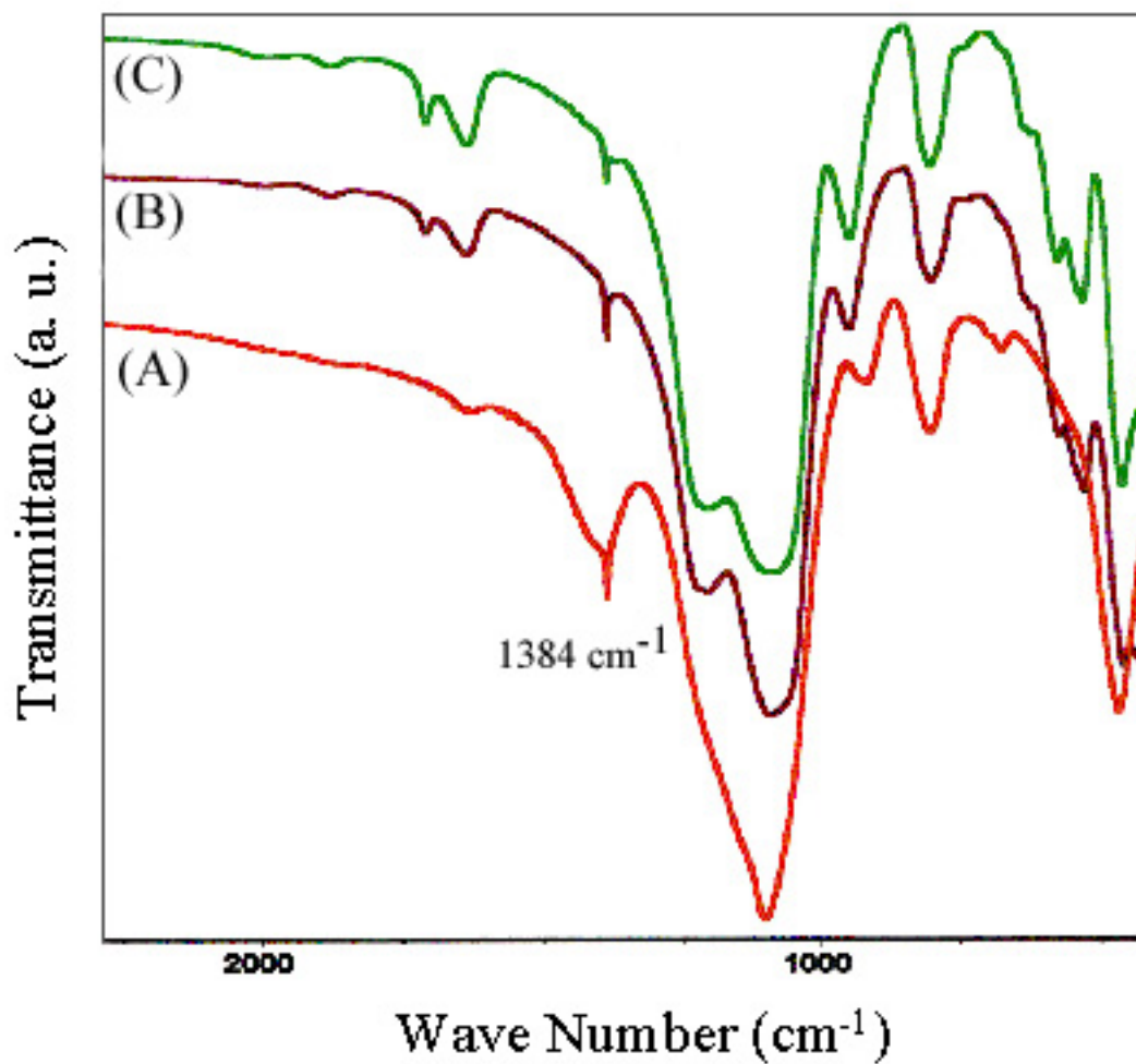
Figure 4.26 FTIR Spectra of (A) \text{P}^+\text{NO}_3^- -CPG, (B) \text{P}^+\text{NO}_3^- -*BEA (from Cl), and (C) \text{P}^+\text{NO}_3^- -*BEA (from Br).
