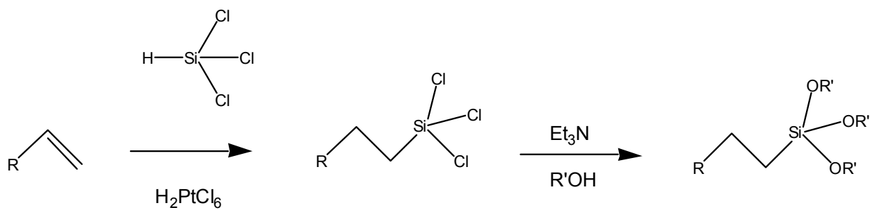
Scheme 3.3 A synthetic route to organosilanes. Adapted from ref. 6.
