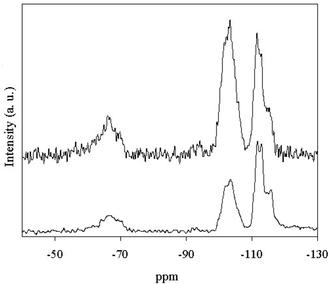
Figure 4.19 ^{29}\text{Si} CP/MAS NMR of (A) \text{P}^+\text{Br}^- \cdot \text{BEA} , and (B) \text{P}^+\text{Ph}_3\text{Br}^- \cdot \text{BEA} .
