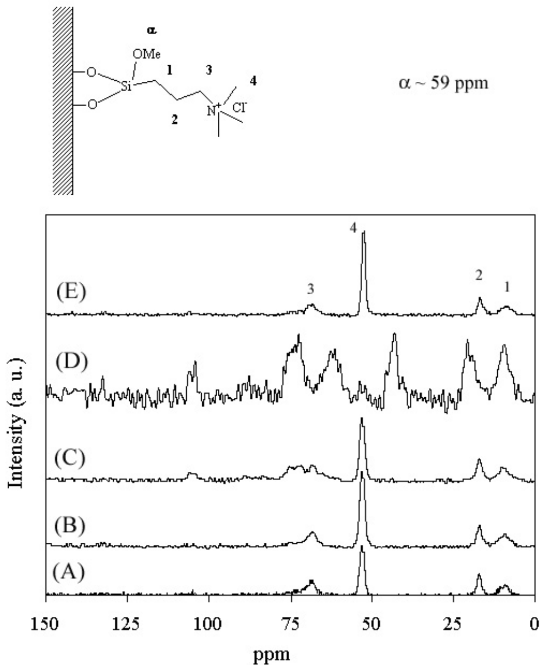
Figure 4.14 ^{13}\text{C} CP/MAS NMR of ammonium-containing CPG: (A) Q-CPG as-made, (B) after heating to 25°C under vacuum, (C) after heating to 100°C under vacuum, (D) after heating to 200°C under vacuum, and (E) after ion-exchange with nitric acid.
