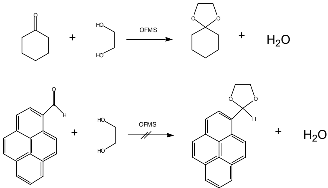
Scheme 3.30 Shape-selective behavior of OFMS catalysts.
