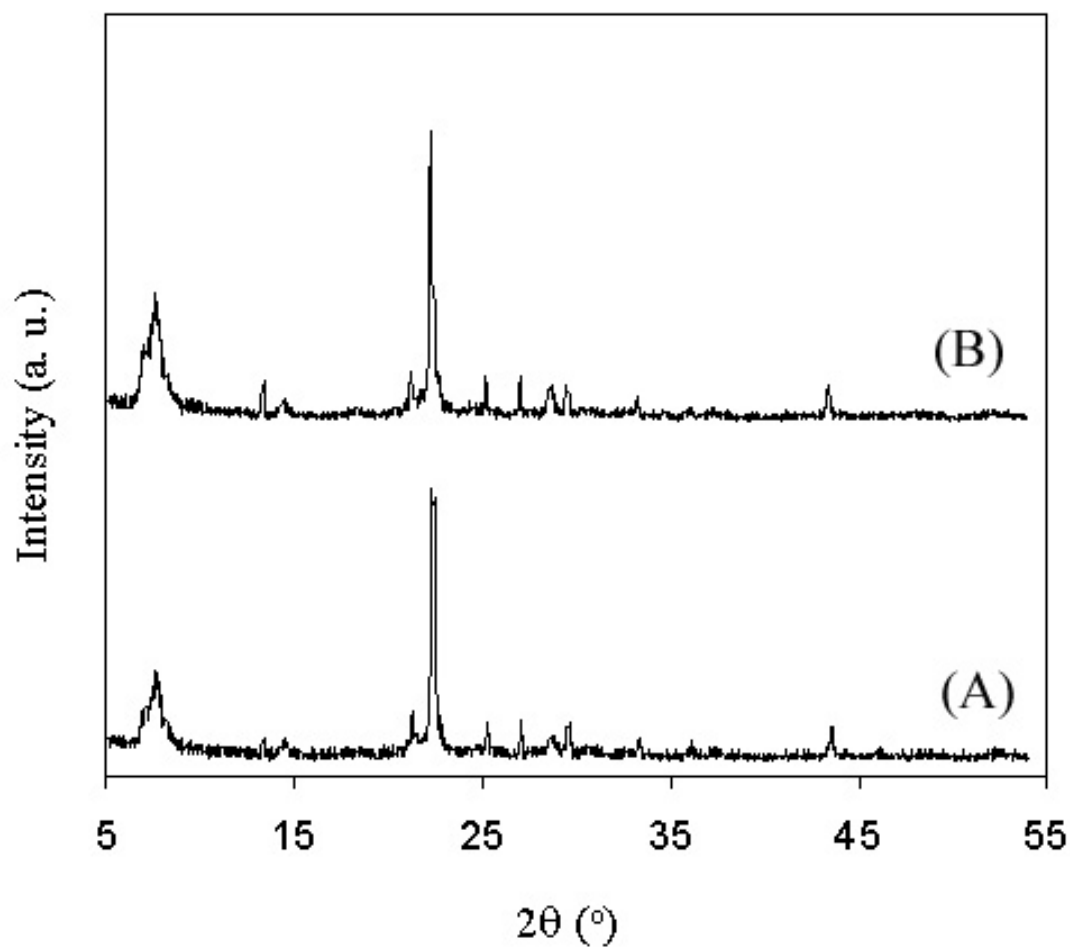
Figure 4.24 XRD of *BEA materials: (A) \text{P}^+\text{NO}_3^- -*BEA and (B) \text{P}^+\text{BPh}_4^- -*BEA.
