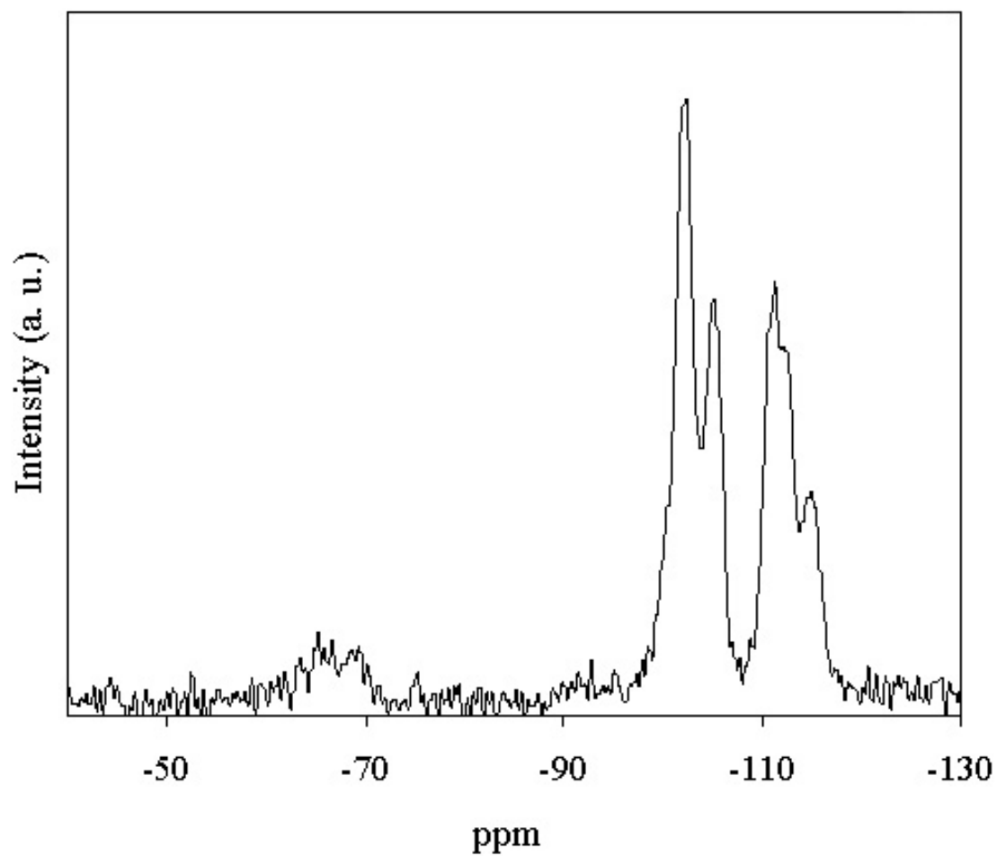
Figure 4.25 ^{29}\text{Si} CP/MAS NMR of ion-exchanged \text{P}^+\text{NO}_3^- -*BEA.
