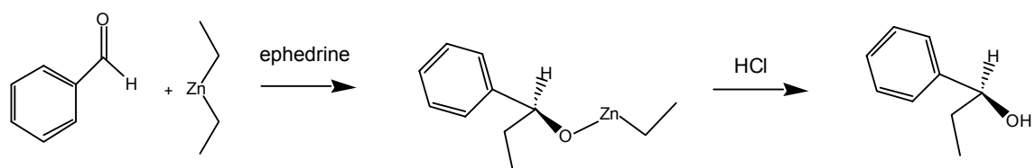
Scheme 3.25 Synthesis of (R)-1-phenyl-propan-1-ol from benzaldehyde and diethylzinc.
