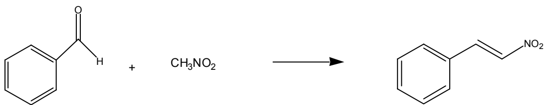
Scheme 3.5 Example of a nitroaldol condensation.
