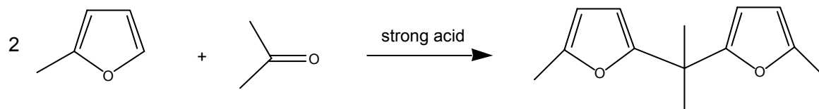
Scheme 3.22 Acid catalyzed addition of 2-methylfuran and acetone.
