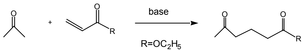
Scheme 2.3 Michael addition. Adapted from ref. 11.
