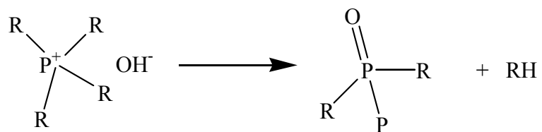
Scheme 4.5 Substitution degradation of quaternary phosphonium compounds.
