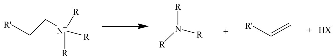
Scheme 4.4 Hofmann degradation of quaternary ammonium compounds.
