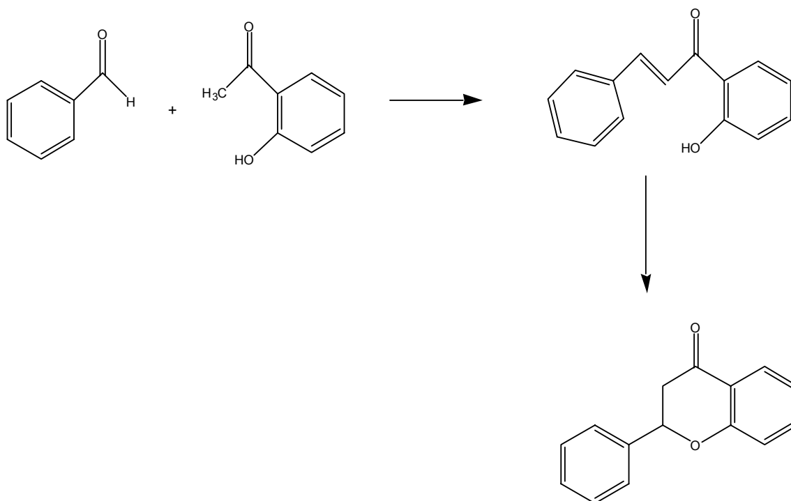
Scheme 3.17 Aldol condensation and intramolecular Michael addition of benzaldehyde and 2'-hydroxyacetophenone to flavanone.
