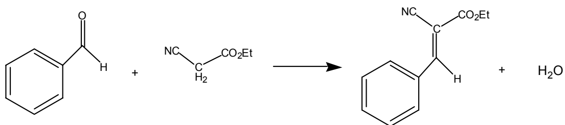
Scheme 3.4 Knoevenagel condensation of benzaldehyde and ethyl cyanoacetate.
