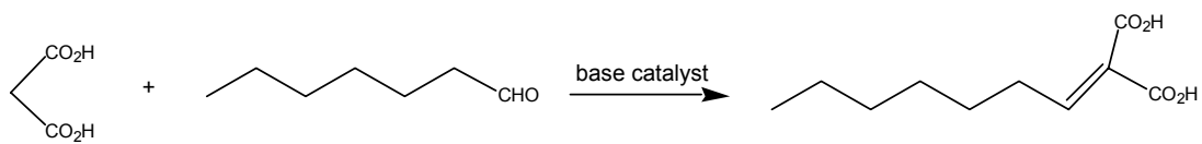
Scheme 3.10 Linstead-Knoevenagel condensation. Adapted from ref. 17.
