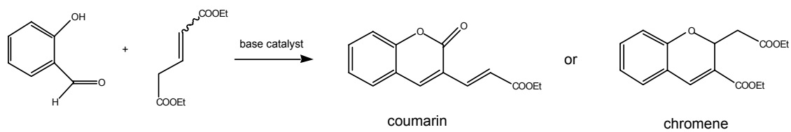
Scheme 3.18 Synthesis of coumarins and chromenes via base catalyzed condensations.
