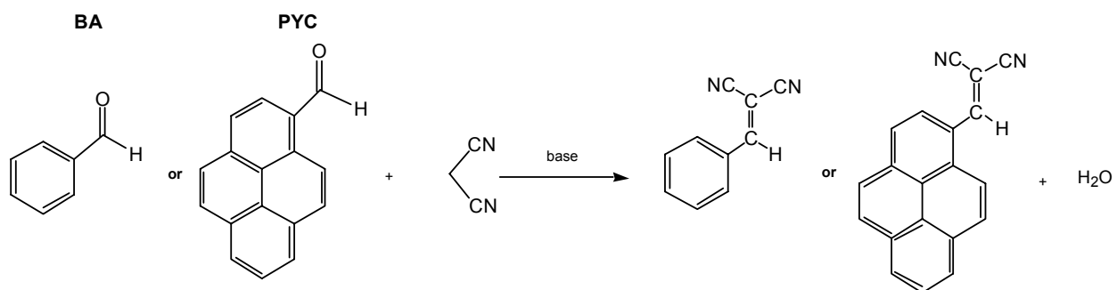
Scheme 2.1 Knoevenagel condensation.
