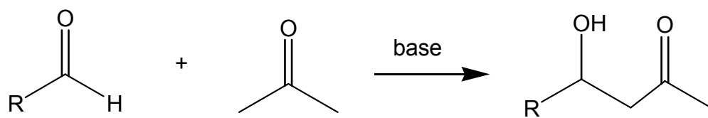
Scheme 2.2 Aldol condensation. Adapted from ref. 23.
