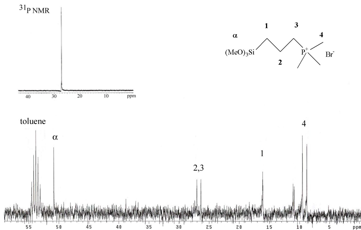
Figure 4.4 ^{13}\text{C} liquid NMR of P-trimethoxysilylpropyl-P,P,P-trimethylammonium bromide, in \text{CD}_2\text{Cl}_2 . Inset is ^{31}\text{P} liquid NMR.
