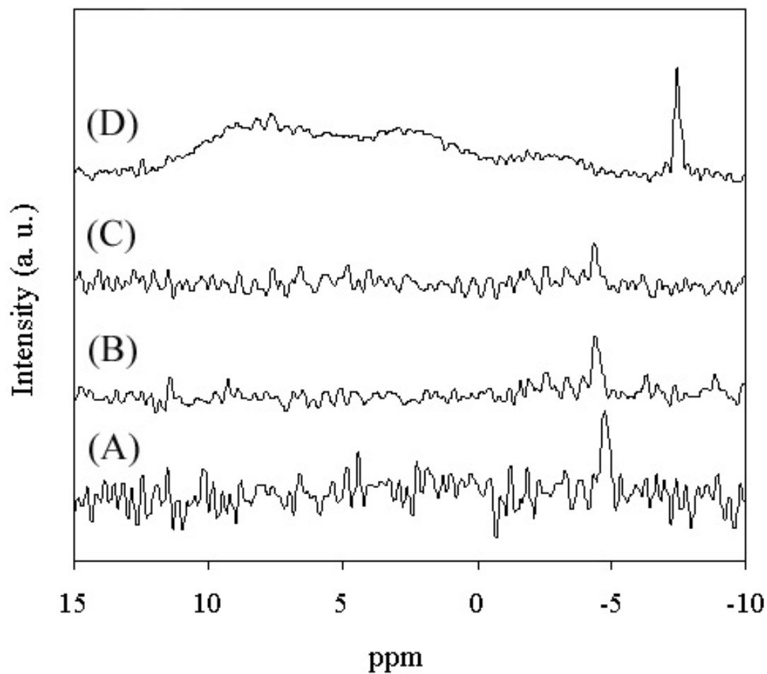
Figure 4.27 ^{11}\text{B} MAS NMR of \text{NaBPh}_4 exchanged materials: (A) Si-*BEA after extraction, (B) \text{P}^+\text{BPh}_4^- -*BEA (from Cl), and (C) \text{P}^+\text{BPh}_4^- -*BEA (from Br), and (D) \text{P}^+\text{BPh}_4^- -CPG (from Cl).
