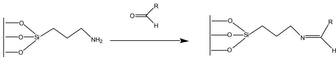
Scheme 3.8 Imine silica preparation from aminopropyl silica. Adapted from ref. 15.
