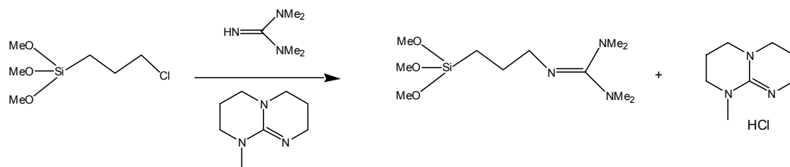
Scheme 3.9 Synthesis of guanidine organosilanes. Adapted from ref. 17.
