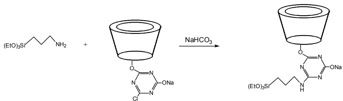
Scheme 3.27 Synthesis of cyclodextrin-containing organosilane. Adapted from ref. 60.
