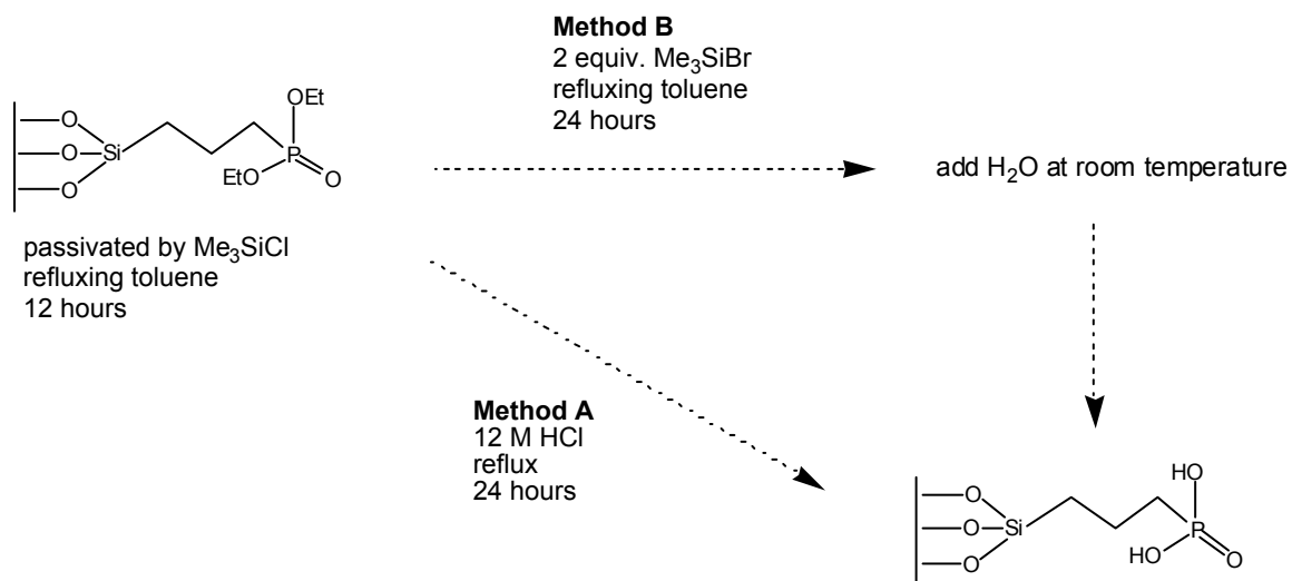
Scheme 3.29 Synthesis of phosphonic acid sites in SBA-15. Adapted from ref. 75.
