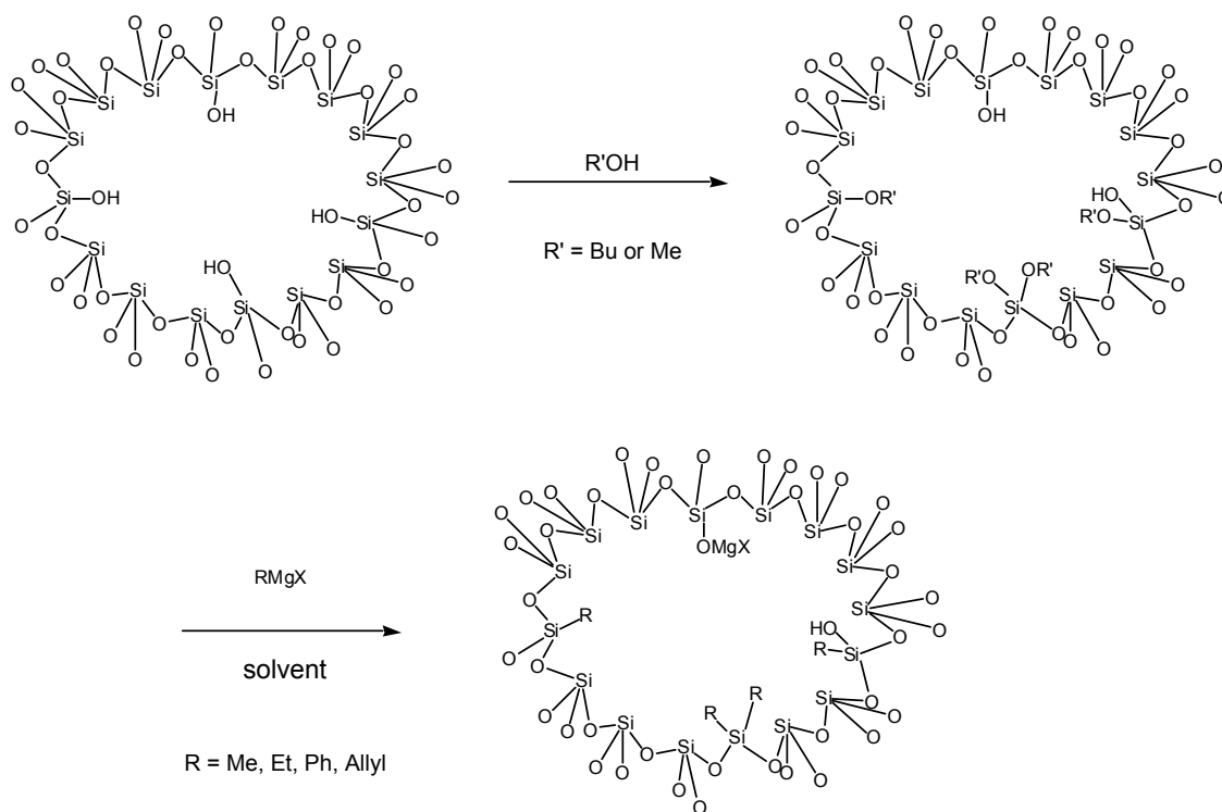
Scheme 3.12 Esterification and Grignard modification of the ordered, mesoporous materials. Adapted from ref. 26.
