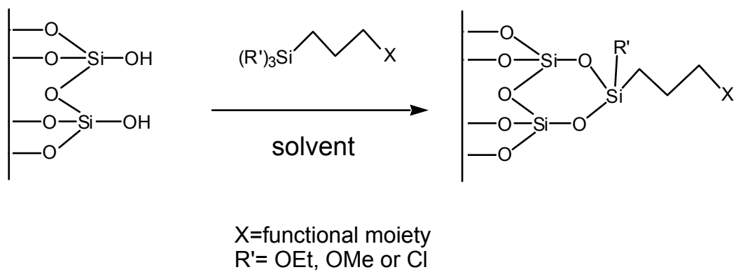
Scheme 3.2 Example of grafting organosilanes onto silanol-containing surface.
