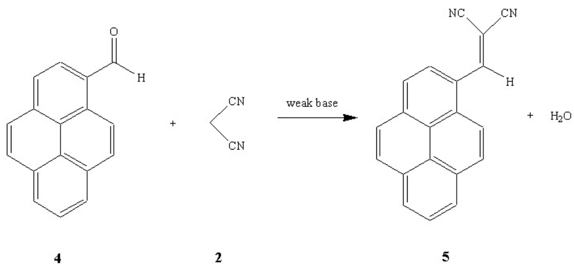
Scheme 5.2 Knoevenagel condensation of 1-pyrenecarboxaldehyde ( 4 ) and malononitrile ( 2 ).
