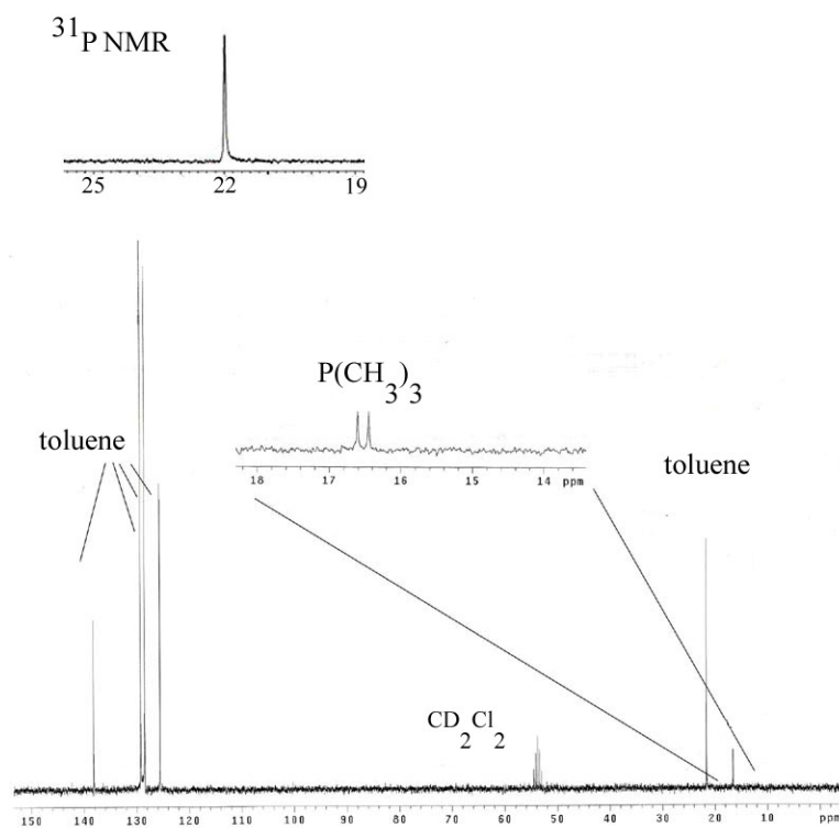
Figure 4.3 ^{13}\text{C} liquid NMR of 1 M trimethylphosphine solution in toluene obtained from Aldrich, in \text{CD}_2\text{Cl}_2 . Inset is ^{31}\text{P} liquid NMR.
