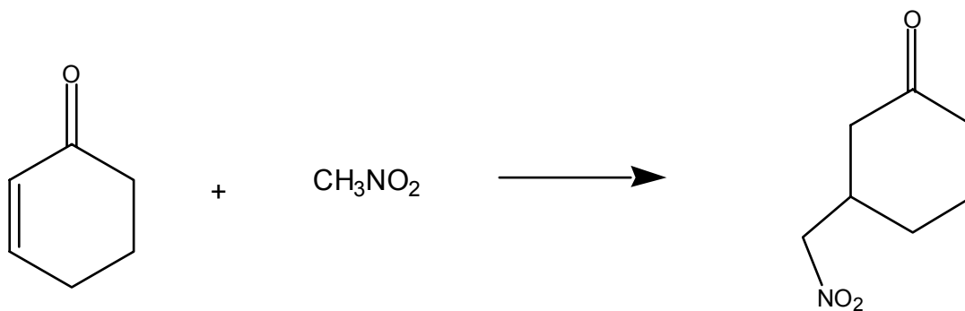
Scheme 3.6 Example of a Michael addition reaction.
