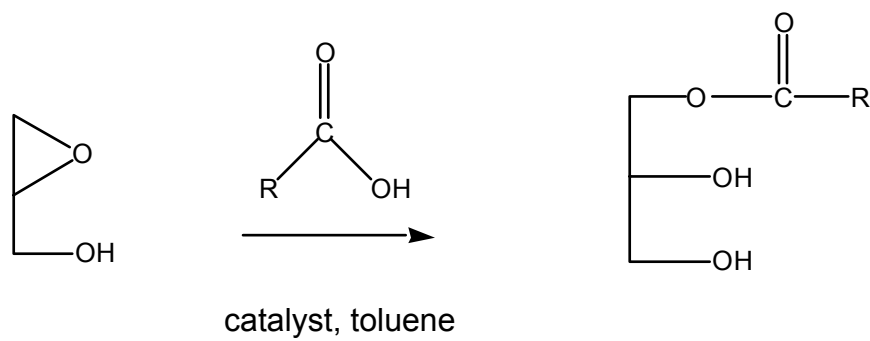
Scheme 3.13 Monoglyceride synthesis from glycidol and fatty acids.
