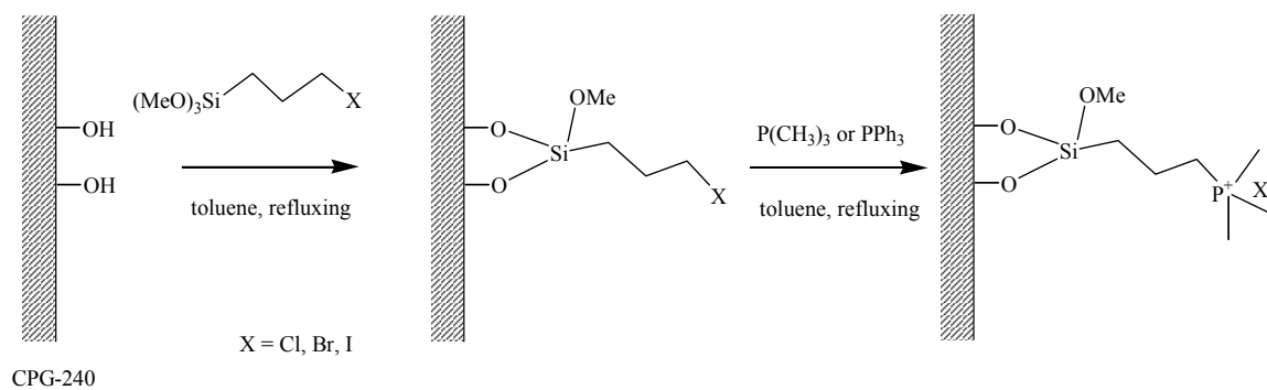
Scheme 4.3 Tethering of organosilanes onto CPG and preparation of phosphonium-functionalized CPG.
