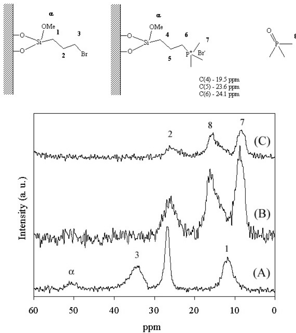
Figure 4.16 ^{13}\text{C} CP/MAS NMR of (A) Br-CPG, (B) \text{P}^+\text{Br}^- -CPG, and (C) \text{P}^+\text{Br}^- -CPG after heat treatment to 300^\circ\text{C} .
