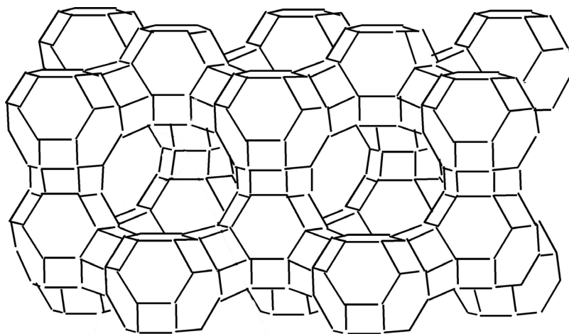
Figure 2.2 Three-dimensional zeolite structure (Faujasite).
