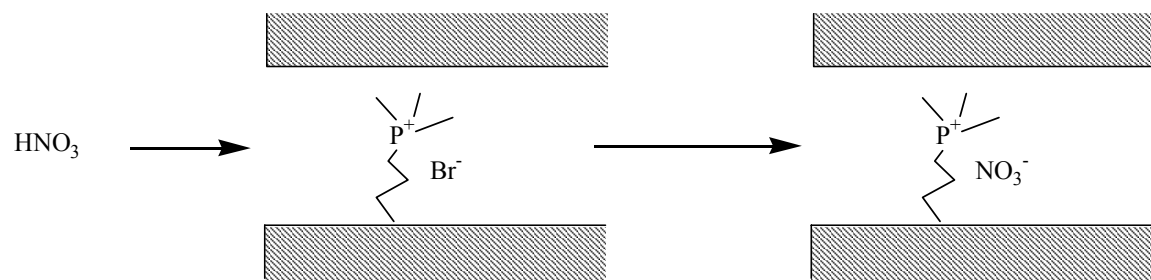
Scheme 4.7 Shape-selective ion-exchange within P^+Br^- -*BEA.
