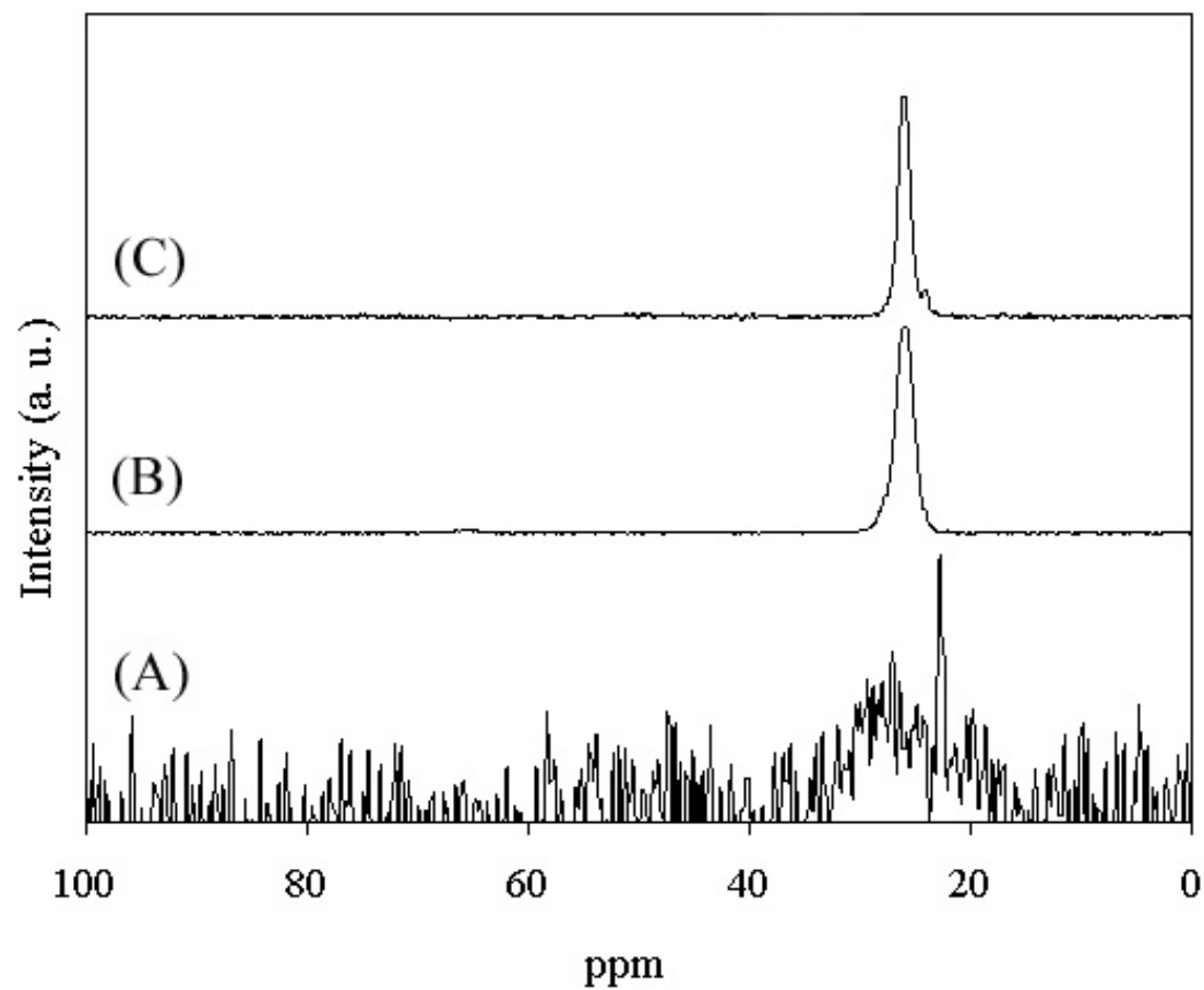
Figure 4.20 ^{31}\text{P} MAS NMR of (A) \text{P}^+\text{Br}^- -*BEA, (B) \text{P}^+\text{Br}^- -CPG, and (C) \text{P}^+\text{Br}^- -CPG heated to 300^\circ\text{C} under vacuum.
