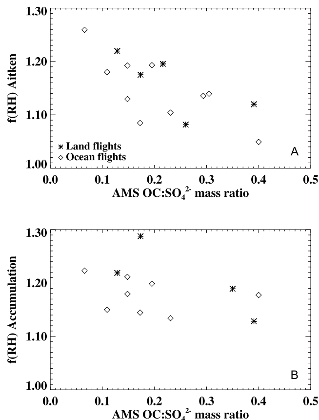
Figure 8. (a) Relationship between Aitken mode f(\text{RH}) and AMS-measured organic carbon to sulfate mass ratio for OC:SO 4 2- ratios below 0.5. (b) Same as Figure 8a, but for accumulation mode f(\text{RH}) .
