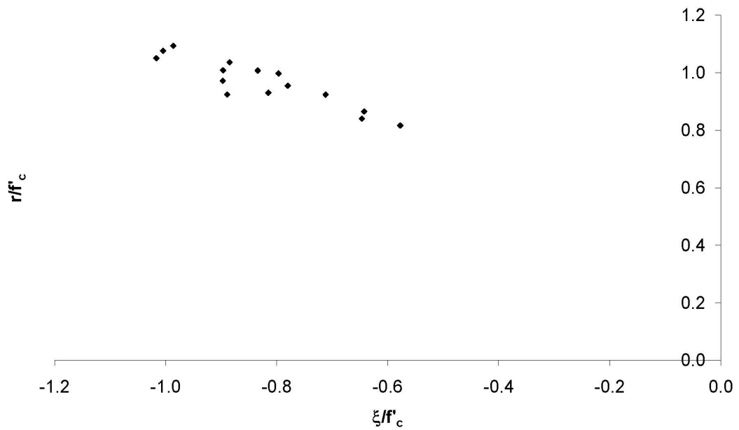
Figure C.11: Test data from Duke and Davis (1944).
