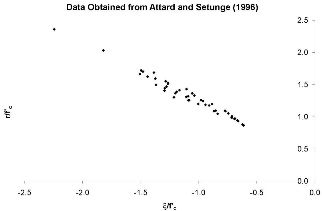
Figure C.3: Test data from Attard and Setunge (1996).
