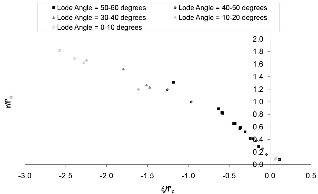
Figure C.19: Test data from Rosenthal and Glucklich (1970).
