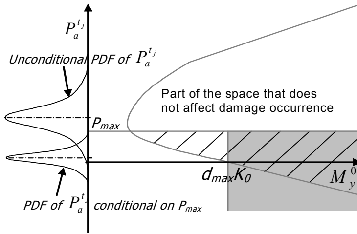
Figure 4.30 Safety regions for exact (hatched) limit-state function and two-dimensional approximate (shaded) limit-state function, axial force is relatively small
