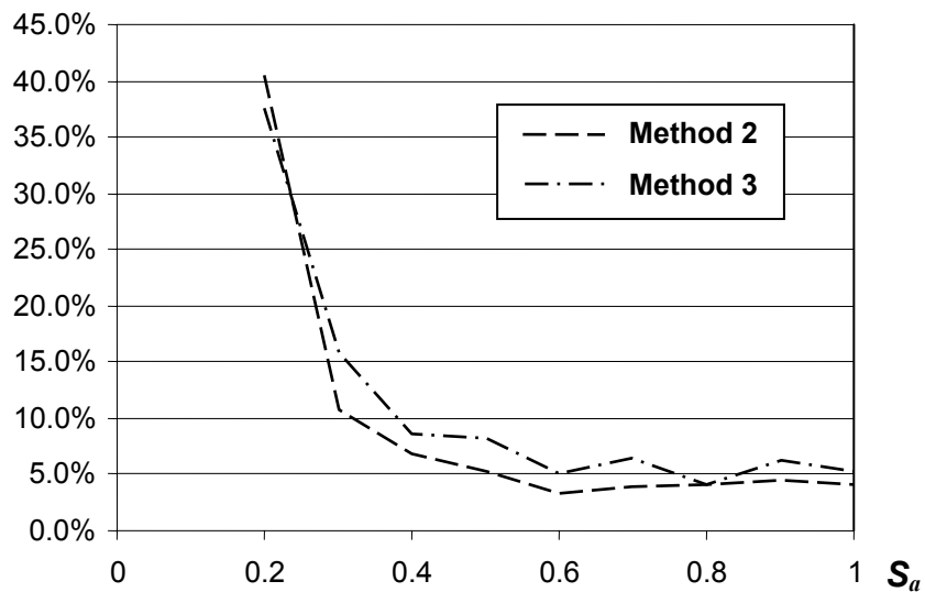
Figure 4.9. Relative errors of estimation of E[N_i] by different methods as a function of spectral acceleration, ground motion LA15.
