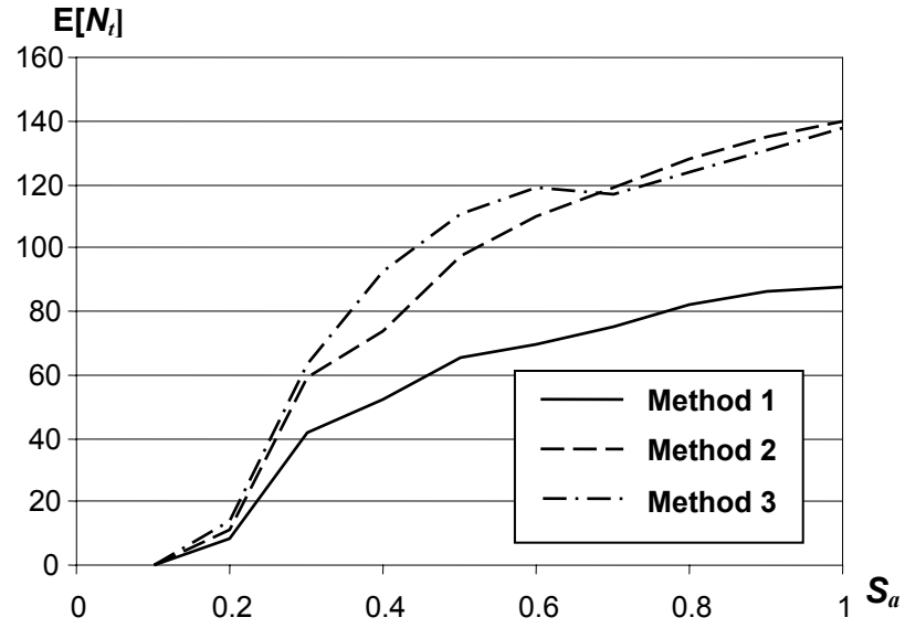
Figure 4.17. Expectation of damage E[N_i] as a function of spectral acceleration for the axial force-flexure interaction model, ground motion LA15.
