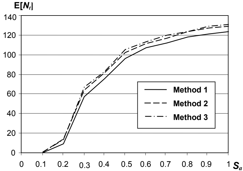
Figure 4.8. Expectation of damage E[N_i] as a function of spectral acceleration, ground motion LA15.
