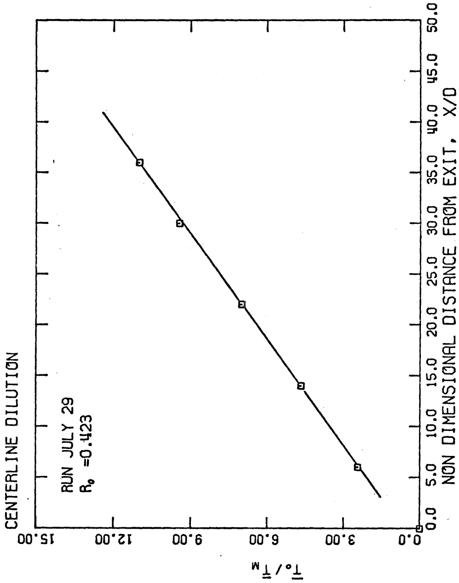
Figure 4.1.8. Temperature distribution along plume axis.
