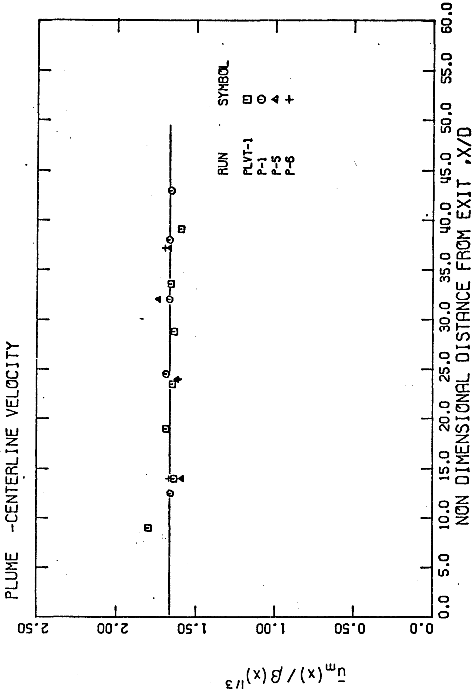
Figure 5.3.1. Velocity distribution along plume axis.
