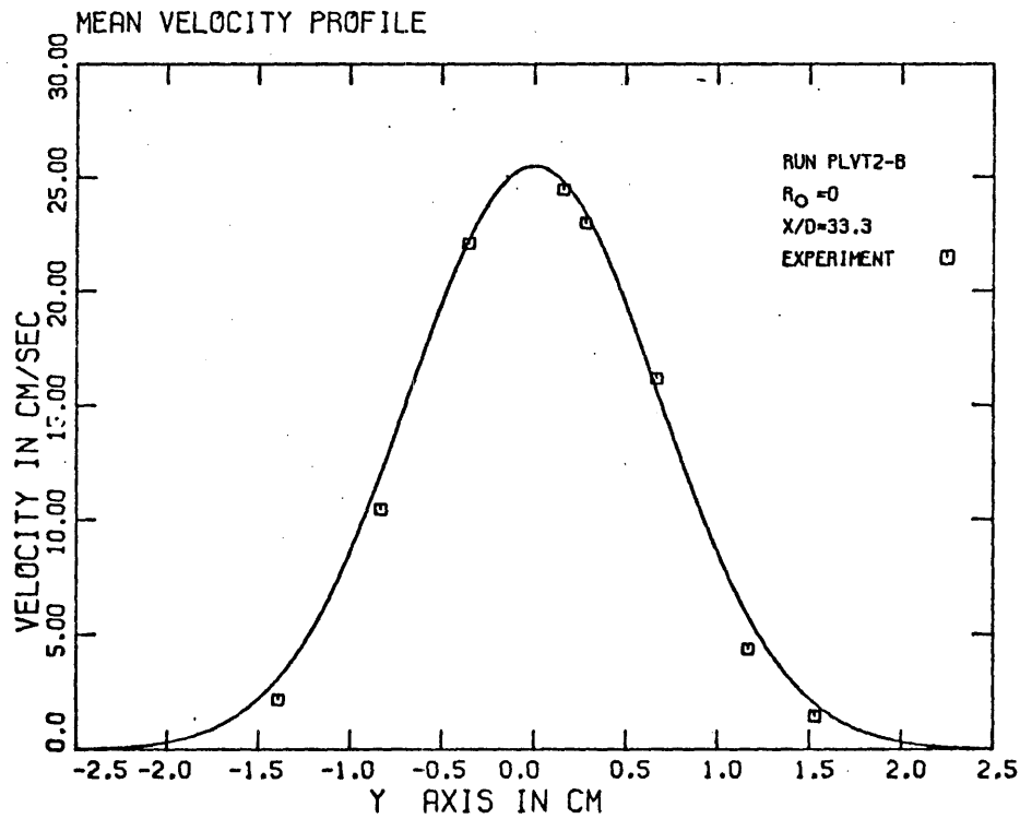
Figure 5.1.b. Mean velocity profile for a turbulent jet at X/D = 33.3
