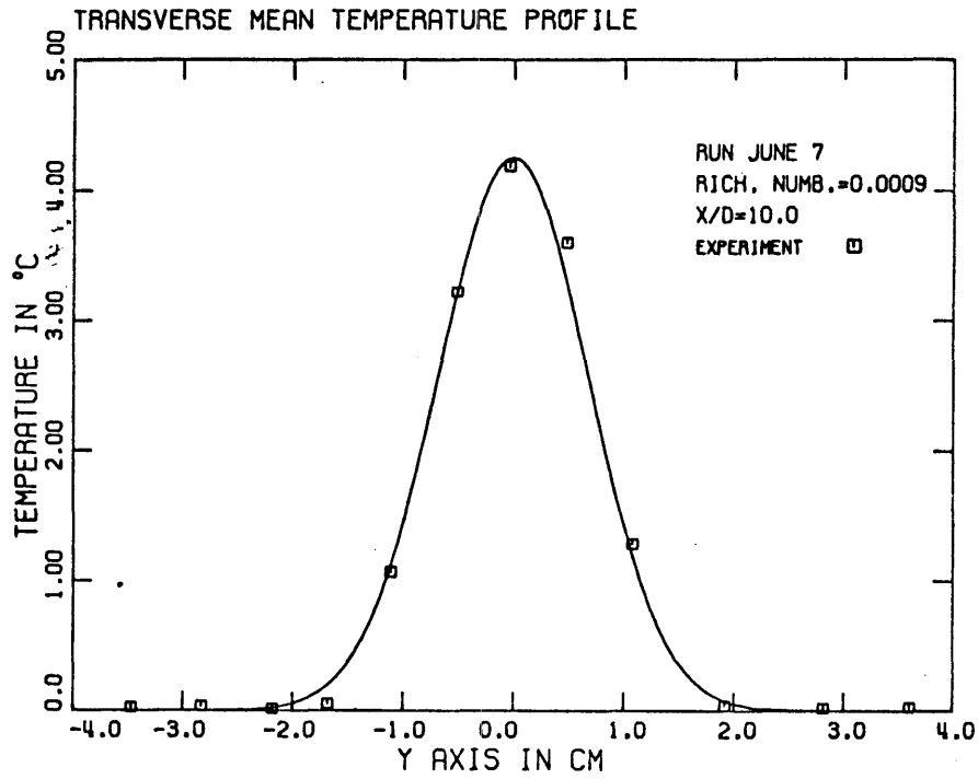
Figure 4.1.1.a. Mean temperature profile for a turbulent jet at x/D = 10.0 .
