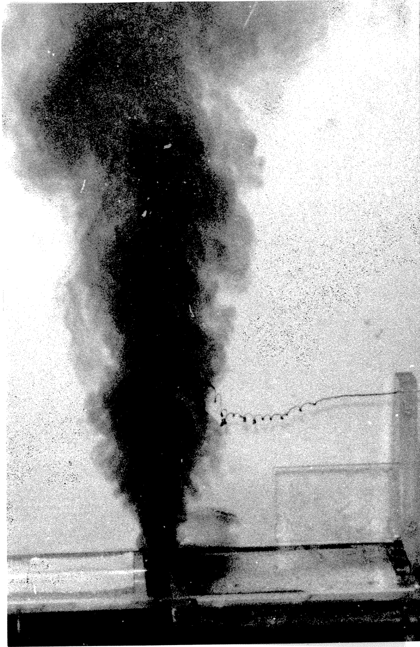
Figure A.3. Medium time (2 seconds) exposure photograph of a turbulent two-dimensional plume ( R_0 \approx 0.5 ).
