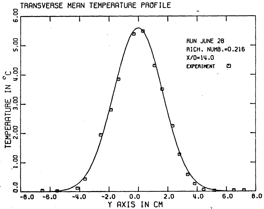
Figure 4.1.4.b. Mean temperature profile for a turbulent plume at x/D = 14.0 .
