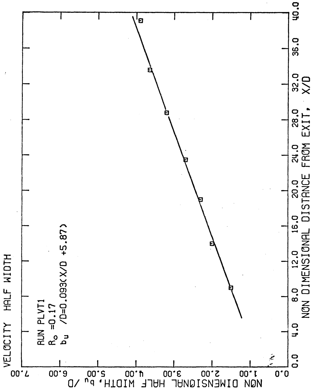
Figure 5.1.5. Non-dimensional velocity half-width of a turbulent plume plotted against non-dimensional distance from jet orifice.
