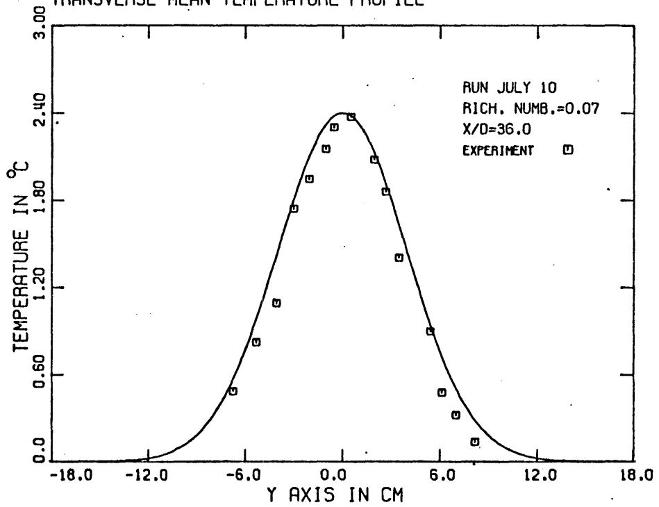
TRANSVERSE MEAN TEMPERATURE PROFILE
