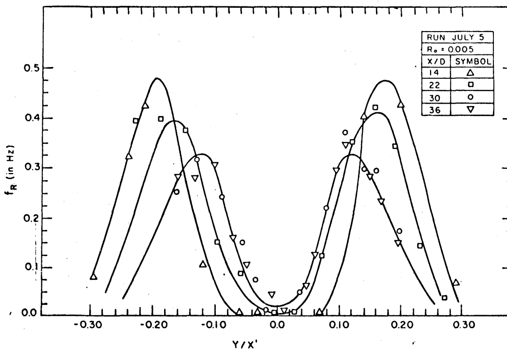
Figure 4.5.3. Profile of frequency of hot/cold, cold/hot interface crossing for a turbulent jet.
