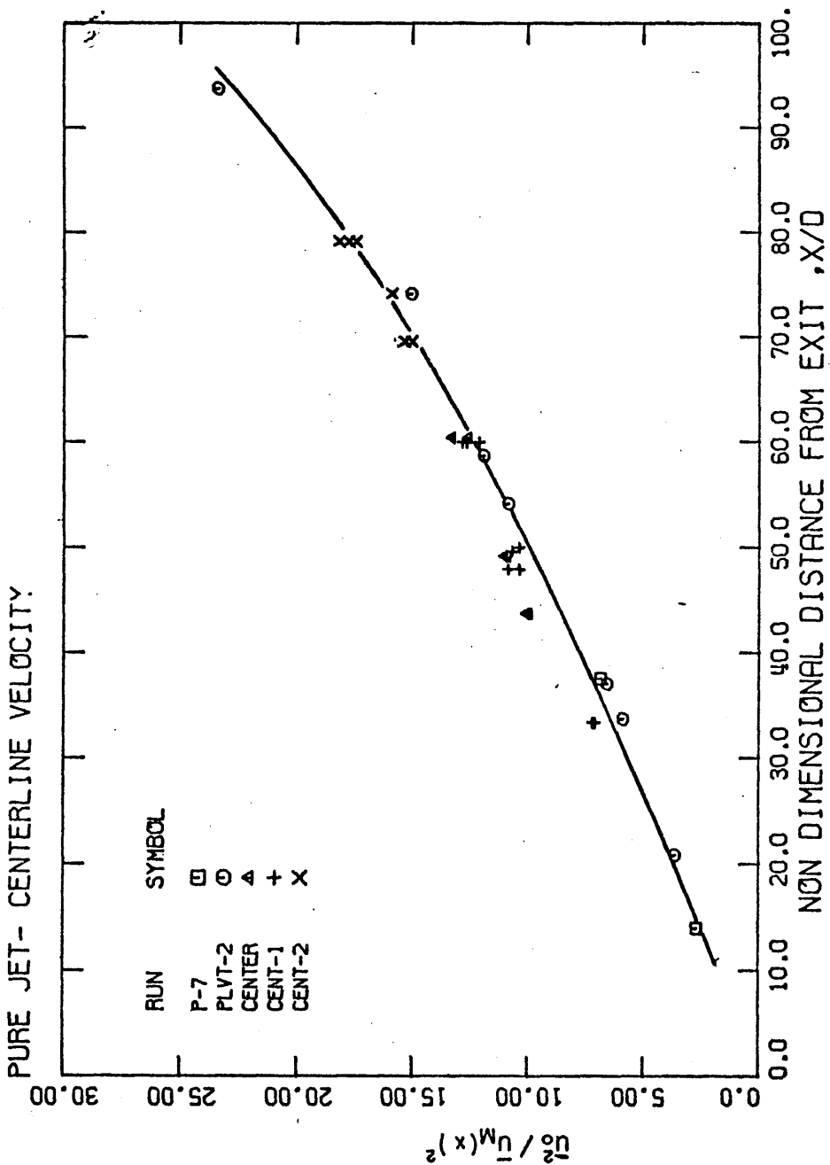
Figure 8.10. Velocity ratio \bar{u}_0^2/\bar{u}_M^2(x) as a nonlinear function of non-dimensional distance x/D .
