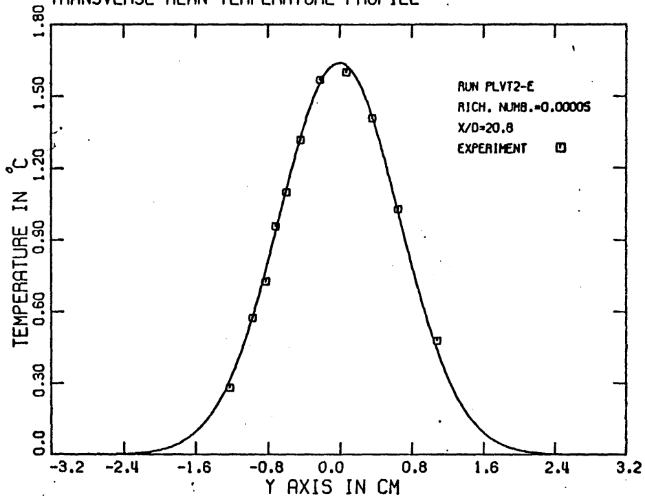
TRANSVERSE MEAN TEMPERATURE PROFILE
