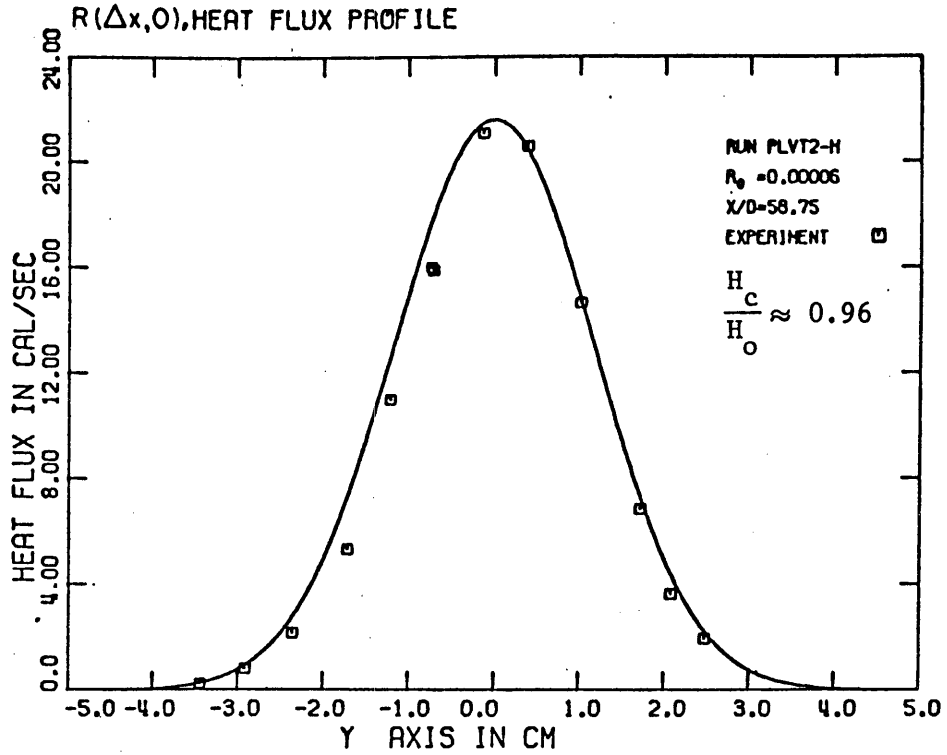
Figure 6.2.2.c. Profile of the correlation \rho c_p R(\Delta x, 0) in a turbulent jet at x/D = 58.75 .
