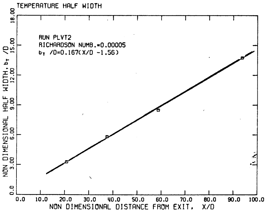
Figure 6.1.2.b. Temperature half-width of a jet ( R_0 \approx 0 ) as a function of distance along the jet.
