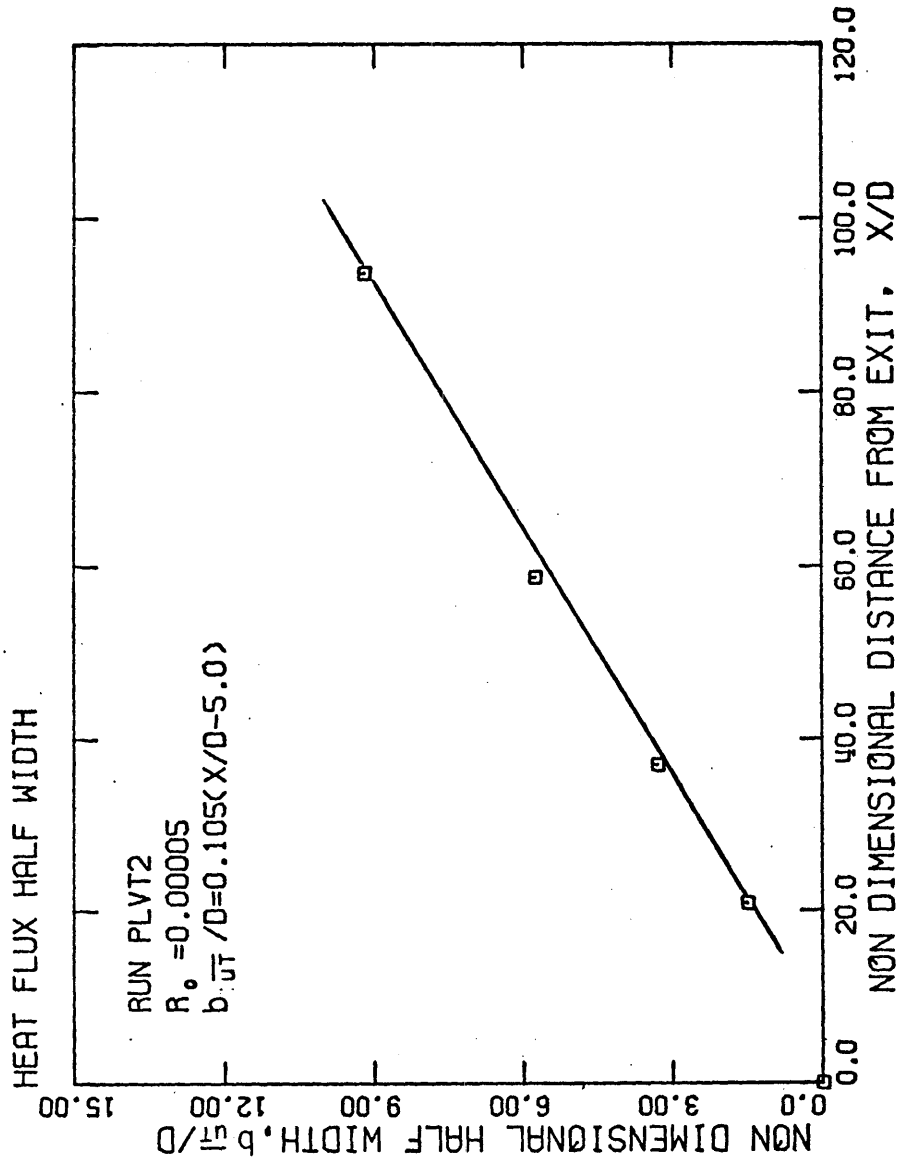
Figure 6.2.4. Heat flux half-width for a turbulent jet as a function of distance along the jet axis.
