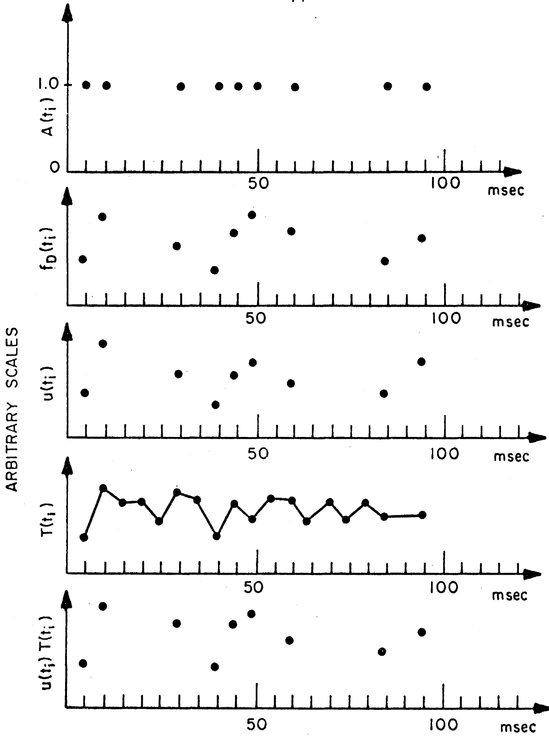
Figure 3.3.2. Schematic for the measurement of the correlation \overline{uT} .
