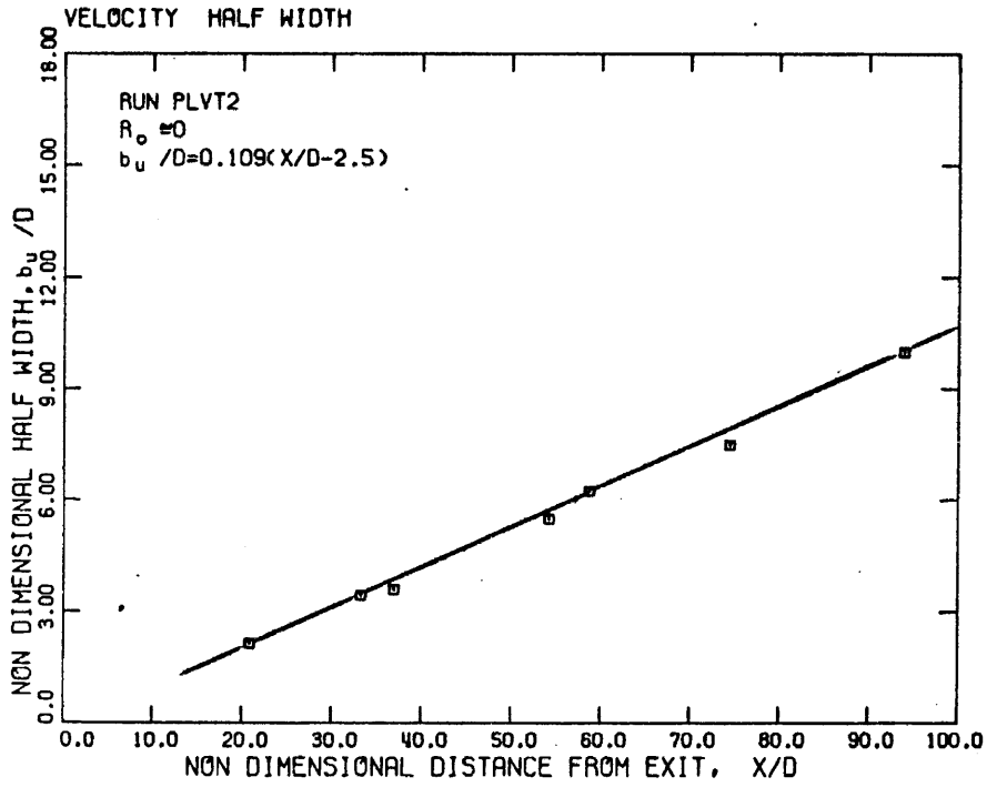
Figure 6.1.2.a. Velocity half-width of a jet ( R_0 \approx 0 ) as a function of distance along the jet.
