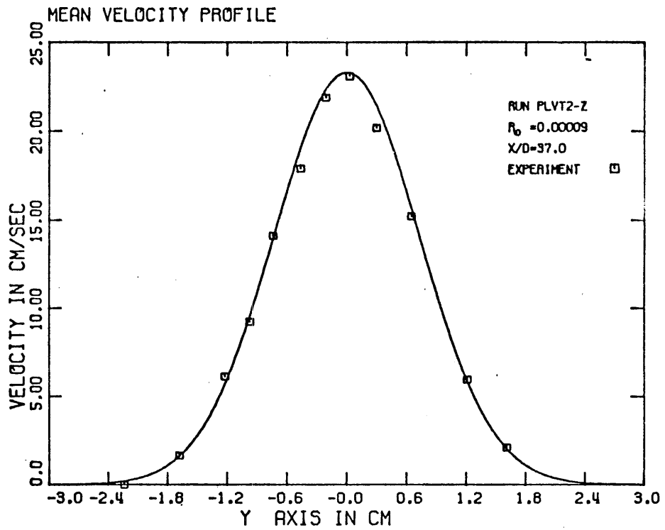
Figure 5.1.1.c. Mean velocity profile for a turbulent jet at X/D = 37.0
