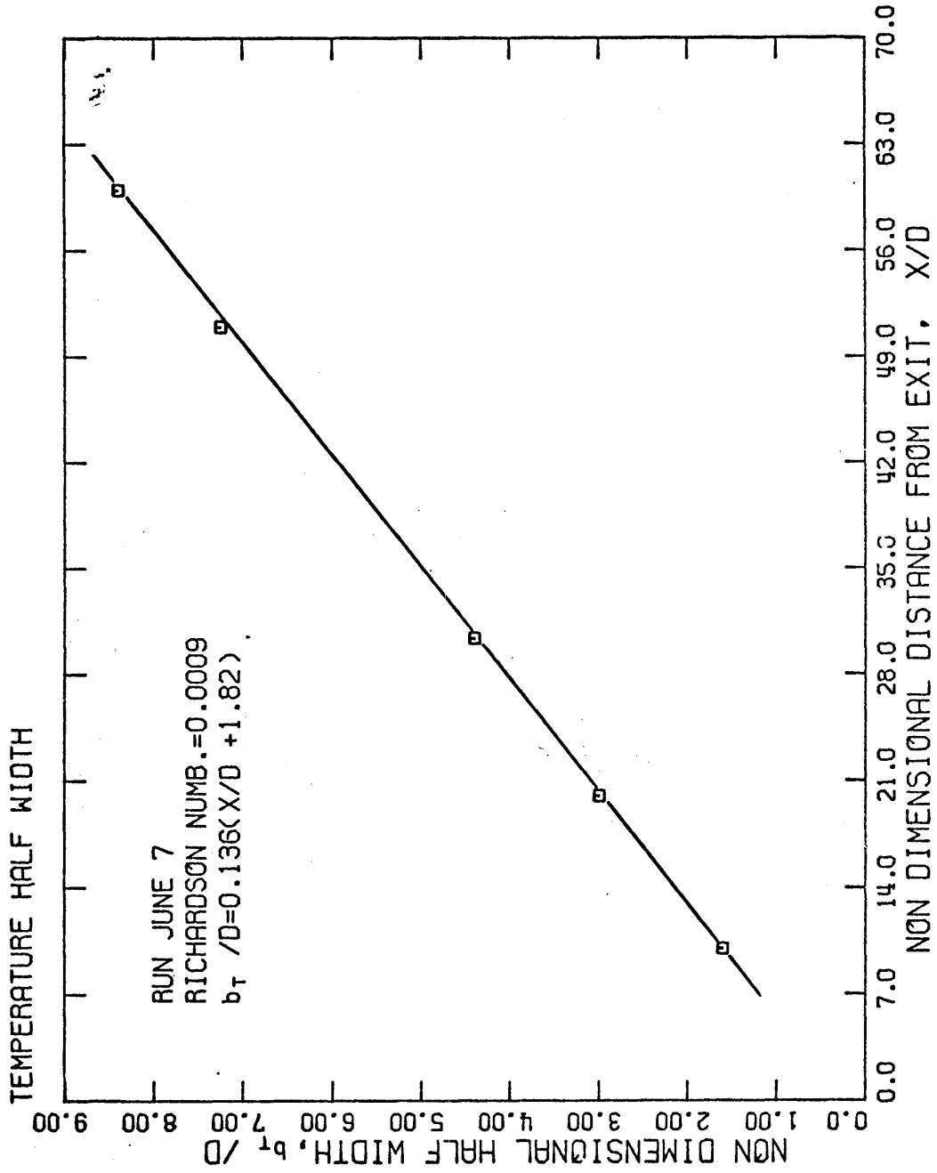
Figure 4.1.2. Non-dimensional temperature half-width of a turbulent jet plotted against non-dimensional distance along the jet axis.
