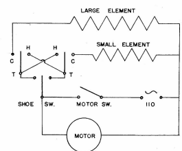
COMPLETE WIRING DIAGRAM
