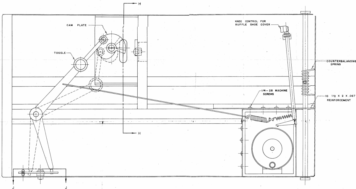
BOTTOM VIEW OF TABLE
