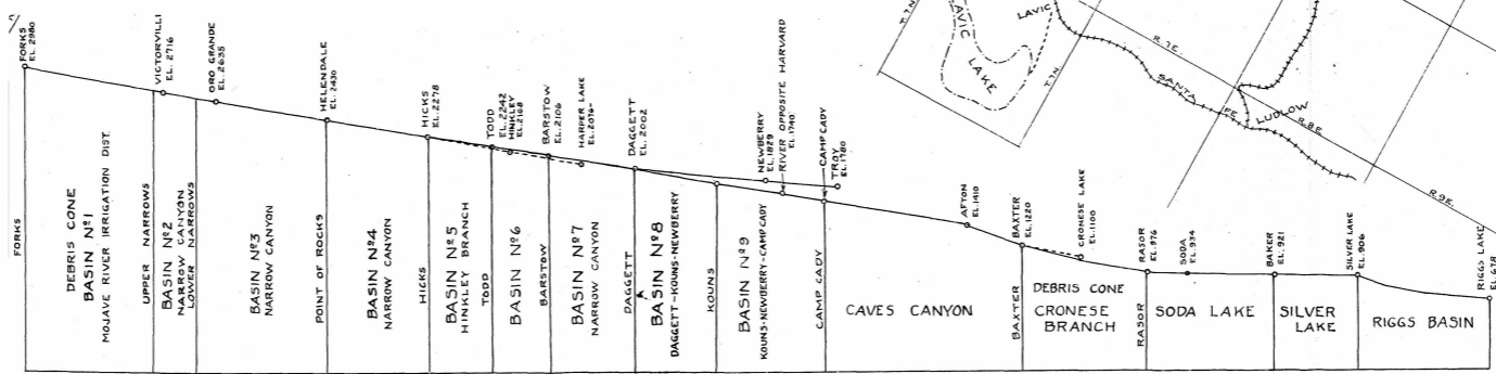
PROFILE OF MOJAVE RIVER FROM RAILROAD ELEVATIONS VERTICAL SCALE 1" = 1000' HORIZONTAL SCALE 1" = 10 MILES
