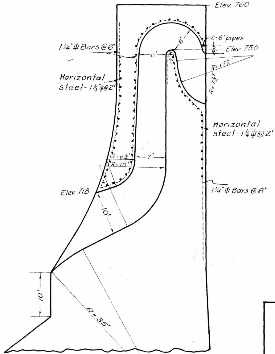
SECTION THROUGH SIPHON
