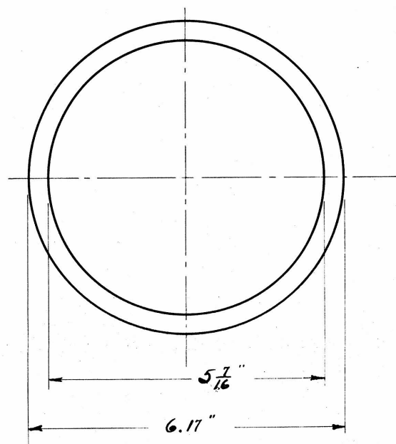
CLAMPING RING 2-REQUIRED MATERIAL STEEL OR W.I.
