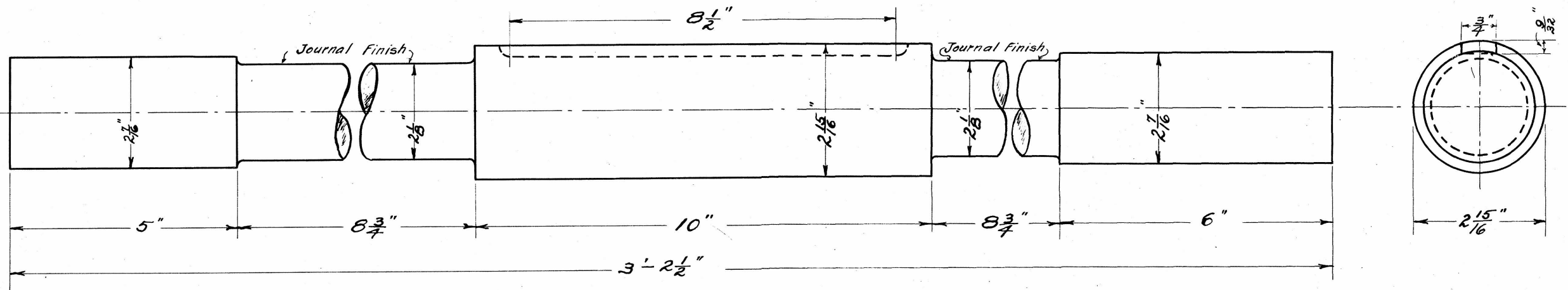
SHAFT 1-REQUIRED MATERIAL STEEL
