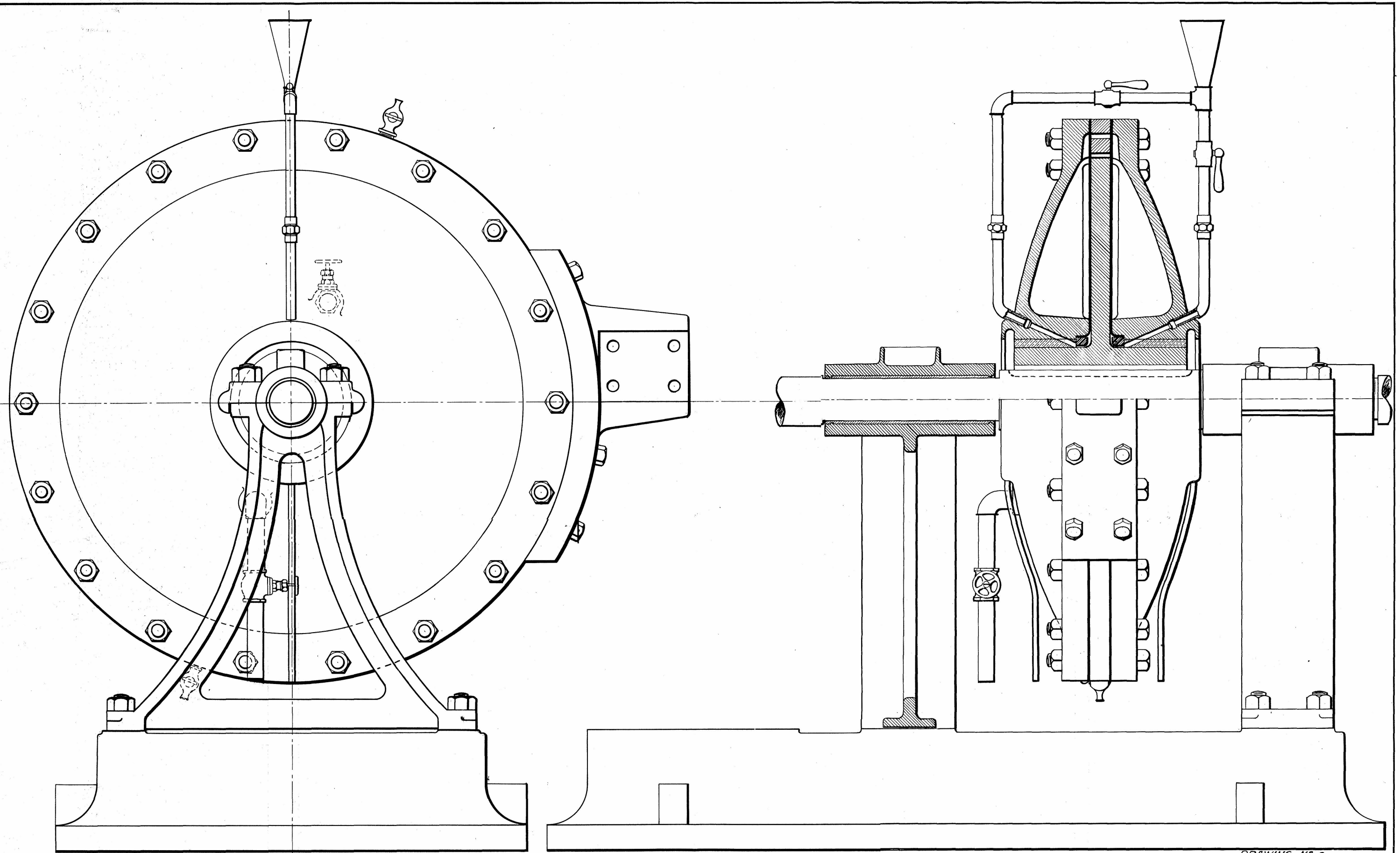
DRAWING N o 8 ASSEMBLY ALDEN BRAKE THROOP COLLEGE OF TECHNOLOGY Pasadena California Scale \frac{3}{8} "-1" Feb. 1914. Drawn and traced by H. Gerckens
