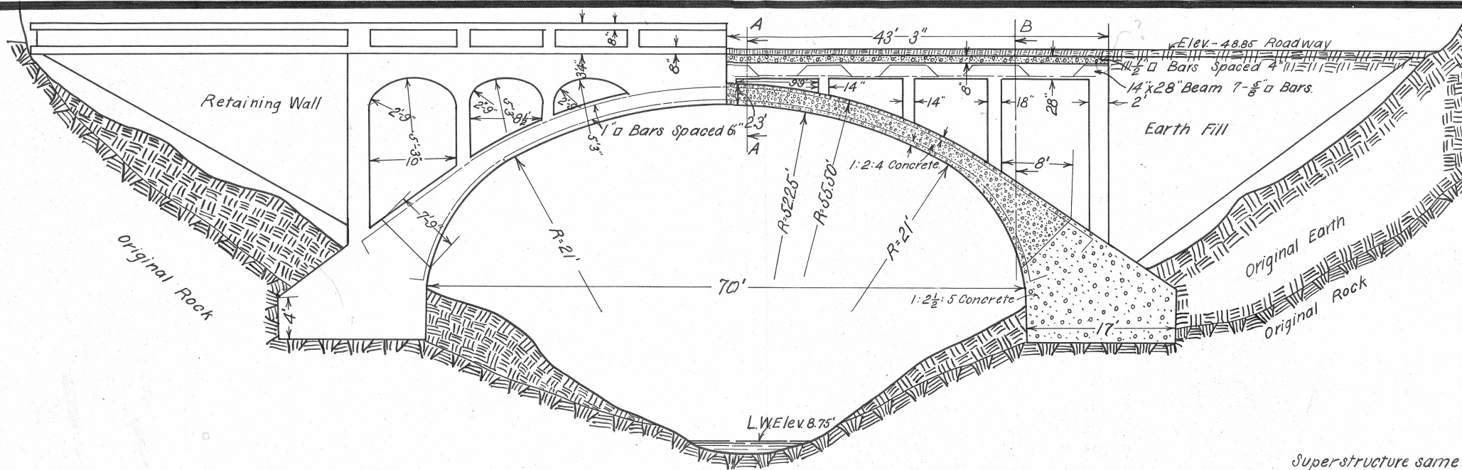
ELEVATION LOOKING DOWN STREAM
