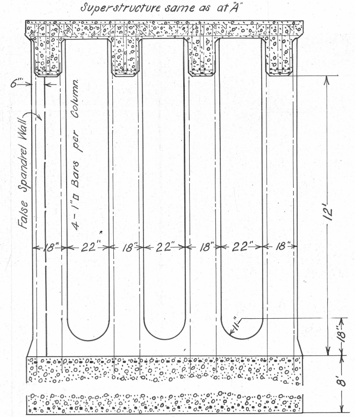
SECTION AT "B"
