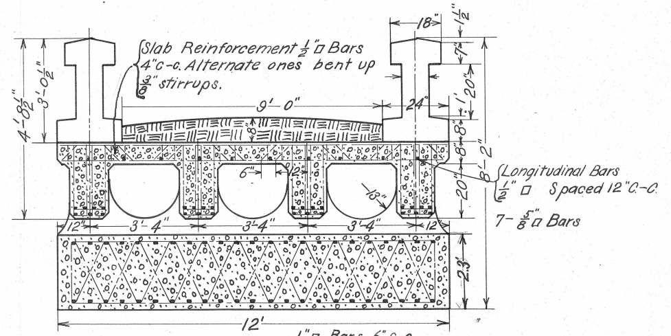
SECTION AT "A."
