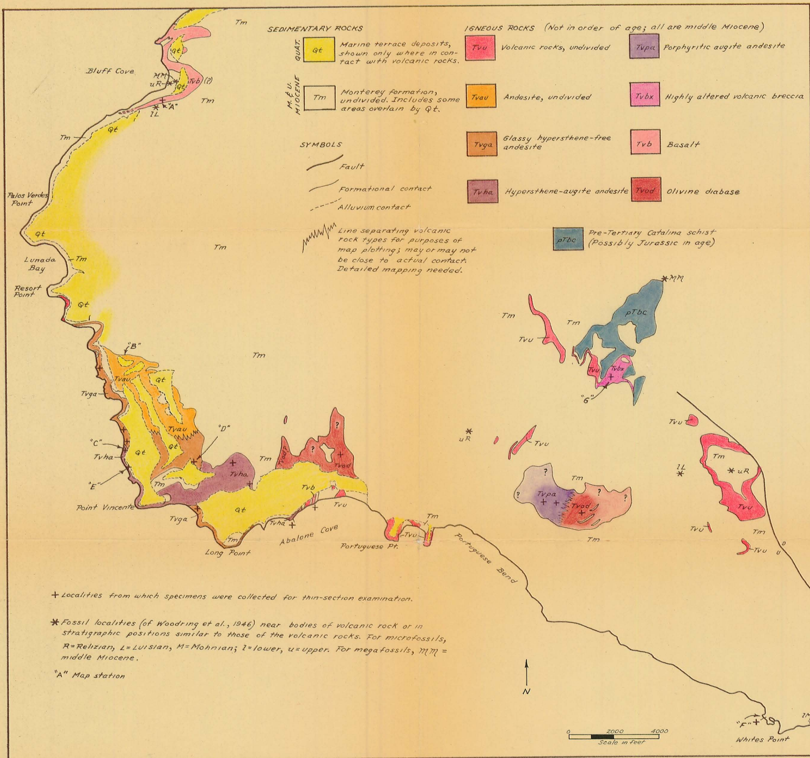
PLATE IV. SKETCH GEOLOGIC MAP OF THE MIOCENE VOLCANIC ROCKS IN THE PALOS VERDES HILLS, CALIF. Distribution of Qt, Tm, and volcanic rocks, as an undivided group, from Woodring et al. (1946)
