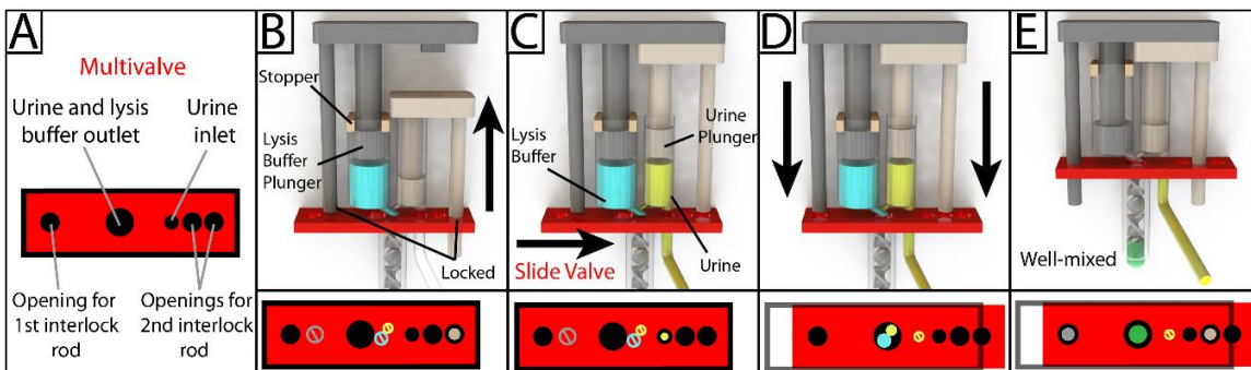
Figure 1.1: Schematic overview of the design and operation of the 3D-printed interlock meter-mix device for metering and mixing a urine sample with lysis buffer.
