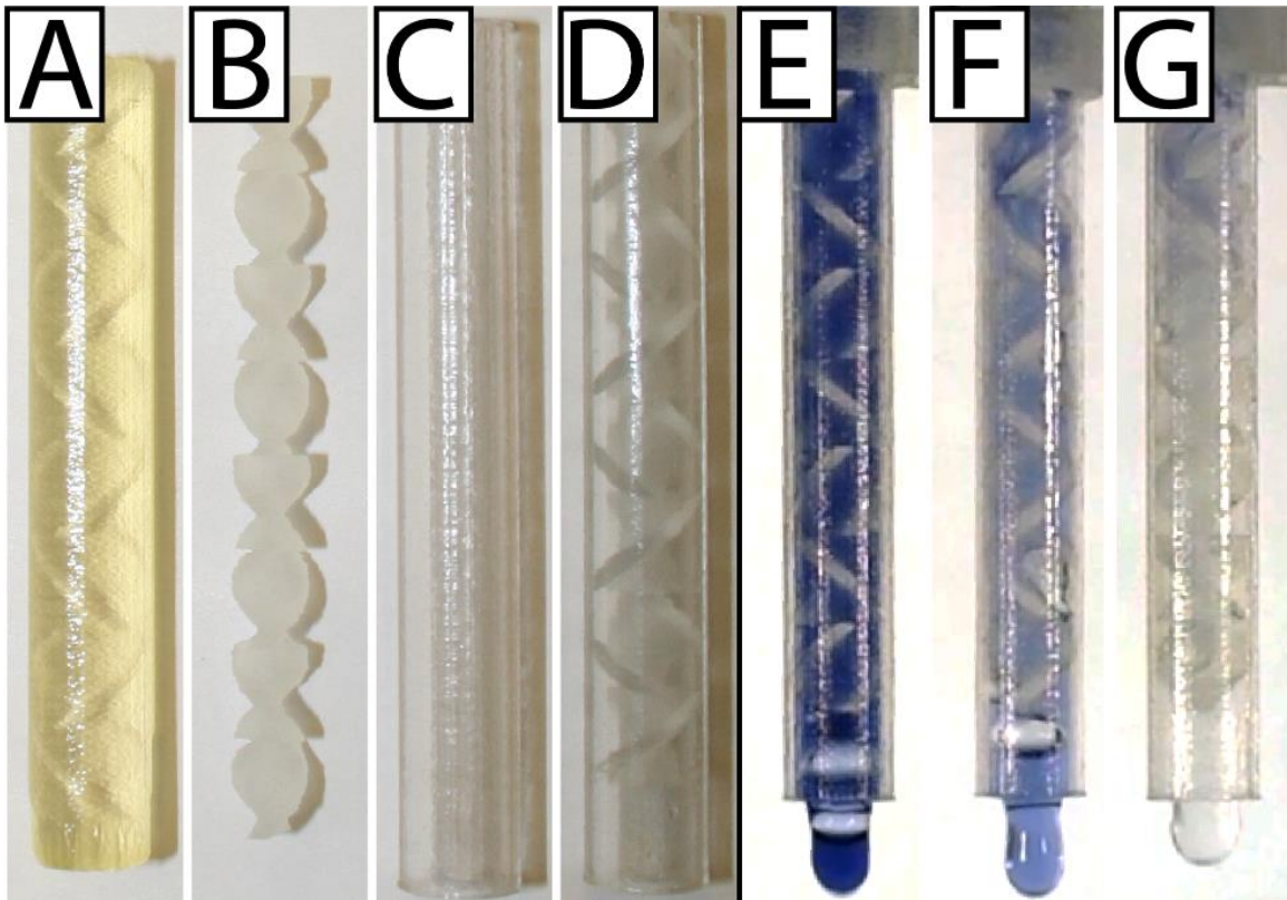
Figure 1.3: Assembly of the static mixer (A–D) and a demonstration of its use in the meter-mix device (E–G).
