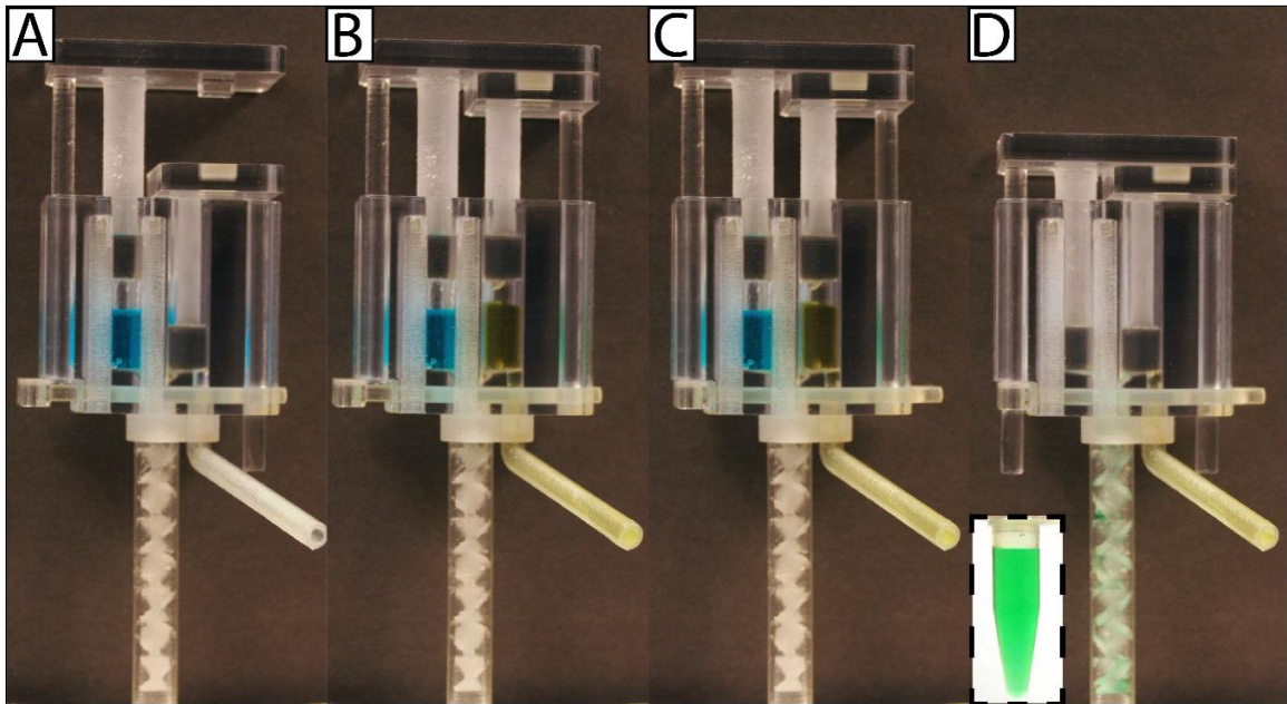
Figure 1.2: Photographs of the device at different stages of operation.
