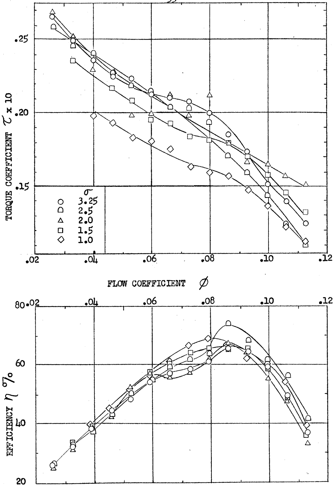
FIG. 10 TORQUE COEFFICIENT AND IMPELLER EFFICIENCY WITH VARYING SOLIDITY, \lambda = 0.15 EXCEPT FOR \sigma = 2.5 ( \lambda = 0.1375 )
