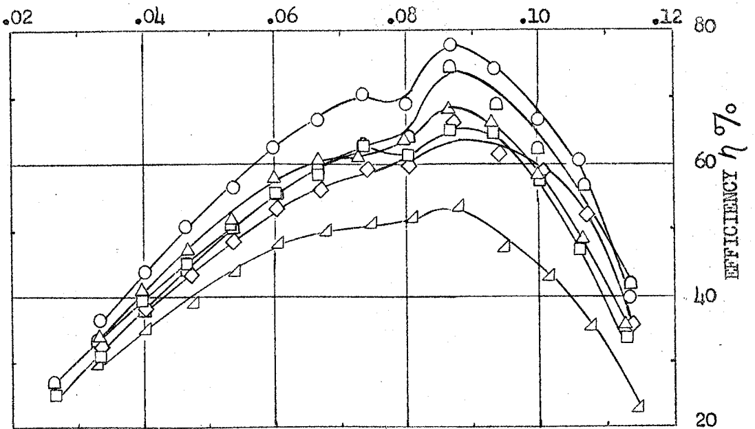
FIG. 7 TIP CLEARANCE EFFECT ON TORQUE COEFFICIENT AND EFFICIENCY
