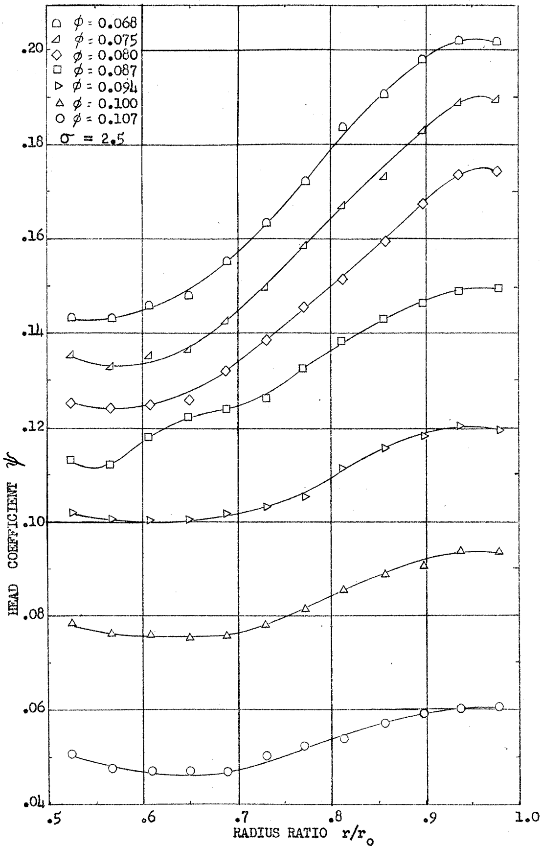
FIG. 11. RADIAL HEAD DISTRIBUTION - TYPICAL IMPELLER ( \lambda = 0.0375 )
