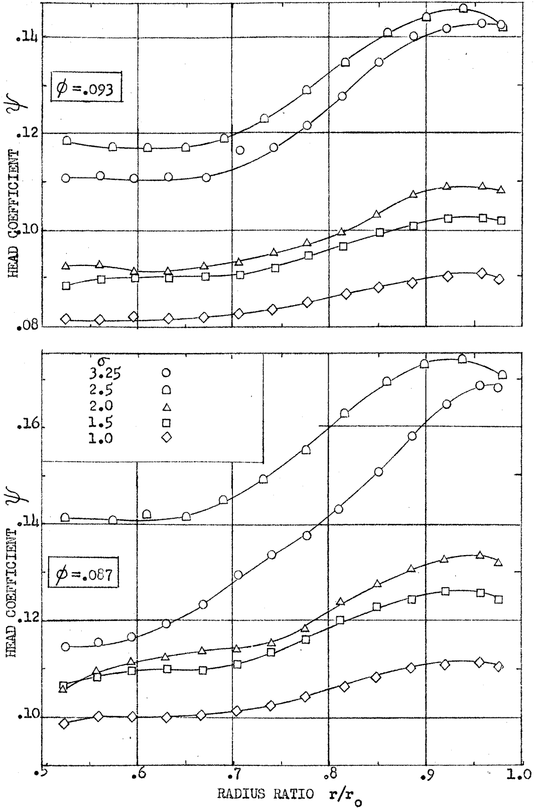
FIG. 16 EFFECT OF SOLIDITY ON RADIAL HEAD DISTRIBUTION \lambda = 0.15 EXCEPT FOR \sigma = 2.5 ( \lambda = 0.1375 )
