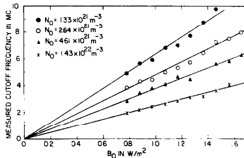
Fig. 5. Cutoff frequency vs magnetic field strength.
