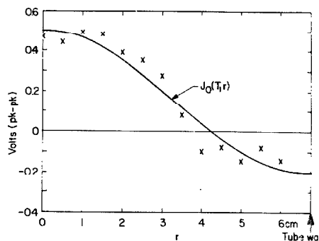
FIG. 11. Radial amplitude variation.
