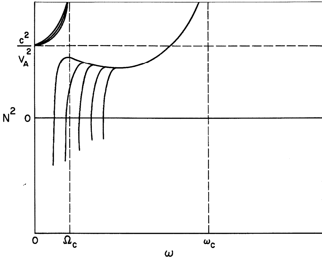
Figure 1.3 Dispersion Relation for the Hydro-magnetic Waveguide
