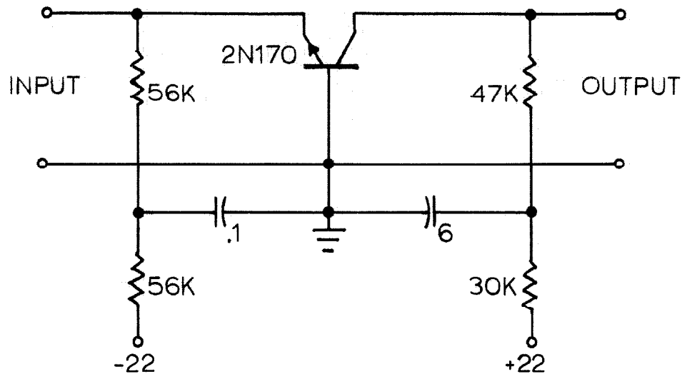
Figure 3.9 Photomultiplier Amplifier
