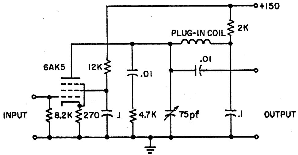
Fig. 3.4 Typical Stage of the R.F. Amplifier
