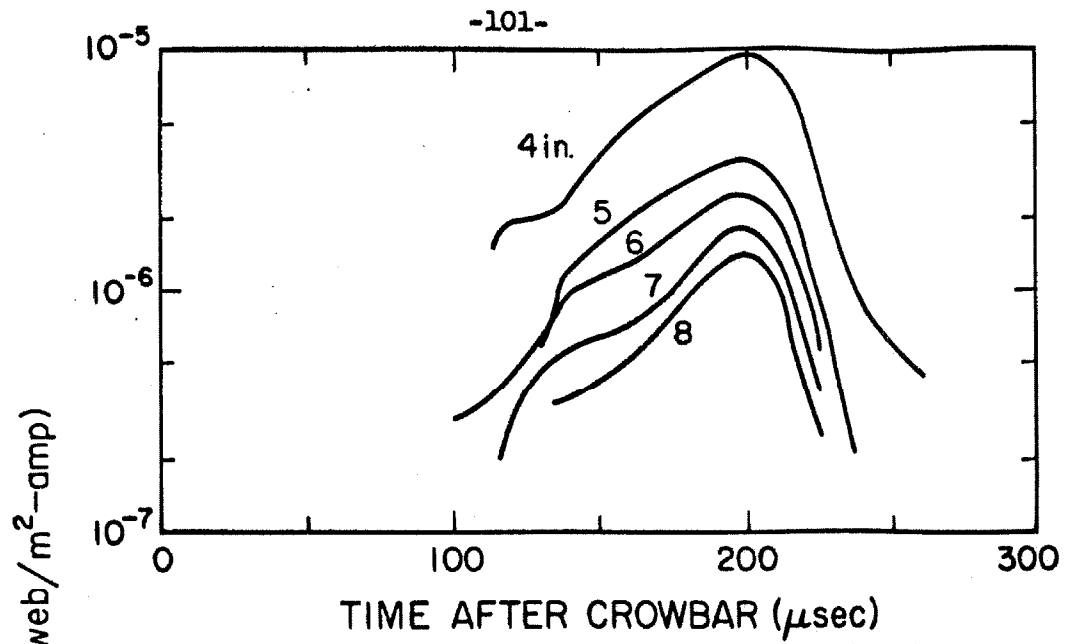
Fig. 4.16 Normalized Amplitude Curves at 15 Mc
