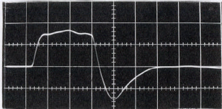
Fig. 3.2 Ionizing Current Vertical Scale - approximately 10 4 amp per large division Horizontal Scale - 10 μsec per large division
