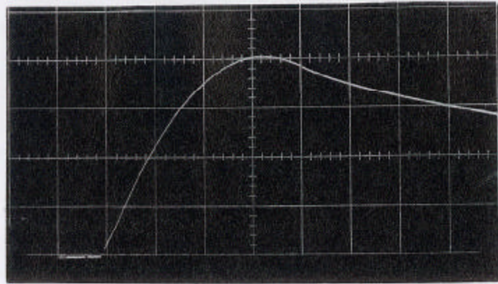
Fig. 3.1 Axial Magnetic Field at 1 kv Bank Voltage. Vertical Scale - 0.5 web/m 2 per large division Horizontal Scale - 200 μsec per large division
