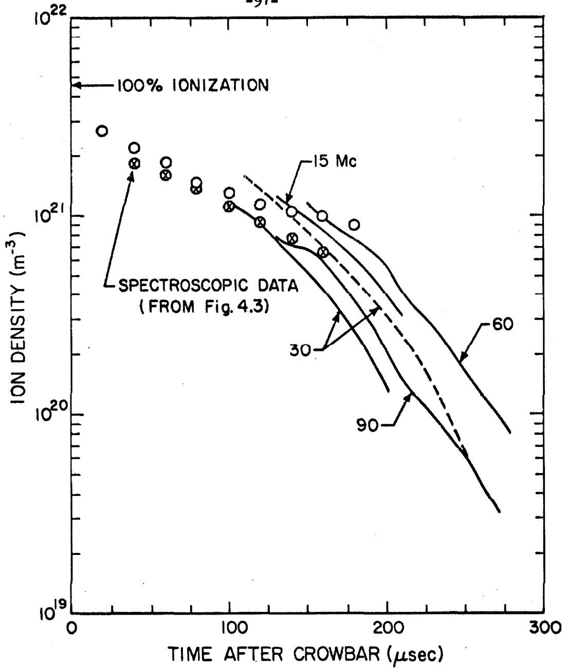
Fig. 4.14 Density Decay Curves
