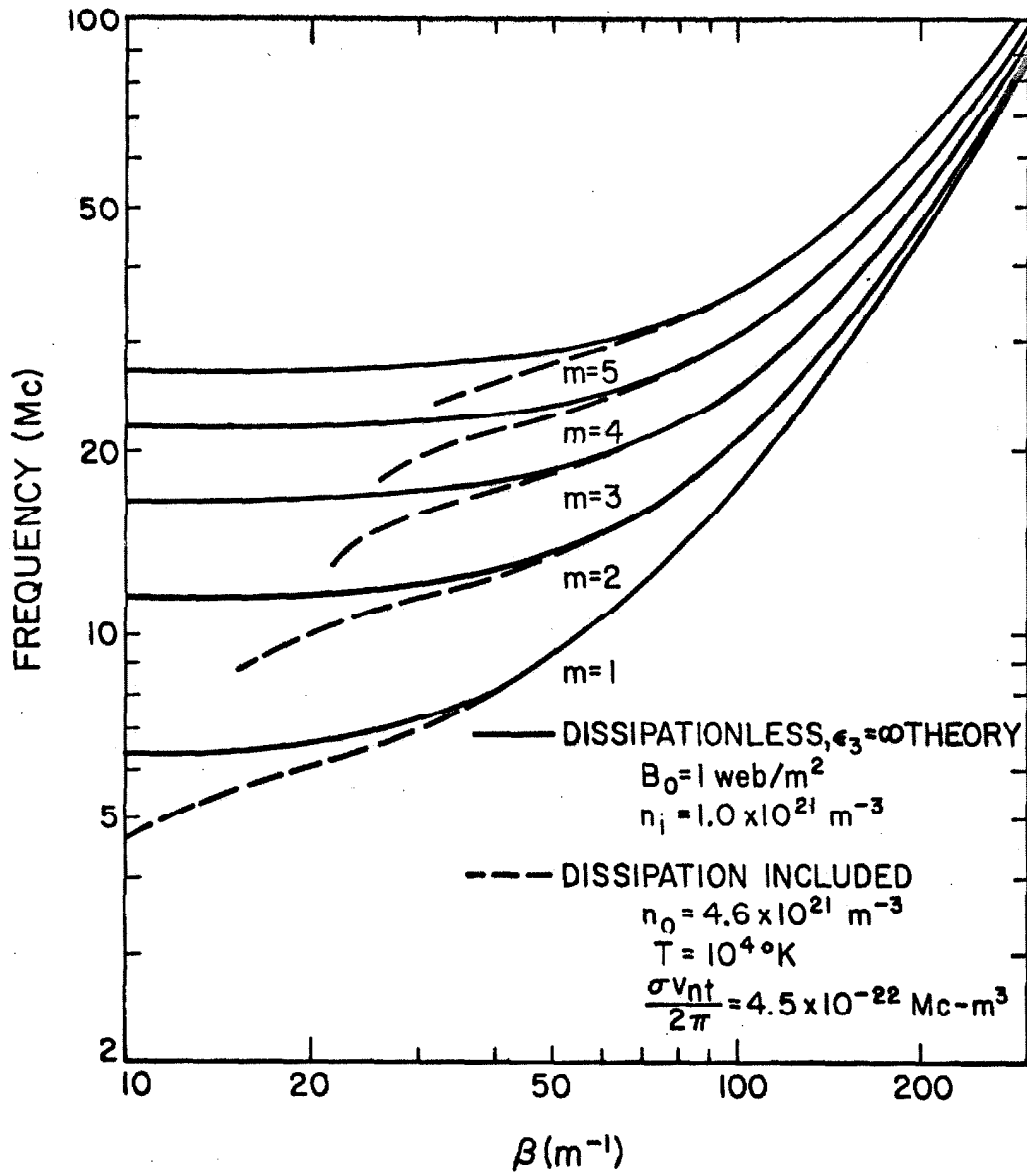
Fig. 2.2 Phase Factors for the First Five Circularly-Symmetric Compressional Modes
