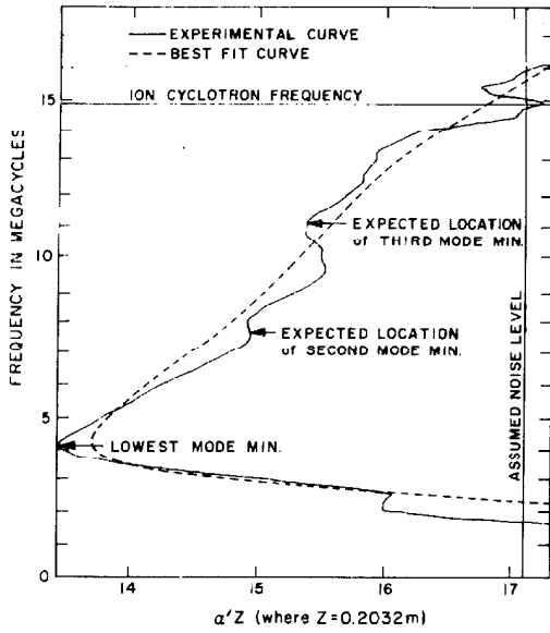
Fig. 8. Frequency vs transfer function effective attenuation constant.
