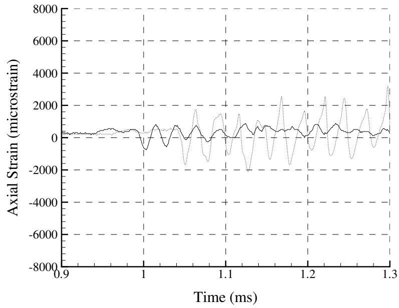
Figure A.150: Shot 137 axial strain.
