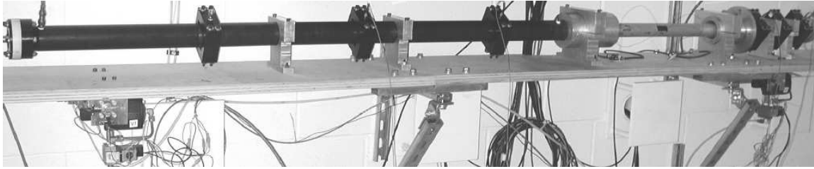
Figure 4.7: Second tube assembly with 0.610-m long specimen and a 0.305 m extension tube.
