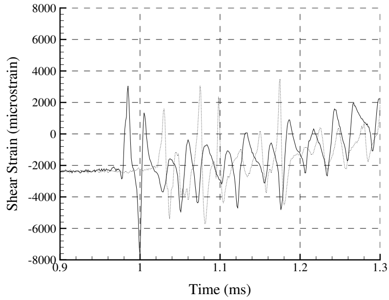
Figure A.169: Shot 149 shear strain.
