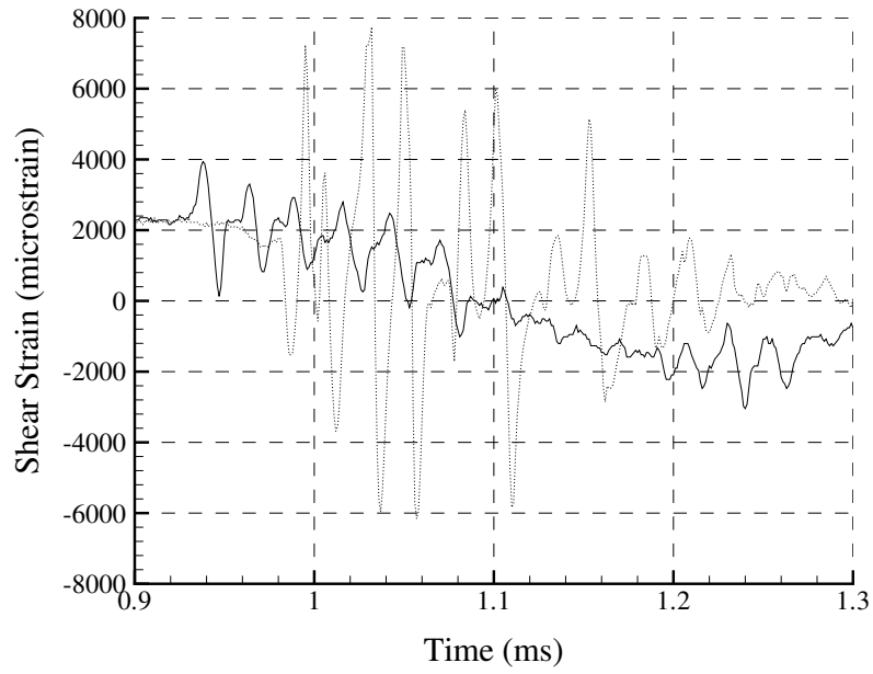
Figure A.173: Shot 151 shear strain.
