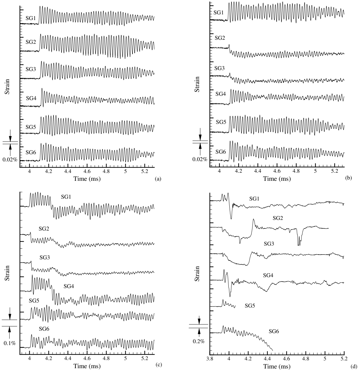
Figure 4.16: Hoop strain of four specimens with the same wall thickness and tube length but different CJ detonation pressure. The flaw sizes were also the same, except Shot 33, which had no notch. All strain traces start at zero strain. (a) Tube with no notch and no rupture (Shot 33). (b) Notched tube with no rupture (Shot 31). (c) Notched tube with rupture confined within the notch (Shot 30). (d) Notched and ruptured tube with forward and backward helical cracks (Shot 34).
