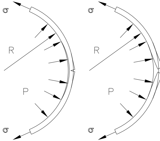
Figure 4.20: Bulging of the regions near the notch and the cracks caused the local shell curvature to change and thus, gave rise to local compressive strains recorded by strain gages. The compression is not unlike the one experienced by one side of a cantilever beam under distributed load.
