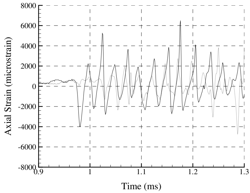
Figure A.170: Shot 149 axial strain.
