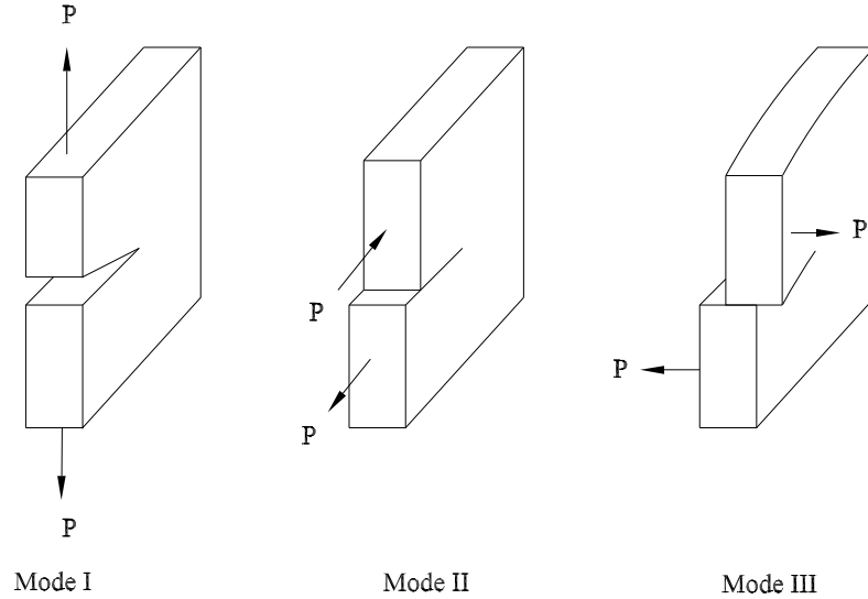
Figure 1.6: Fracture modes.
