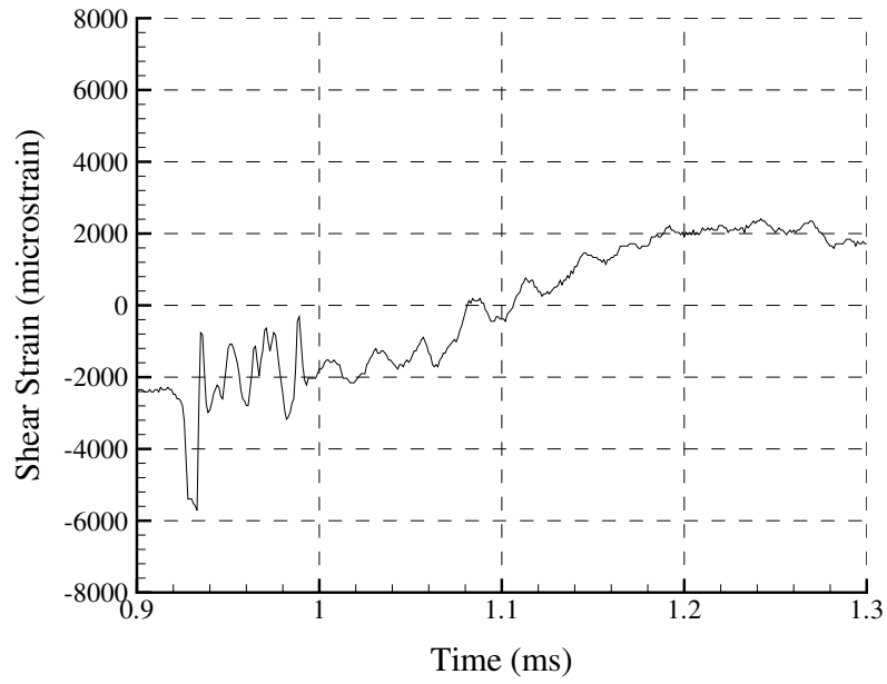
Figure A.161: Shot 145 shear strain.
