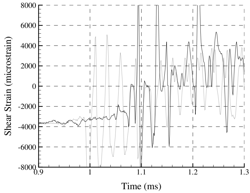
Figure A.177: Shot 153 shear strain.
