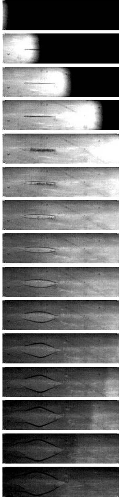
Figure 7.1: Polycarbonate specimen with an initial axial flaw rupturing under gaseous detonation loading. Interframe time is 31\ \mu\text{s} .
