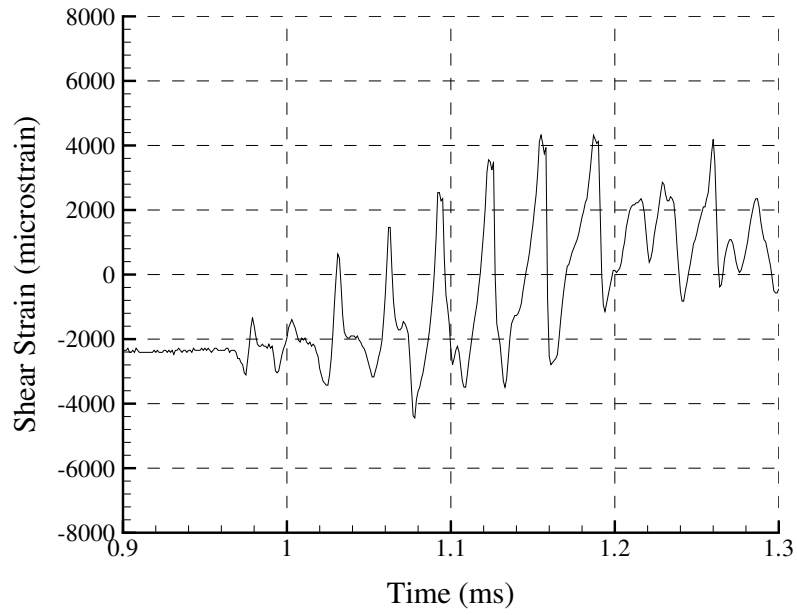
Figure A.165: Shot 147 shear strain.
