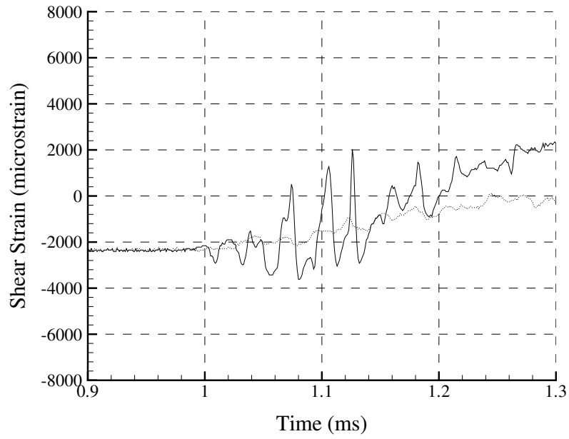
Figure A.149: Shot 137 shear strain.
